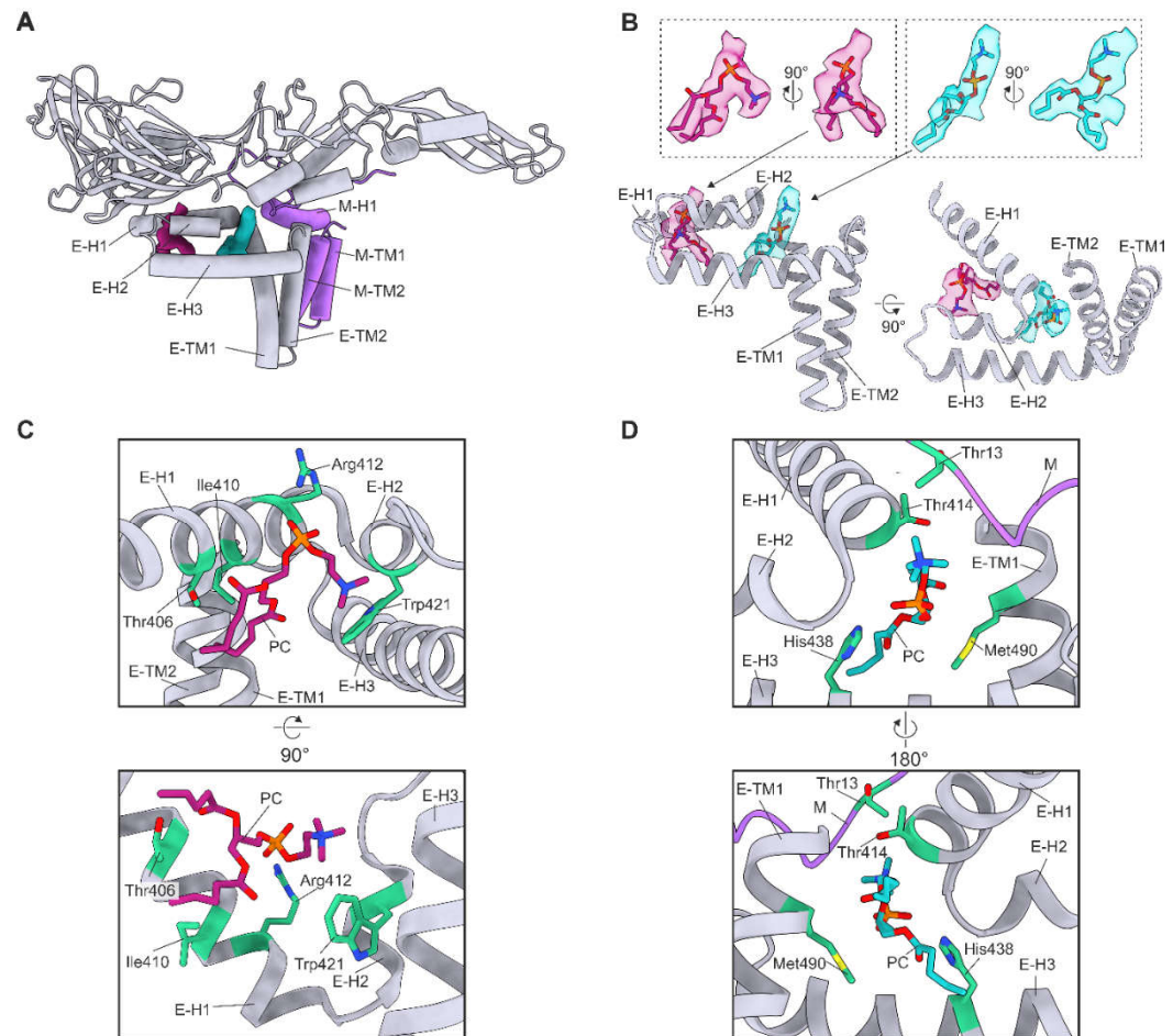
Figure 5 Ordered phosphatidylcholine (PC). (a) Two PC molecules bound per heterodimer. (b) Location of the lipid factors in relation to the E protein Domain IV. The PC atomic models are coloured in magenta (PC 1) and turquoise (PC 2) with oxygen, nitrogen, and phosphorus atoms coloured in blood red, blue, and orange, respectively. (a, b) The E chain C is coloured in grey, and M chain D is coloured in purple. The densities corresponding to PC 1 and PC 2 are coloured in magenta and turquoise, respectively. The transmembrane (TM) and perimembrane (H) helices of E and M are labelled. (c) Residues within 4 Å of PC 1. (d) Residues within 4 Å of PC 2. M protein is coloured in purple. (c, d) Residues within 4 Å of PC 1 are shown, labelled, and coloured in green.
