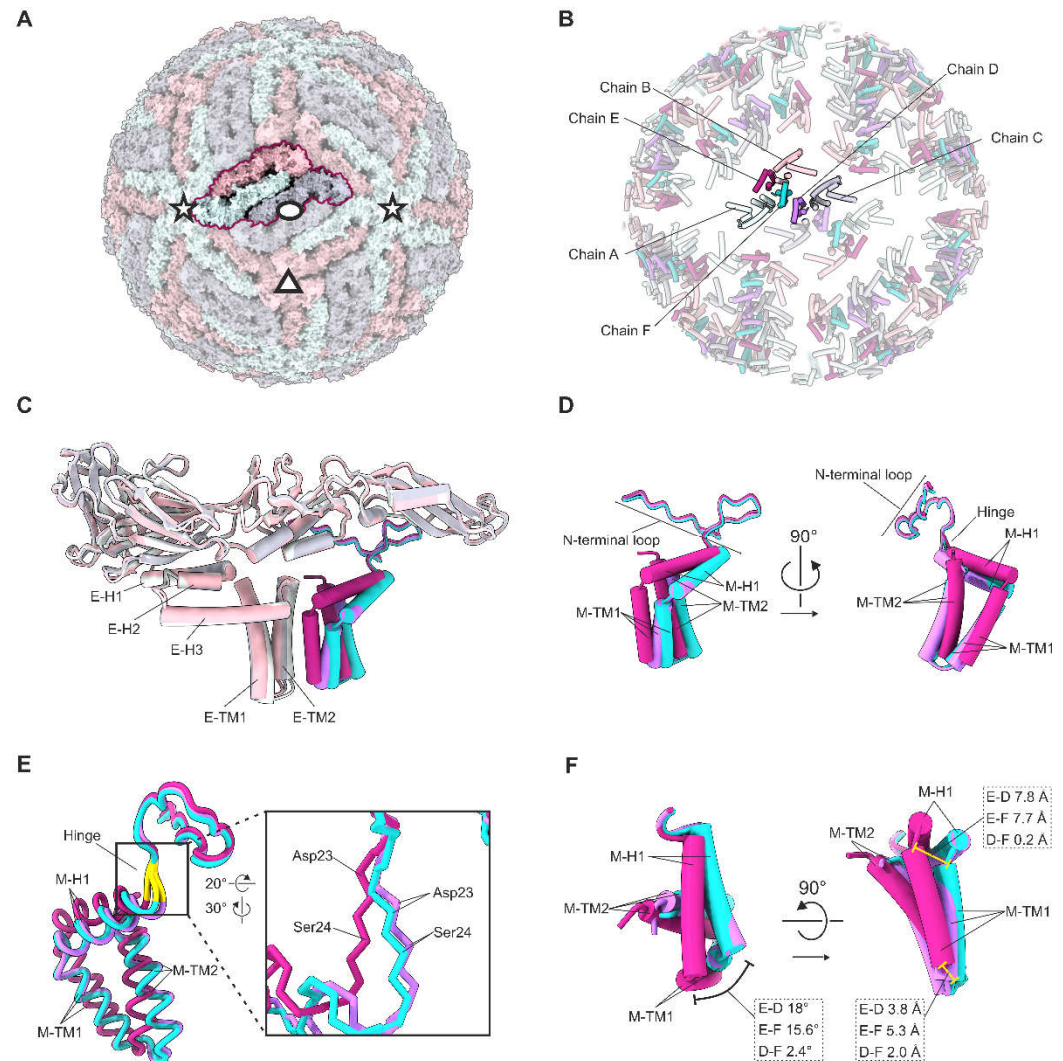
Figure 2 Quasi-equivalence within the asymmetric unit. (a) Surface representation of the TBEV virion. One asymmetric unit is highlighted. The symmetry axes are indicated with an ellipse (two-fold), a triangle (three-fold), and stars (five-fold). (a-c) The three E proteins forming the asymmetric unit are coloured in light green (chain A around the five-fold axes of symmetry), pink (chain B around the three-folds), and grey (chain C around the two-folds). (b) Cartoon representation of the E and M membrane associated domains within the context of a virion. (b-f) The three M proteins within one asymmetric unit are coloured in purple (chain D), magenta (chain E), and turquoise (chain F). (c) Superimposition of the three E-M heterodimers that make up the asymmetric unit, based on the E proteins. Transmembrane helices of E are labelled as E-TM1, and E-TM2; perimembrane helices are labelled E-H1, E-H2, and E-H3. (d) Detailed view of the superimposed M proteins of one asymmetric unit. Transmembrane helices of M are labelled as M-TM1, and M-TM2; perimembrane helix is labelled M-H1; N-terminal loop and hinge are indicated. (e) Superimposition of the three M proteins in one asymmetric unit as in (c). The hinge between M-H1 and the N-terminal loop is highlighted in yellow and is shown zoomed in. The differences in the backbone positions at residues 23 and 24 are indicated. (f) Superimposition of the three M proteins in one asymmetric unit as in (c) with the N-terminal residues 1-21 hidden for clarity. The angles between the superimposed helices are shown in the top view (left), and the distances between the corresponding Cα atoms are indicated in the side view (right).
