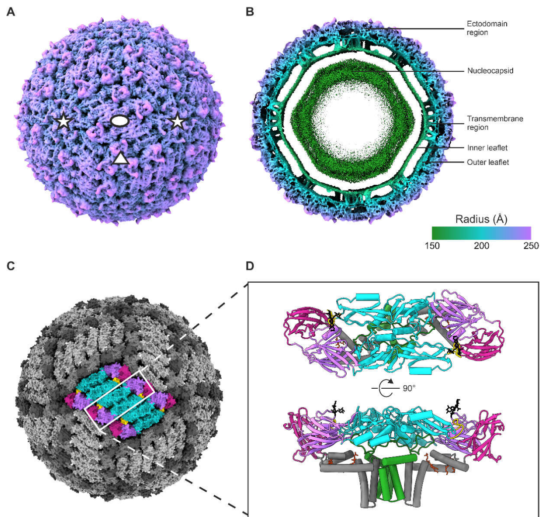
Figure 1. TBE virion cryoEM reconstruction and atomic model. (a) Radially-coloured isosurface representation of the reconstruction viewed down a two-fold axis of symmetry, shown at 2.35 \sigma above the mean. The symmetry axes are indicated with an ellipse (two-fold), a triangle (three-fold), and star (five-fold). The colour key is the same as in panel B. (b) A 60-Å central slice of a radially-coloured isosurface representation of the reconstruction viewed down a two-fold axis of symmetry, at 2.35 \sigma above the mean. (c) Surface representation of the reconstruction, with a raft of three E-M-M-E heterotetramers highlighted, viewed down a two-fold axis of symmetry. (d) Cartoon representation of the E-M-M-E heterotetramer shown from the top and side views. (c and d) The E domains are coloured in purple (domain I), turquoise (domain II), magenta (domain III), grey (domain IV), the E fusion loop is coloured in gold, the E Asn154 glycan motif in black, the M protein in green, and the phosphatidylcholine (PC) lipids in red-orange.
