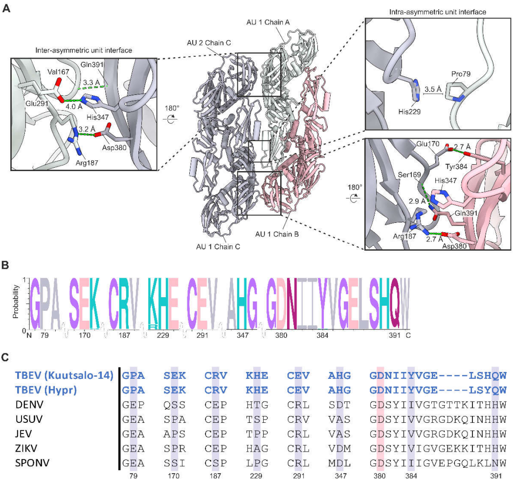
Figure 4 Interactions at the E heterotetramer interface. (a) Interactions between the E proteins located at the heterotetramer interface. Chain B is shown in pink, chain A in light green and chain C in grey. The asymmetric units (AU) are labelled. Interacting residues are shown as stick representations and labelled in the close-up views. Hydrogen bonds are shown by green dotted lines. The distance between the interacting residues is labelled. The \pi -stacking interaction between His347 and Arg187 and the salt bridge between Arg187 (atom-NE) and Asp380 are not shown for clarity. His347 and Arg187 are separated by a distance of 3.4 Å, and Arg187 (atom-NE) and Asp380 by 4 Å. (b) A consensus sequence of the interacting E residues in 183 TBEV sequences.. Letter size is proportional to the frequency of the residue. Interacting residues are marked with numbers and
