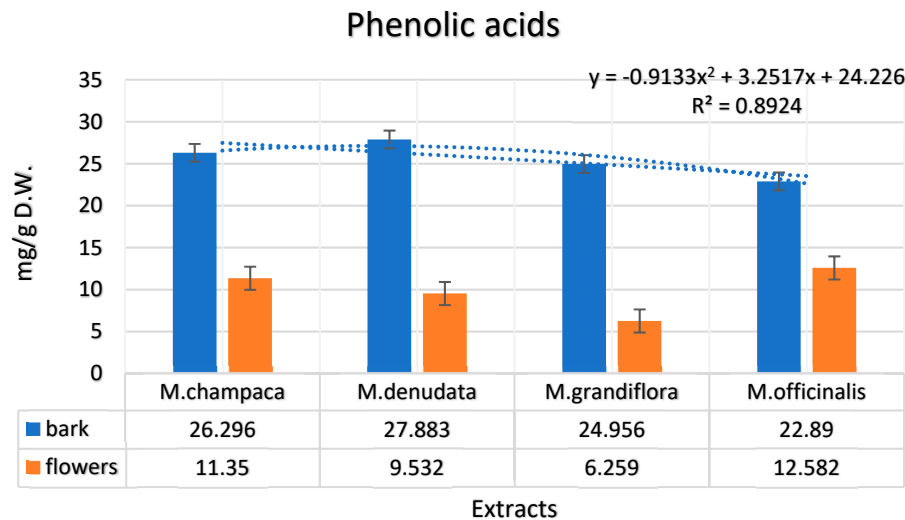
Figure 1. Assessment of phenolic acids in hydroethanolic extracts from the bark and flowers of Magnolia ( M. champaca , M. denudata , M. grandiflora , M. officinalis ).
