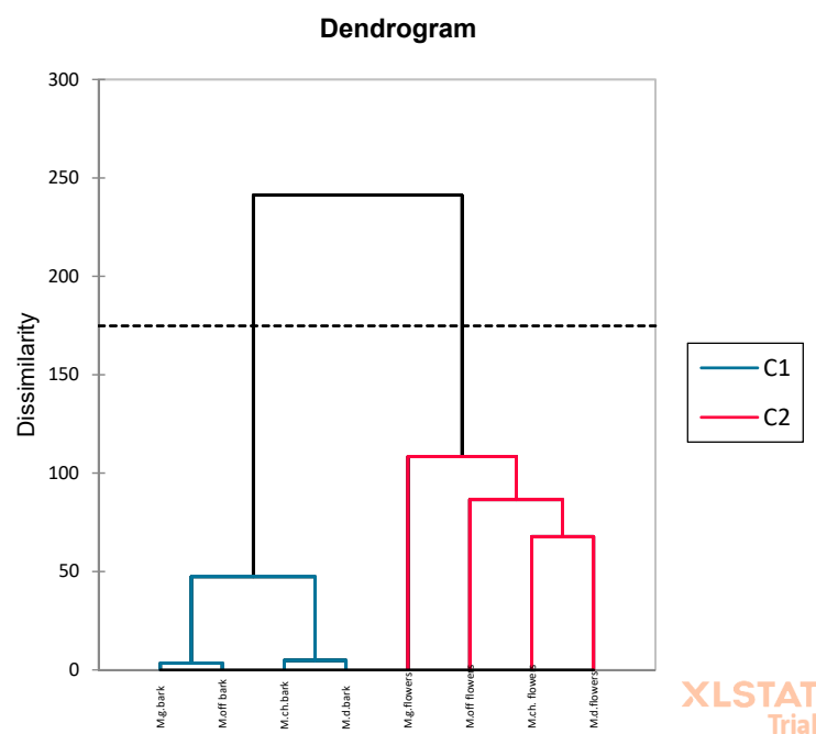
Figure 6. Cluster distribution of bark and flower extracts from four Magnolia species ( M. champaca , M. denudata , M. grandiflora , M. officinalis ).
