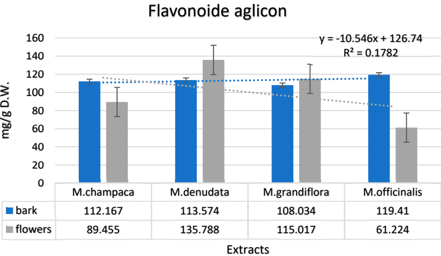
Figure 2. Assessment of aglycone flavonoids in hydroethanolic extracts from the bark and flowers of Magnolia ( M. champaca , M. denudata , M. grandiflora , M. officinalis ).
