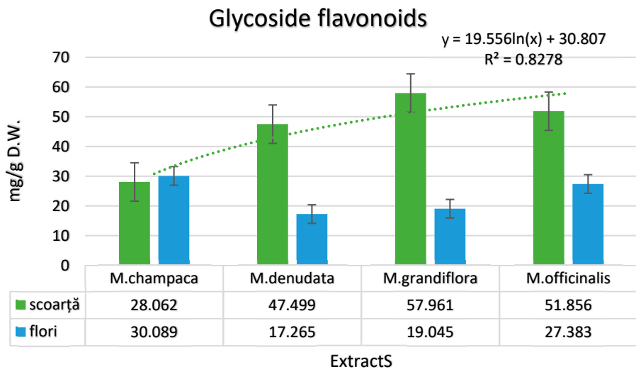
Figure 3. Assessment glycoside flavonoids in hydroethanolic extracts from both the bark and flowers of Magnolia ( M. champaca , M. denudata , M. grandiflora , M. officinalis ).
