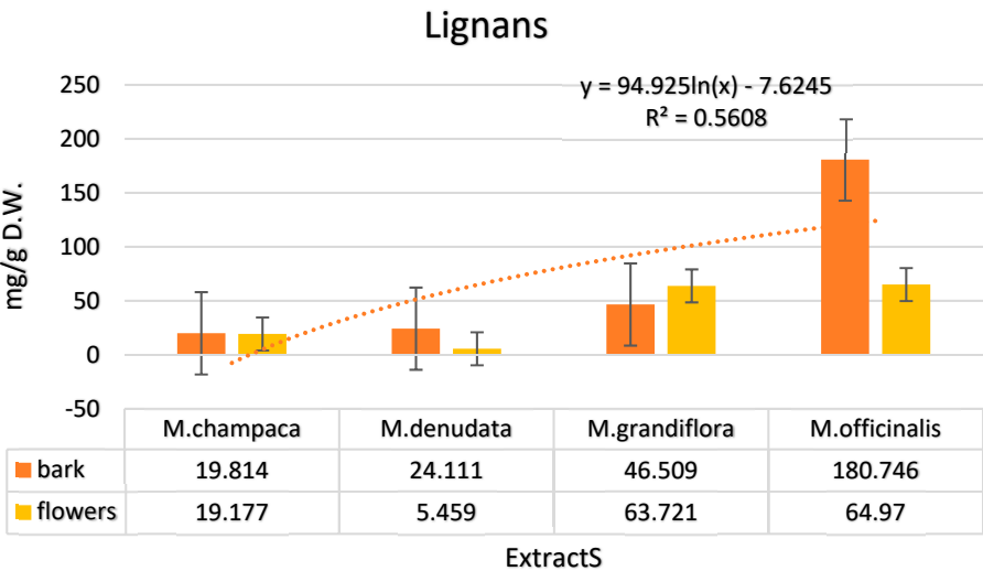
Figure 4. Assessment of lignans in hydroethanolic extracts from the bark and flowers of Magnolia ( M. champaca , M. denudata , M. grandiflora , M. officinalis ).
