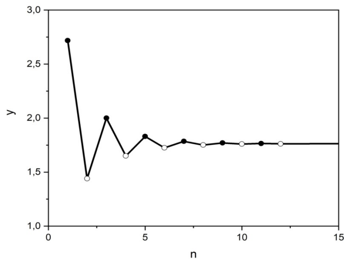
Figure 1. Graph (–) of the oscillating sequence y_n in the algorithm (4) for q = 1 : y^{l_{2n-1}} (●) and y^{l_{2n}} (○) with the same limit value y^{l_{\infty}} = y^{l_{\infty}} = y_{\infty}(1) = 1.7632...
