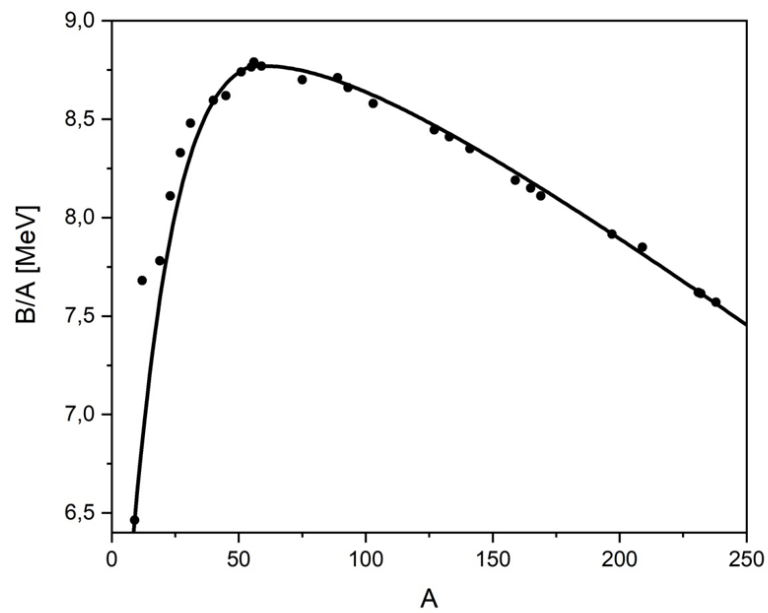
Figure 4. Binding energy/nucleon (MeV) as function of the nucleon number A . (●) experimental values; (—) calculated values with Equation (28).
