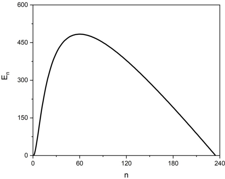
Figure 3. The interaction function E_n from Equation (27) versus the number n of nucleons.
