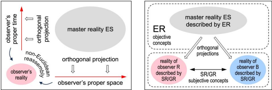
FIG. 1. Observer’s reality and master reality ES (for orthogonal projections, see Sect. 4). Left: How to relate an observer’s reality to ES. Right: Where to apply SR/GR and where to apply ER.
