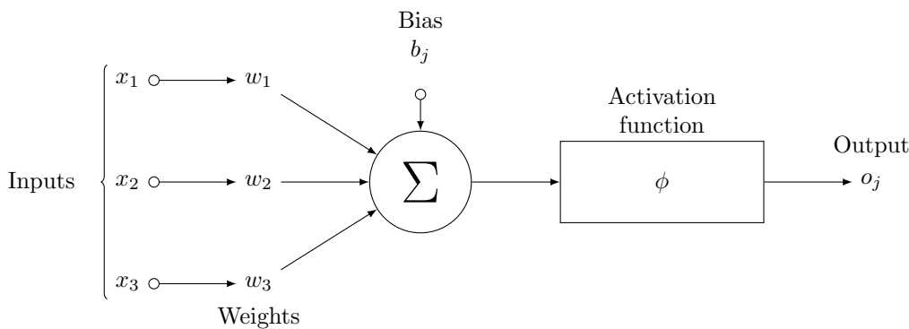
Figure 2. A schematic representation of of a perceptron model. A weighted sum of the inputs ( \Sigma ) is passed through an activation function ( \phi ) to get the output ( o_j ).
