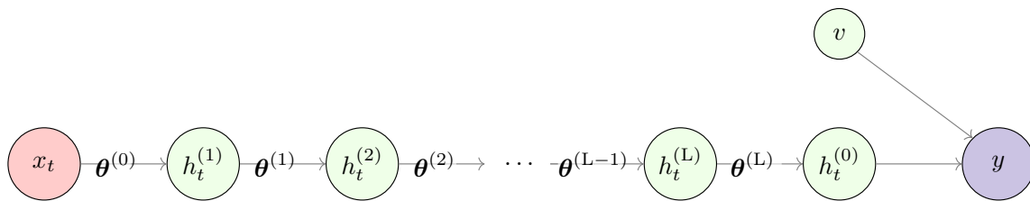
Figure 3. A compact representation of a Feedforward Neural Network (FFNN). For simplicity, we assume x_t, y_t \in \mathbb{R} , and the observation model is given by y = h_t^{(0)} + v , where v \sim \mathcal{N}(0, \sigma_v^2) . The network consists of L hidden layers, each containing A hidden units. For any layer j \in \{1, 2, \dots, L\} , the parameters between layers j and j + 1 are denoted by \theta^{(j)} . Adopted from Deka et al. [100].
