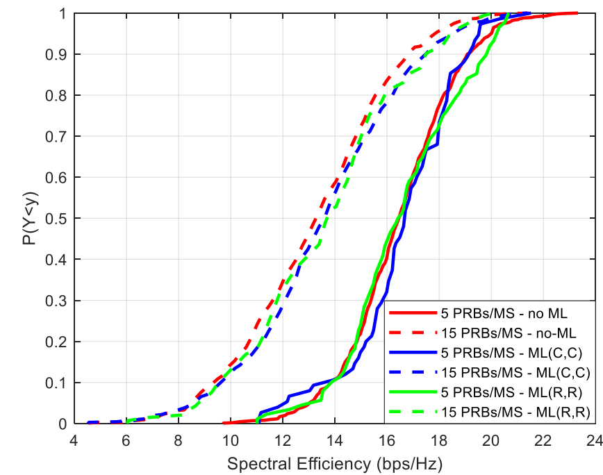
Figure 9. Spectral Efficiency (bps/Hz).
