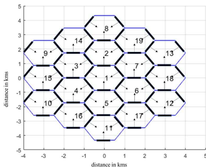
Figure 1. Multicellular mm-Wave m-MIMO orientation.
