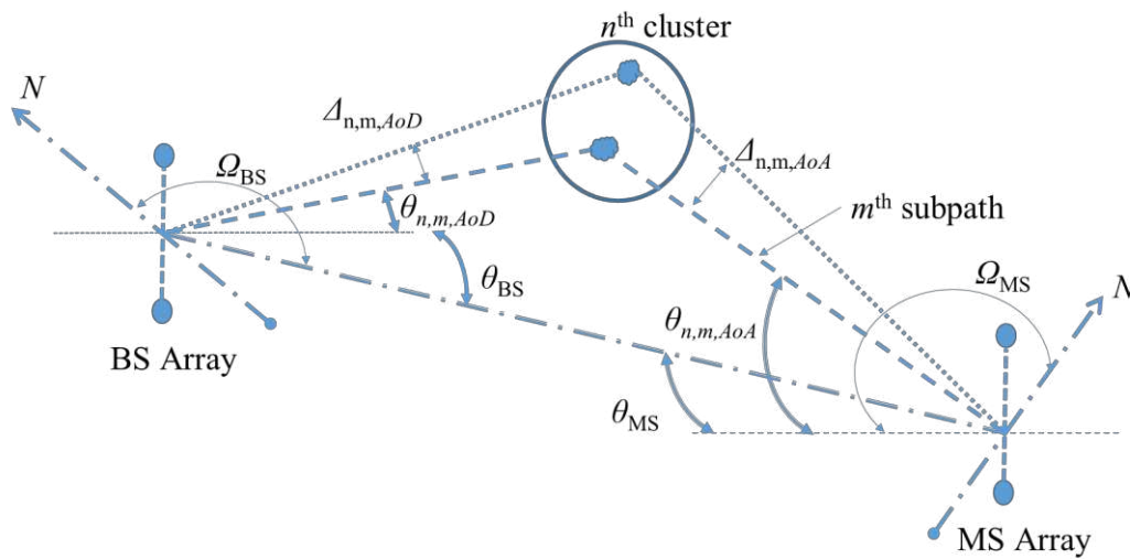
Figure 2. Clusters and subpaths in 3GPP channel modelling.
