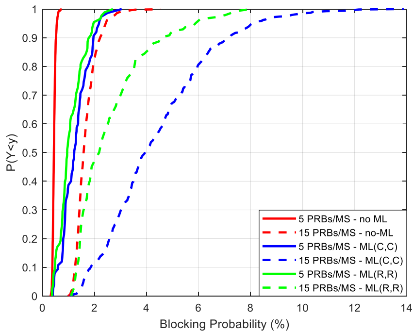
Figure 11. Blocking probability.
