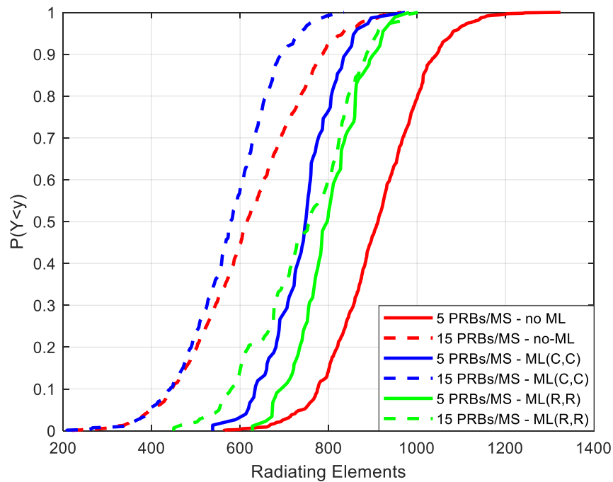
Figure 12. Radiating elements.
