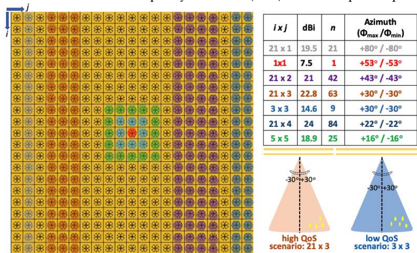
Figure 4. Representative antenna array configurations spotted with colors (left panel) in concert with their corresponding directivity in dBi, number of REs ( n ) and the azimuth coverage in degrees ( \Phi^\circ ).
