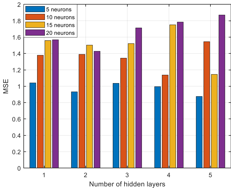
Figure 6. Mean square error for 15 PRBs per MS and SE training.
