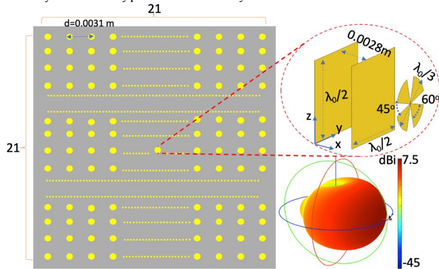
Figure 3. The proposed antenna array scheme of 21×21 REs (left panel) along with the geometry and the radiation pattern of each RE (right panel).
