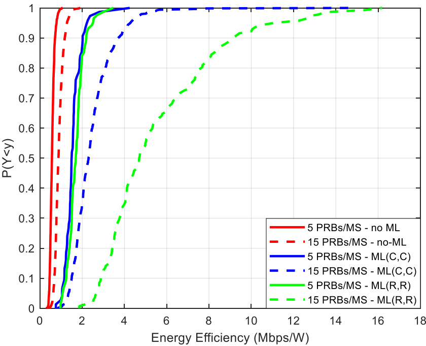
Figure 10. Energy Efficiency (Mbps/W).
