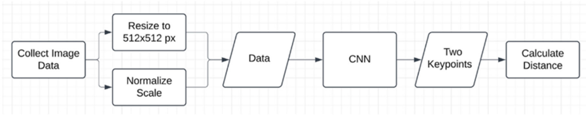
Fig: 3: Flowchart of the CNN keypoint implementation model's process
