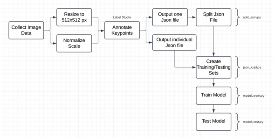
Fig 5: Keypoint implementation model training process
