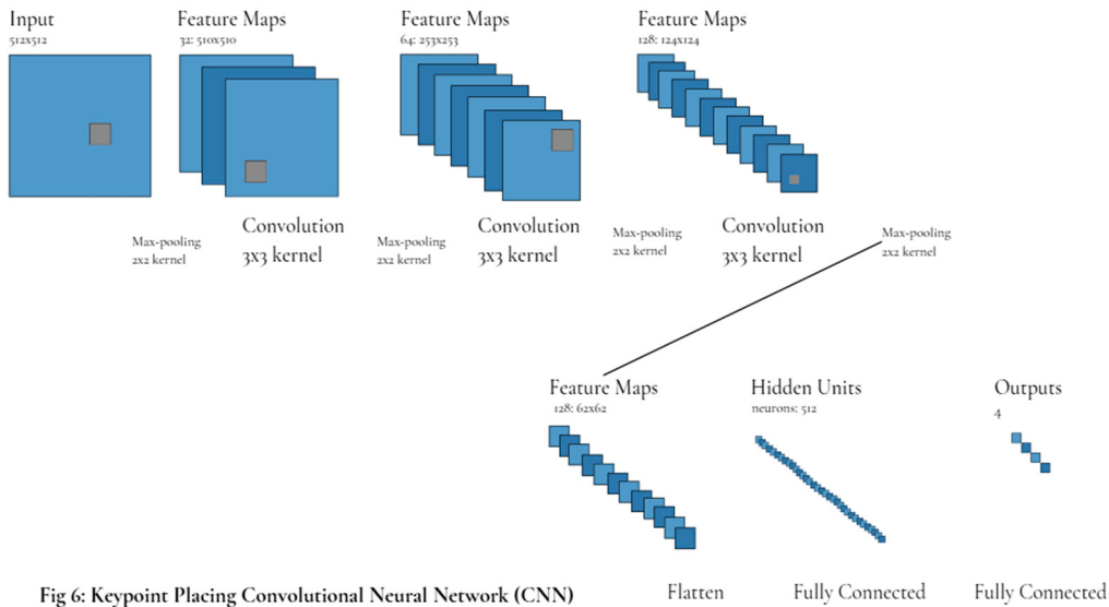
Fig 6: Keypoint Placing Convolutional Neural Network (CNN)
