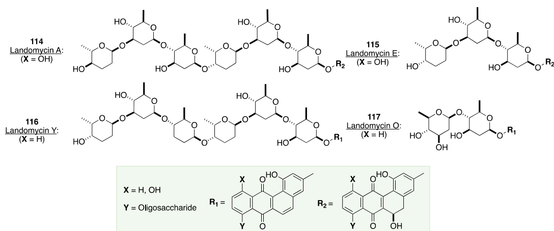
Scheme 18. The landomycin family of oligosaccharides.
