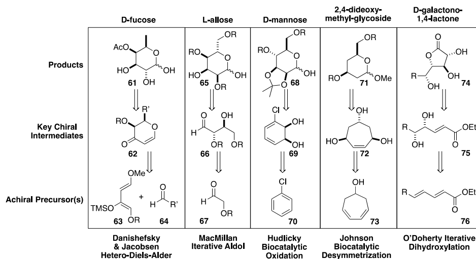
Scheme 12. Other de novo asymmetric synthesis of hexoses.
