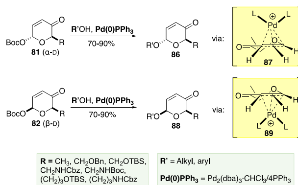
Scheme 14. Diastereoselective Pd-glycosylation.
