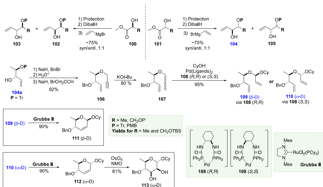
Scheme 17. Rhee asymmetric synthesis of hexoses via a Pd-glycosylation (Pd-allylation/RCM).
