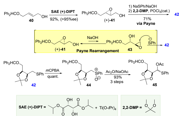
Scheme 9. Sharpless epoxidation/Payne rearrangement for the synthesis of cis-acetonide.
