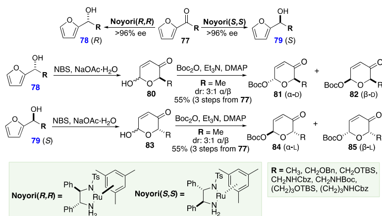
Scheme 13. O'Doherty de novo asymmetric synthesis of pyranone based Pd-glycosylation donors.
