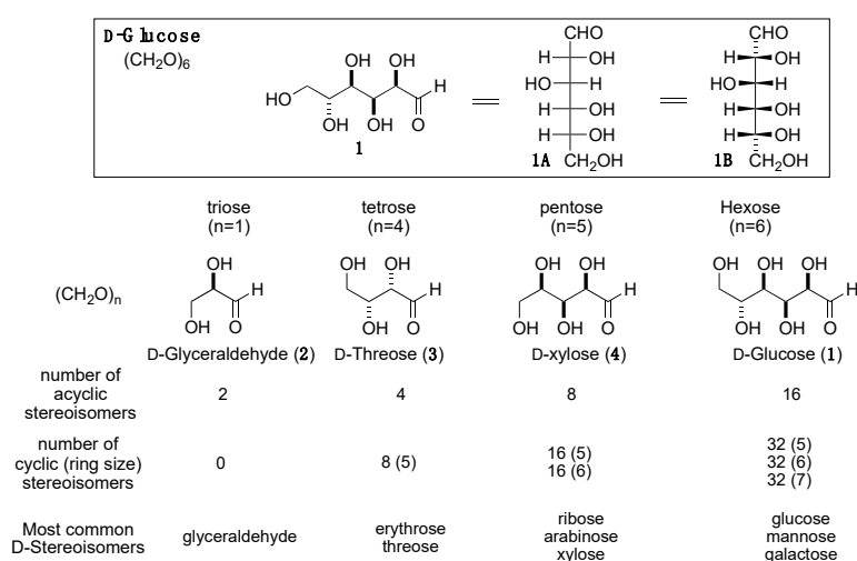
Scheme 1. The monosaccharides and their stereochemical complexity from C-3 to C-6.
