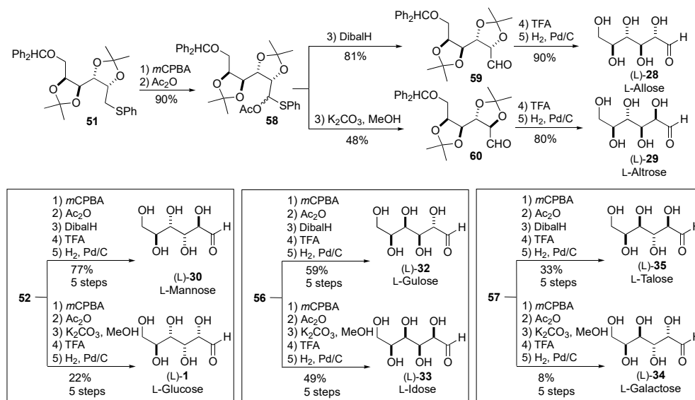
Scheme 11. End game for the Sharpless de novo asymmetric synthesis of the L-hexoses.
