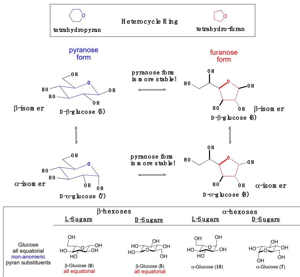
Scheme 2. The cyclic hexoses in their cyclic furanose and pyranose forms.
