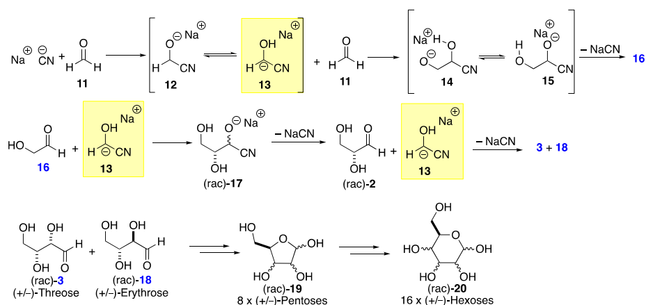
Scheme 3. The formose synthesis of sugars and mechanism.
