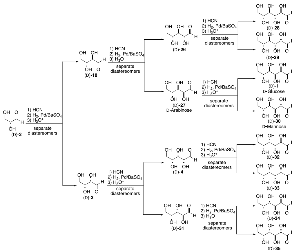
Scheme 6. The Fischer synthesis of all the D-hexoses.
