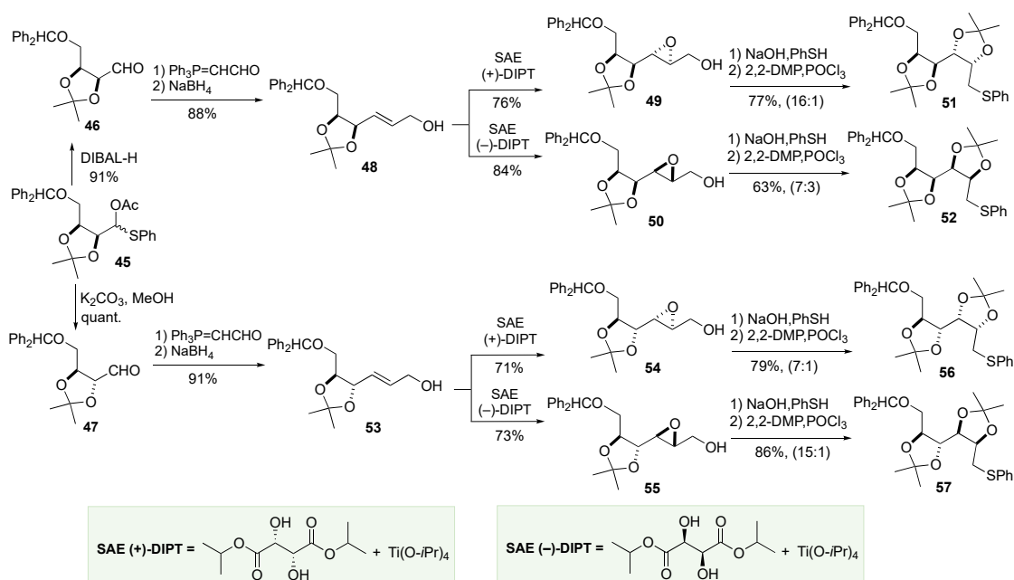
Scheme 10. Sharpless synthesis of C-6 sugars via cis-/trans-acetonide isomerization.
