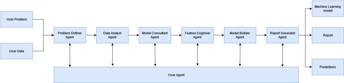
Figure 1. Multi-agents for data science pipeline.
