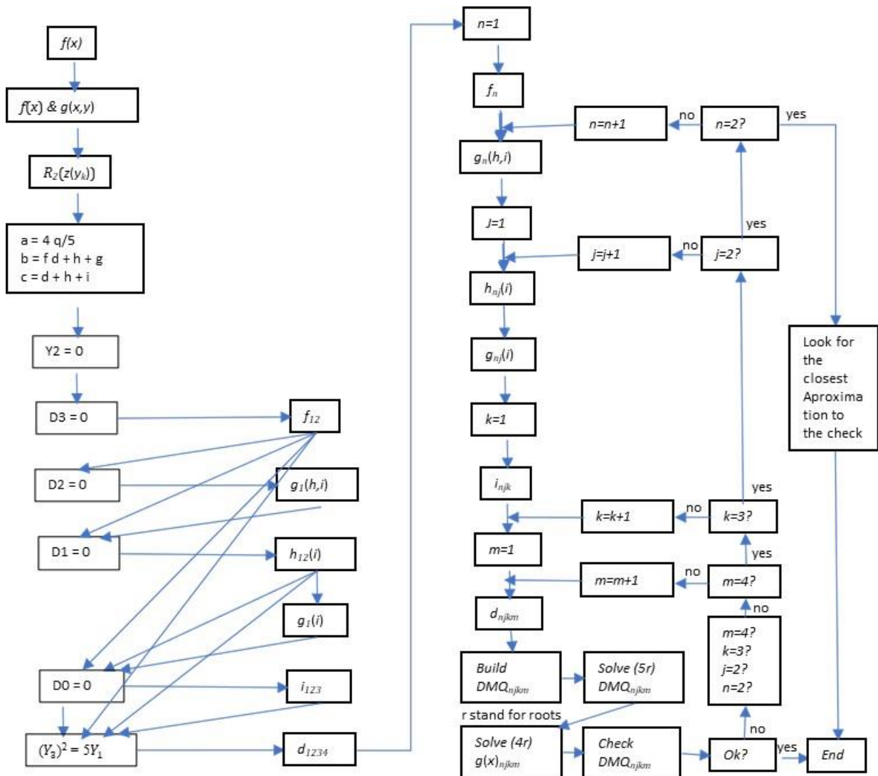
Fig. 5 General Flow Chart applied to the unsolvable Abel's example
