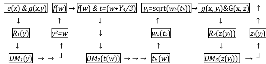
Figure 5. Flowchart of the steps to solve the Bring-Jerrard Normal Sextic Equation (BJS)
