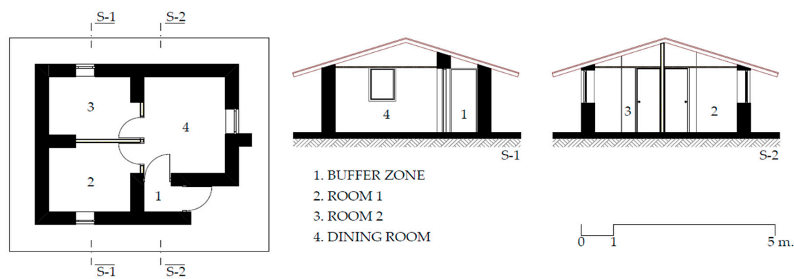
Figure 4. Spatial distribution of the housing module, Cusco.
