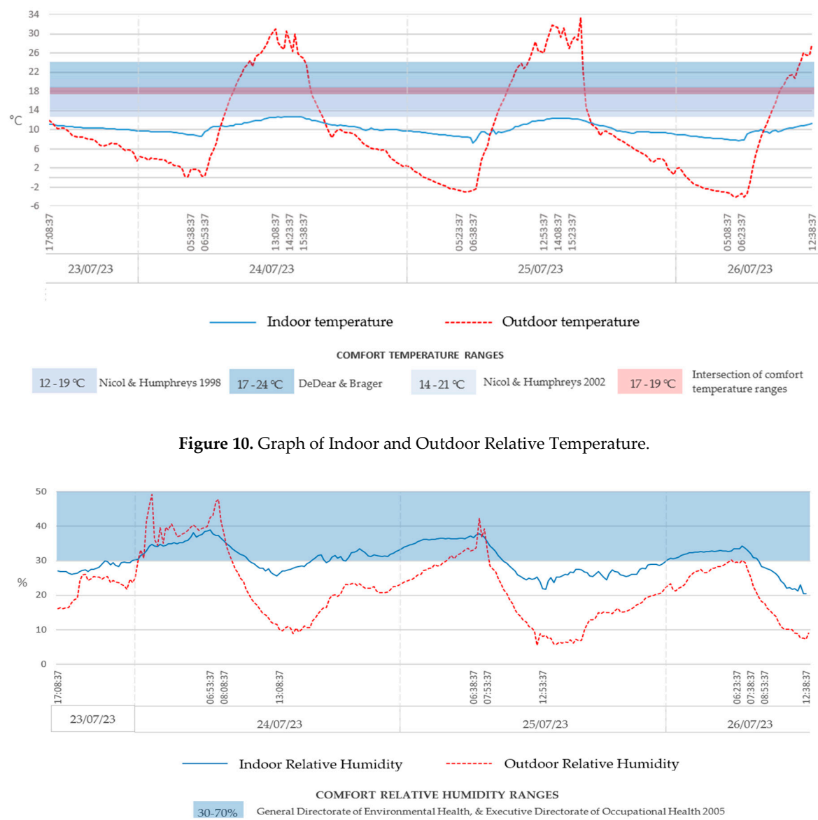
Figure 11. Graph of Indoor and Outdoor Relative Humidity.
