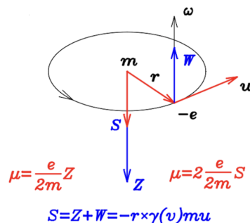
Figure 4. The spinning point particle model of Martin Rivas. The center of charge -e moves along a circular trajectory of Compton radius (noted r in the figure), generating a spin angular momentum S . The center charge is separated from the center of mass m . (Credit: from [14]).
