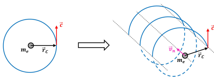
Figure 11. Left: The electron at rest. It consists of an electromagnetic wave moving a speed c along a circle of Compton radius (noted r_c in the figure). Right: Electron in movement with longitudinal velocity \vec{v}_n relative to the proton rest frame. (Credit: C. Dos Santos from [22]).
