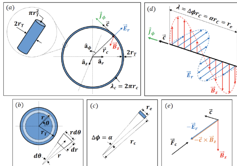
Figure 6. The EM torus of dos Santos. An electromagnetic field shown in (d) above, has a electric field (in blue) and magnetic field (in red). The arc length is the classical electron radius, and the angle \alpha as shown in (c) and (d). The field is confined to the torus on the figure with small radius r_\tau = 1/\sqrt{\pi} * r_e . The field is circulating at the Compton radius as shown in (a). (e) shows the component of the centripetal Lorentz force stabilizing this orbit around the center. (Credit: C. Dos Santos from [19]).
