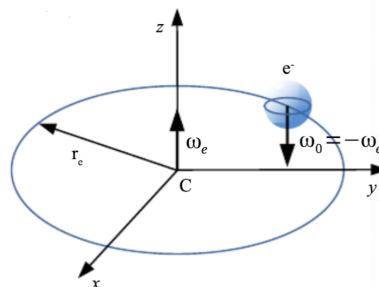
Figure 2. Zitterbewegung model of Vassalo: a charged sphere of Fermi scale is rotating on the circular trajectory of Compton radius (noted r_e in the figure), with angular frequency \omega_e . The ball is counter rotating with frequency -\omega_e . (Credit: G. Vassalo from [11]).
