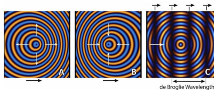
Figure 12. A standing wave at Compton scale becomes a traveling wave under Lorentz boost (indicated by the black arrow). The superposition of the waves A and B produces the traveling wave C, which manifests a de Broglie wavelength with phase velocity c^2/v . (credit: from [25])
