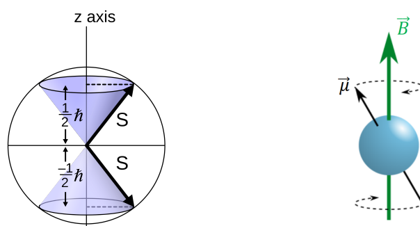
Figure 3. Left: quantum projection of the spin vector \vec{S} on a given direction z ; Right: Larmor precession (with \vec{\mu} magnetic moment vector and \vec{B} external magnetic field).
