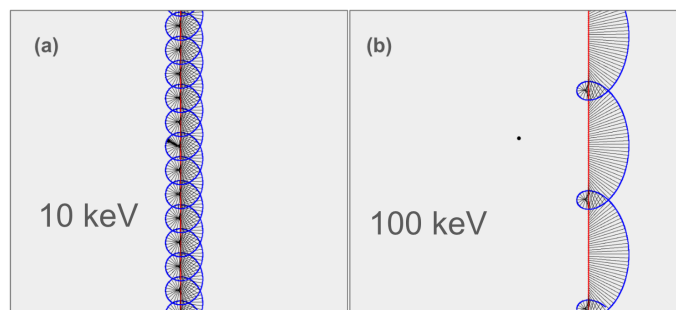
Figure 10. The Cycloid of Rivas. As energy increases to relativistic speeds, here from 10^4 eV (a) on the left to 10^5 eV (b) on the right, a cycloid emerges. The electron mass trajectory is in red, it moves from bottom to top. The electron charge position is in blue and orbits about the center of mass. Here the spin is left, the charge moves counter-clockwise around the center of mass. As the center of mass reaches relativistic velocities the cusps appear as the charge is moving counter to the mass. In all these simulations the spin is co-planar to the orbit: the spin is in the plane of the picture. (Credit: Marc Fleury).
