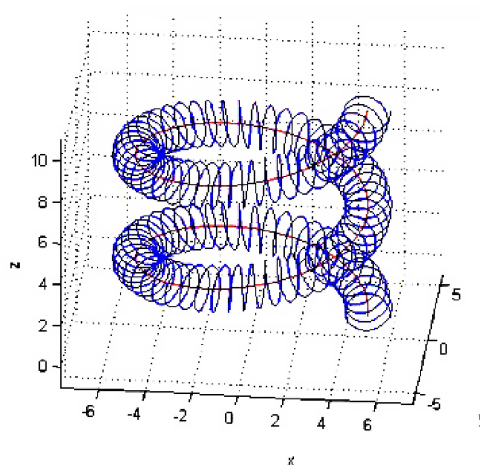
Figure 8. Helicoidal solenoid electron moving in the z direction. (Credit: O. Consa from [9]).
