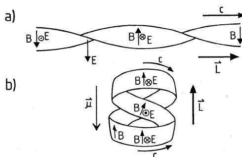
Figure 7. The toroidal model of Williamson. a) free photon with circular polarization of electric and magnetic fields \vec{E}/\vec{B} ; b) photon confined on the double loop, making appear the charge, magnetic moment \mu and orbital angular momentum \vec{L} (spin). The toroidal structure is characterised by a radius r = \lambda_c/4\pi . (Credit: from [20]).
