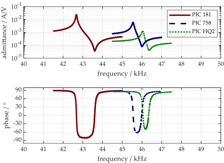
Figure 6. Small signal admittance characteristics (free vibration, room temperature).
