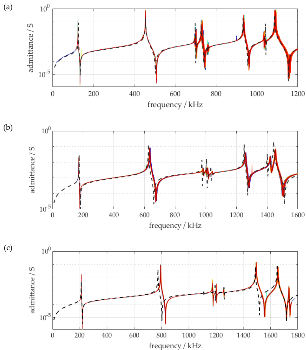
Figure 4. Measured frequency responses of the short-circuit input admittance of 50 individual ring ceramics (coloured solid lines) compared to simulation results (dashed black line) for (a) PIC 181, (b) PIC 758, (c) PIC HQ2. Please remark the different frequency ranges used in the diagrams for convenience.
