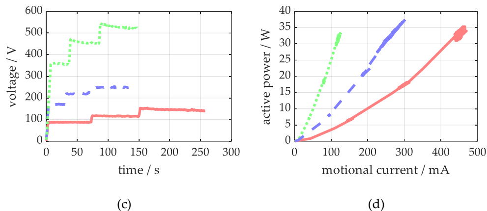
Figure 9. Results of the load tests with heat up (immersion of the transducer tip into water, controlled vibration at different levels of motional current, continuous drive until steady state temperature): (a) motional current amplitude over time, (b) temperature rise over time, (c) voltage amplitude over time, and (d) active power over motional current amplitude.
