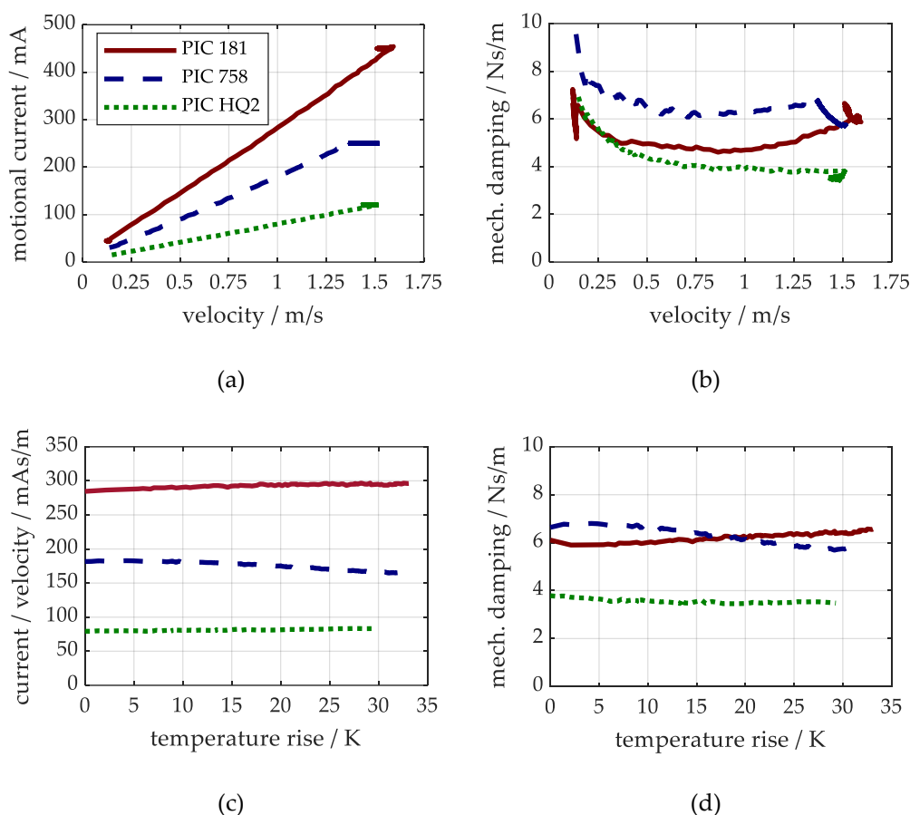
Figure 7. Results of tests (resonance controlled continuous vibration up to 1.5 m/s, heat up over time): (a) Dependency of tip velocity and motional current, (b) mechanical damping factor over tip velocity, (c) ratio of motional current and tip velocity over temperature rise, and (d) mechanical damping factor over temperature rise.
