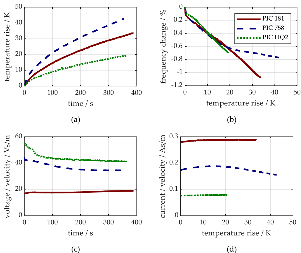
Figure 5. Results of the burn-in process (free resonant vibration at \approx 1 m/s for \approx 6 minutes), : (a) Temperature rise over time, (b) resonance frequency change over temperature rise, (c) voltage related to tip velocity over time, (d) motional current related to tip velocity over temperature rise.
