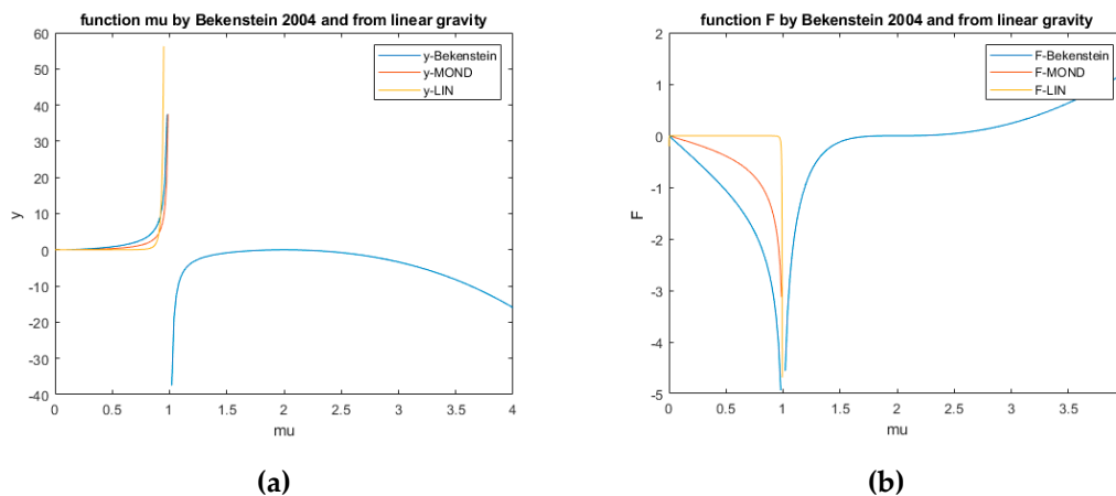
Figure 11. Function y(\mu) of Bekenstein and linear gravity (a) Function F(\mu) of Bekenstein and linear gravity (b).
