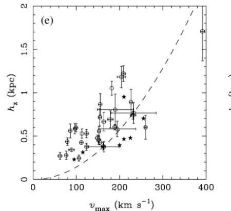
Figure 3. Vertical disk scale length vs. Vobs after de Kregel et al [33].
