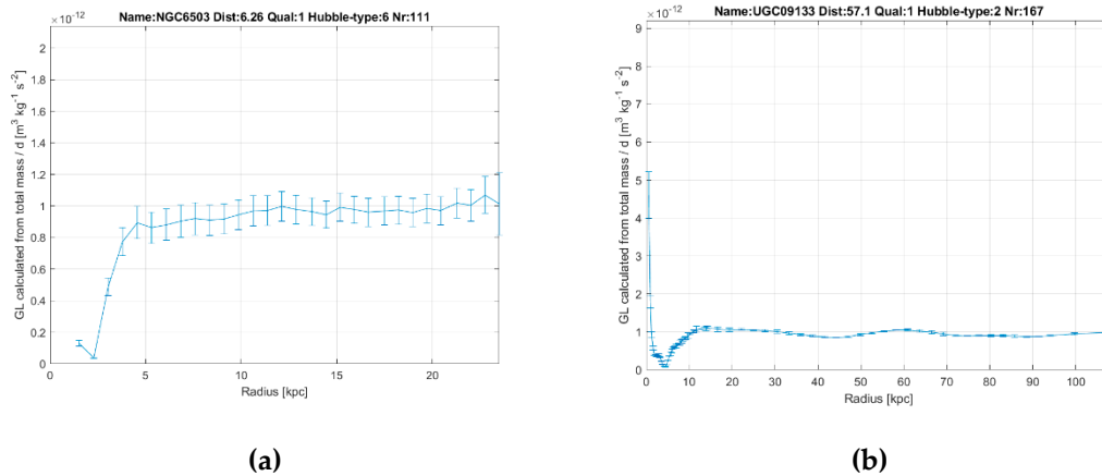
Figure 7. G_L as function of radius in galaxy examples (a) NGC6503; (b) UGC09133; the complete figure set of 175 figure is available in Annex 2.
