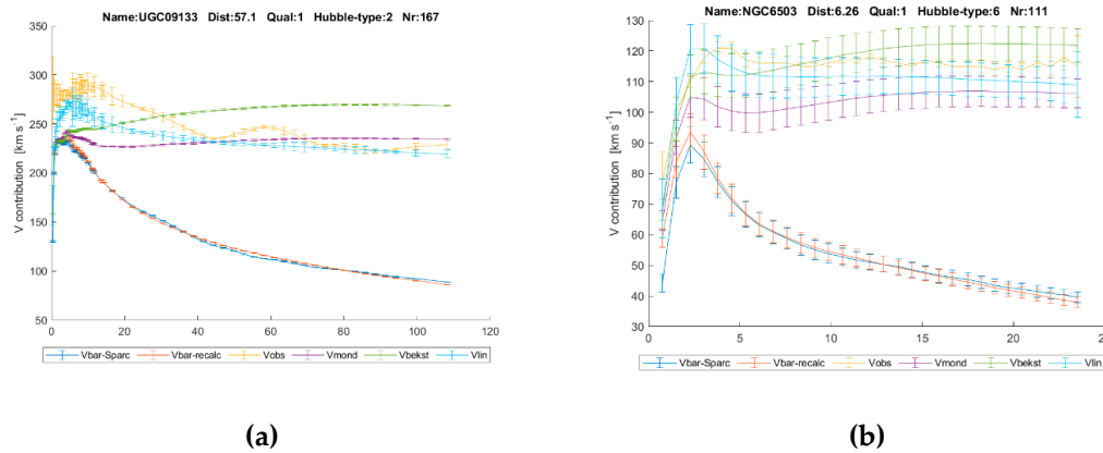
Figure 10. Examples of rotation curves with MOND, TeVeS and linear gravity predictions; (a) UGC09133, (b) NGC 6503; the complete figure set of 175 figure is available in Annex 3.
