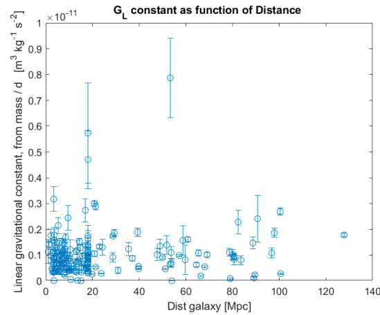
Figure 8. G_L for all 175 galaxies.
