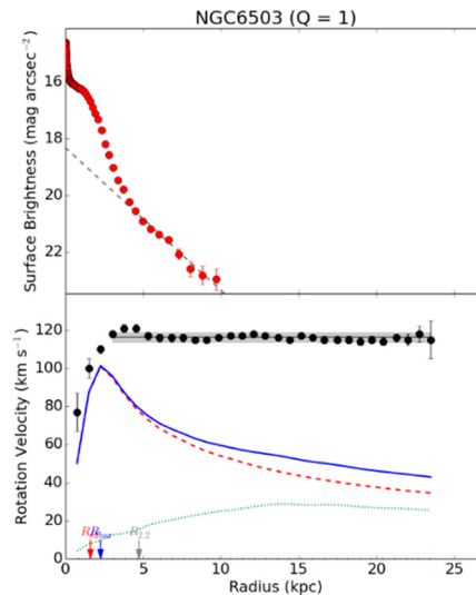
Figure 1. rotation curve sample [11].
