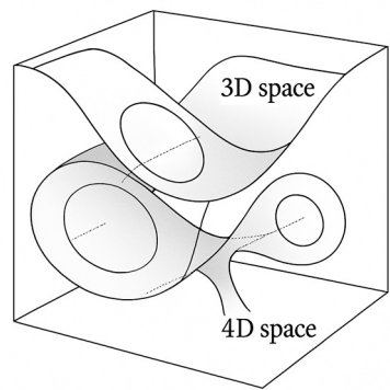
Figure 2. Folded 3D spaces filling a 4D space in orthogonal directions.
