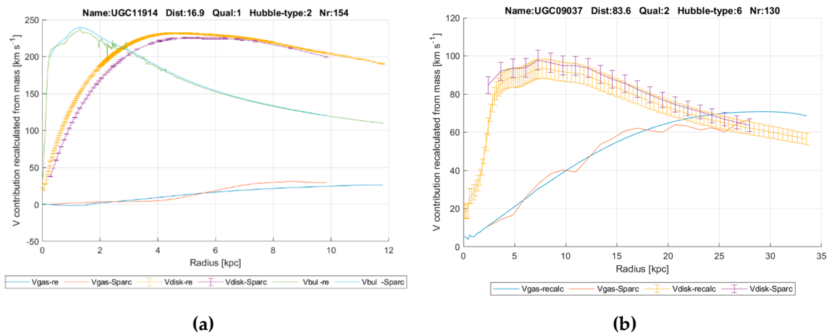
Figure 4. V_{gas} , V_{disk} and V_{bulge} from SPARC team and from author assuming mass-light-ratio Y_{ml} = 1 (a) UGC11914; (b) UGC09037; the complete figure set of 175 figure is available in Annex 1.
