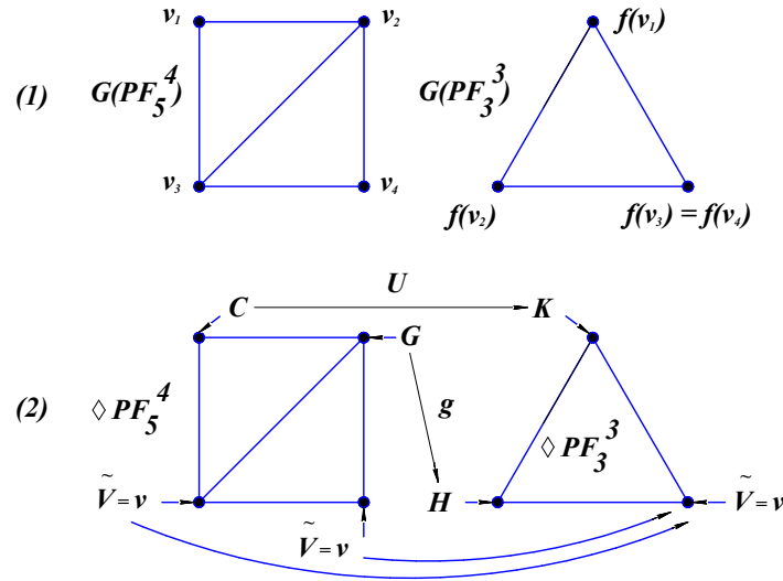
Figure 2. Condition 1. The image of G(PF_5^4) under the strict homomorphism is G(PF_3^3) . Condition 2. U is a functor; g is a homomorphism of groups.
