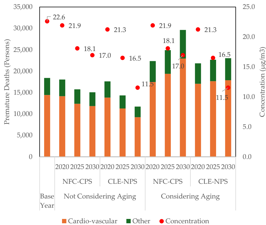
Figure 8. Number of premature deaths due to PM 2.5 by scenario and year, Not considering and considering the impact of aging.
