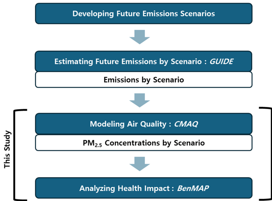
Figure 3. Future PM 2.5 concentration estimation process.
