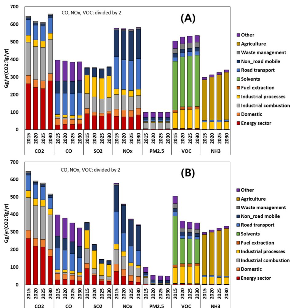
Figure 5. (A) Future emissions by NFC-CPS scenario from 2015 to 2030; (B) Future emissions by CLE-NPS scenario from 2015 to 2030.
