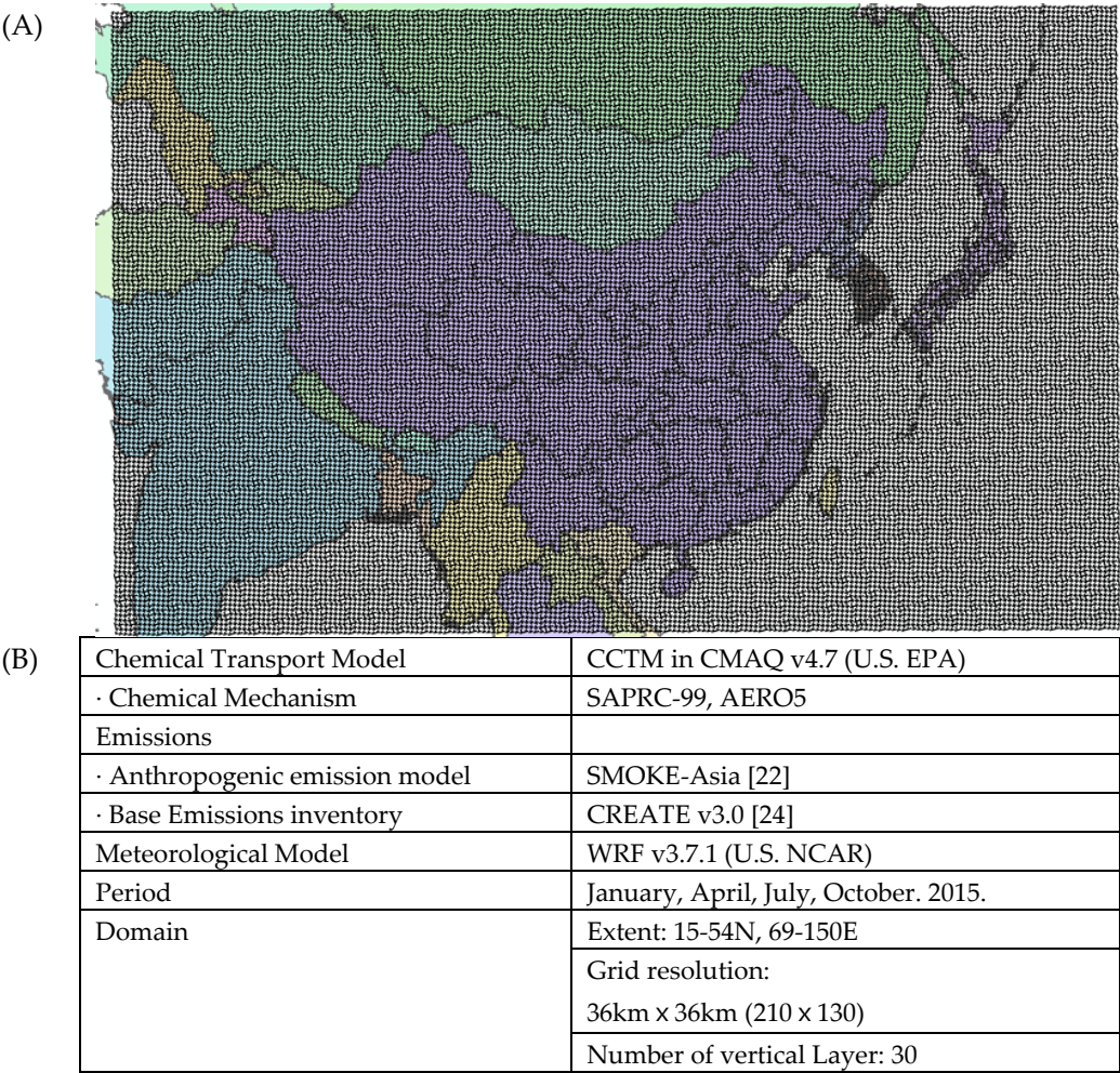
Figure 6. (A) Modeling domain (36 x 36km 2 grid); (B) Chemical transport model framework.
