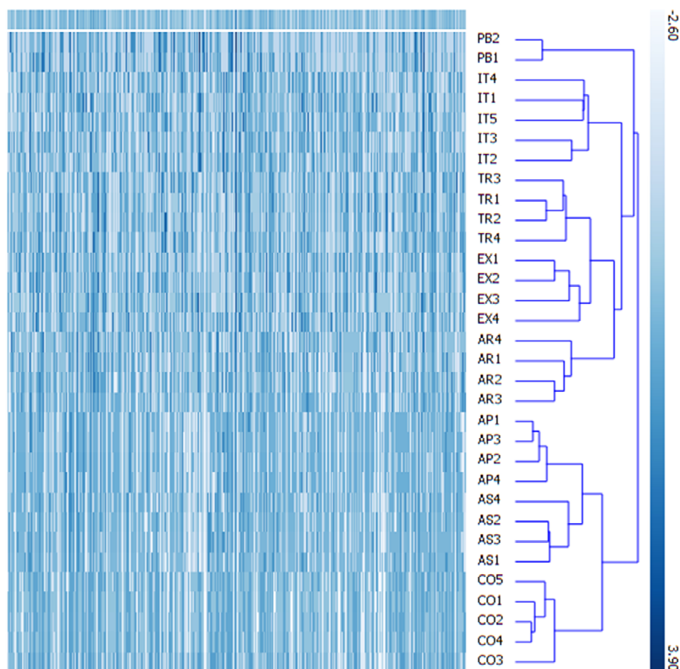
Figure 3. Hierarchical group heat map by indicators.
