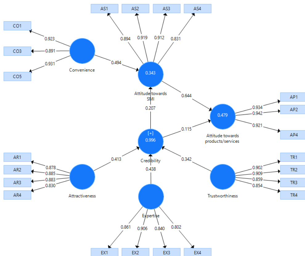
Figure 6. SEM procedure validity result – path coefficients and coefficients of determination.
