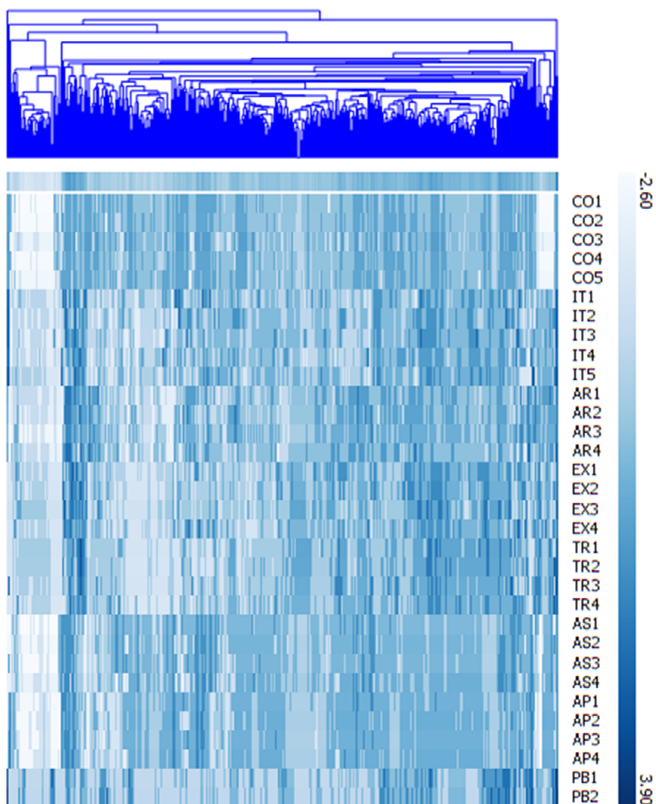
Figure 2. Hierarchical group heat map by respondents.
