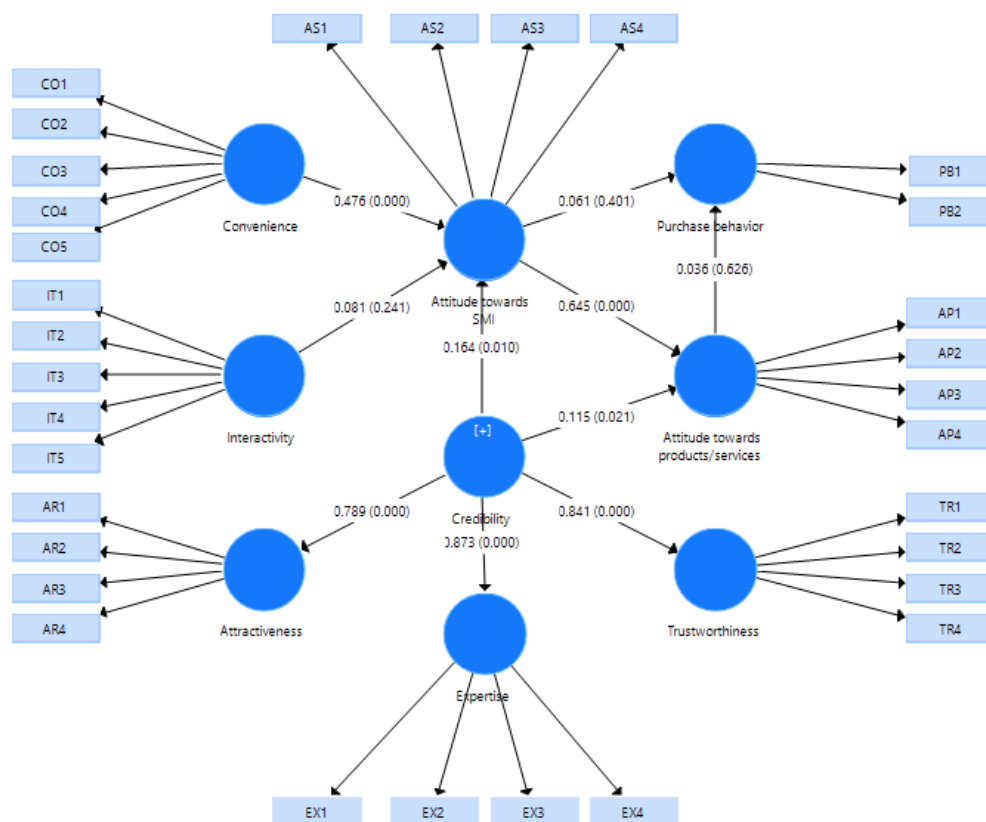
Figure 5. Measurement model with six latent variables, their path coefficients and p -values.
