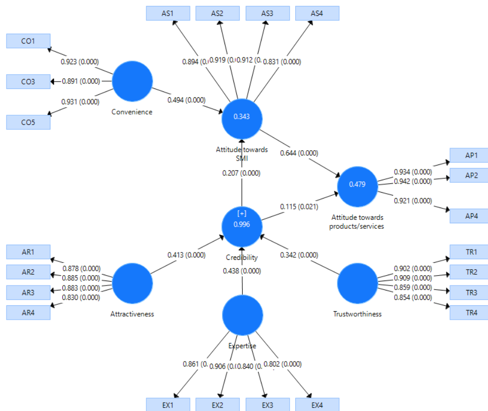
Figure 7. Path coefficients and p -values—inner and outer model.
