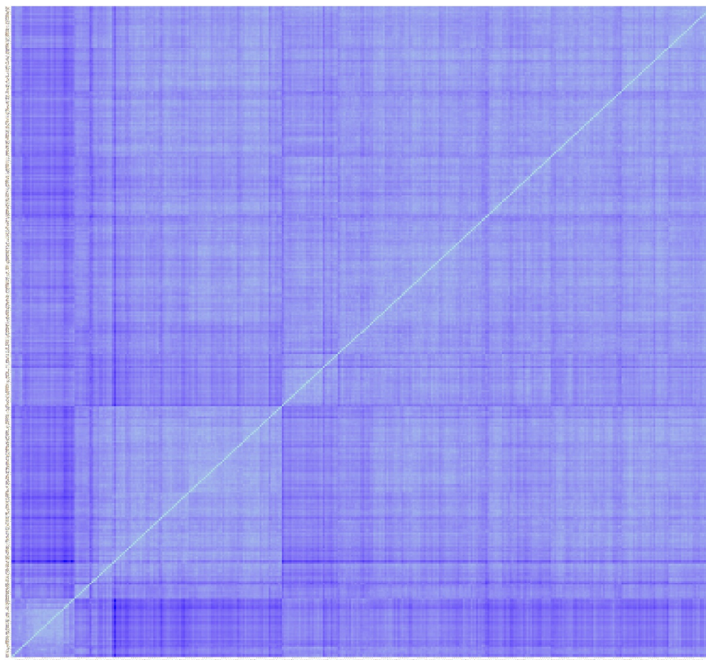
Figure 1. The ordered dissimilarity matrix of respondents' answers.
