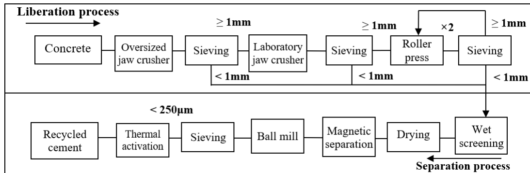
Figure 1. Flowchart of the novel liberation and separation method. (Carrico, et al., 2021).
