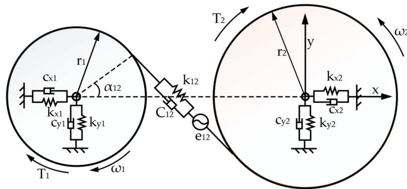
Figure 18. Translational-rotational model of a fixed-shaft gear set.
