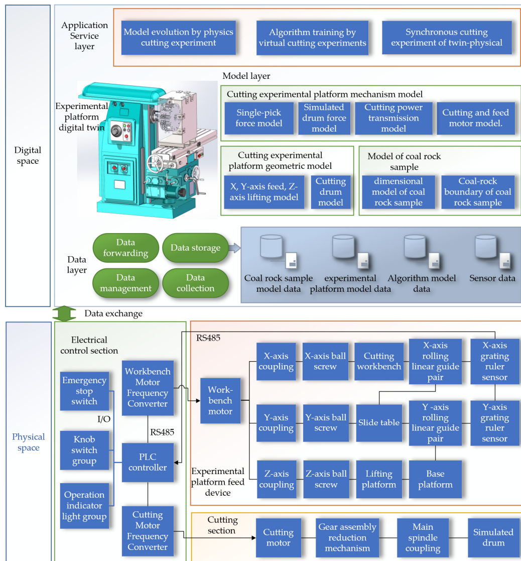
Figure 2. Digital Twin Cutting Experiment System Block Diagram.
