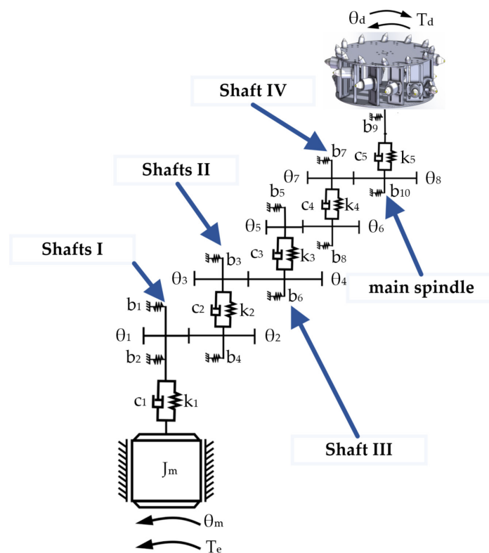
Figure 19. Lumped parameter model for the multistage gearbox.
