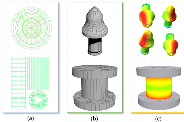
Figure 22. (a) Expanded UV grid; (b) UV mapping; (c) heat map rendering.
