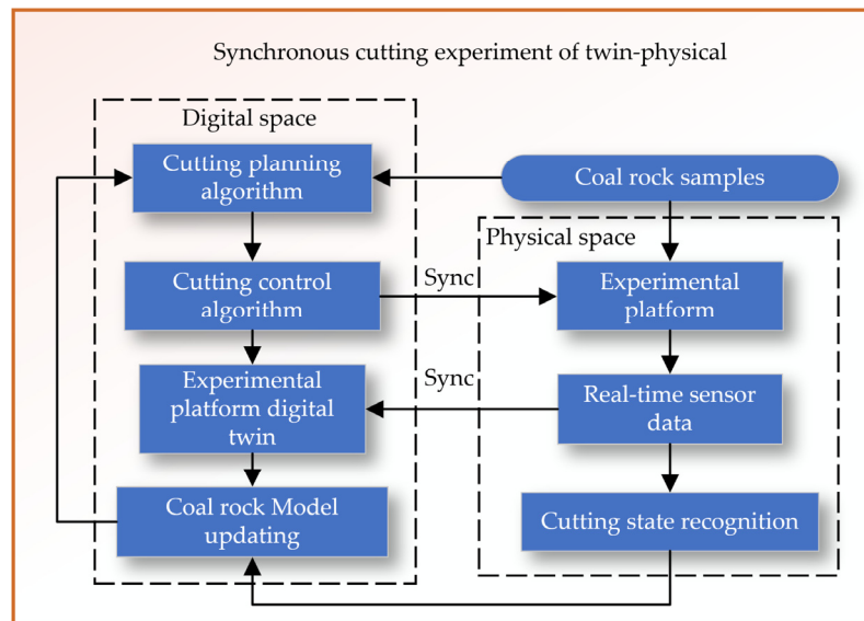
Figure 16. Synchronous cutting experiment of twin-physical.
