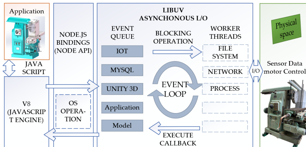
Figure 21. The architecture and process of a data application developed using Node.js.
