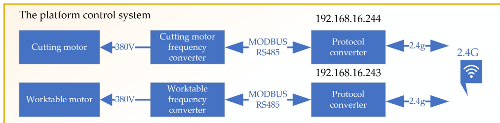
Figure 12. The Platform Control System Block Diagram.
