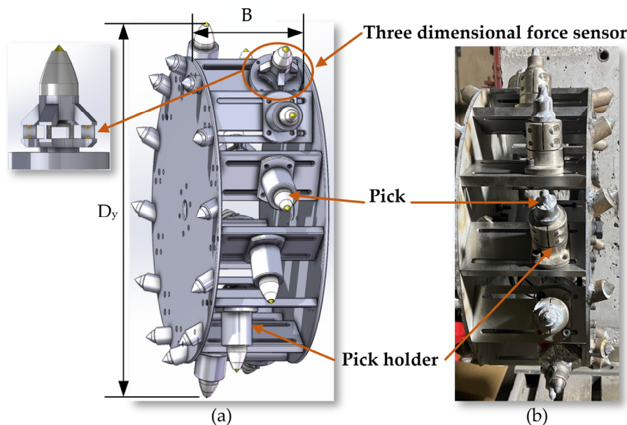
Figure 4. (a) The model of the cutting drum; (b) The physical cutting drum.
