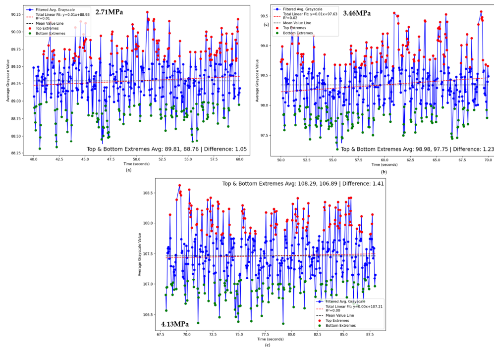
Figure 29. (a) Experimental mode one; (b) Experimental mode two; (c) Experimental mode three.
