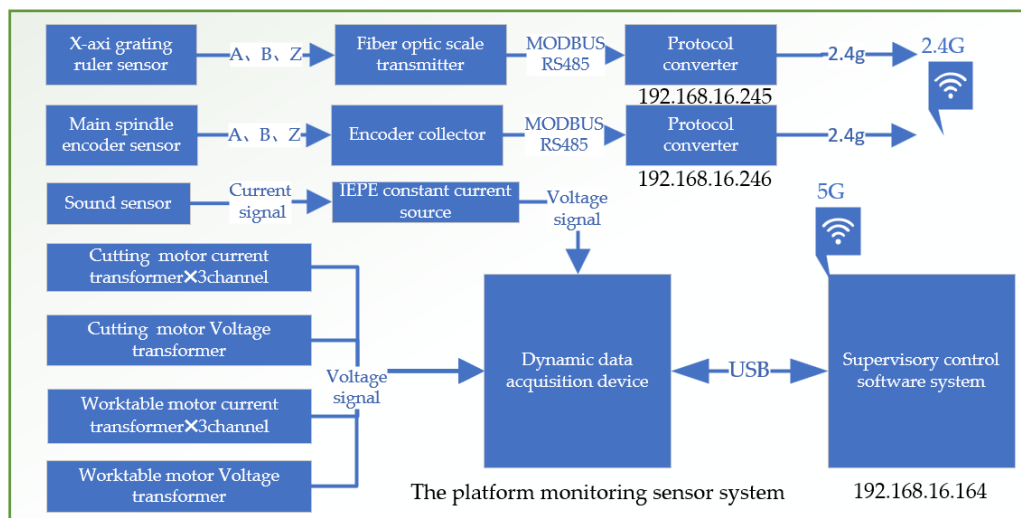
Figure 11. The Platform Signal Acquisition System Block Diagram.
