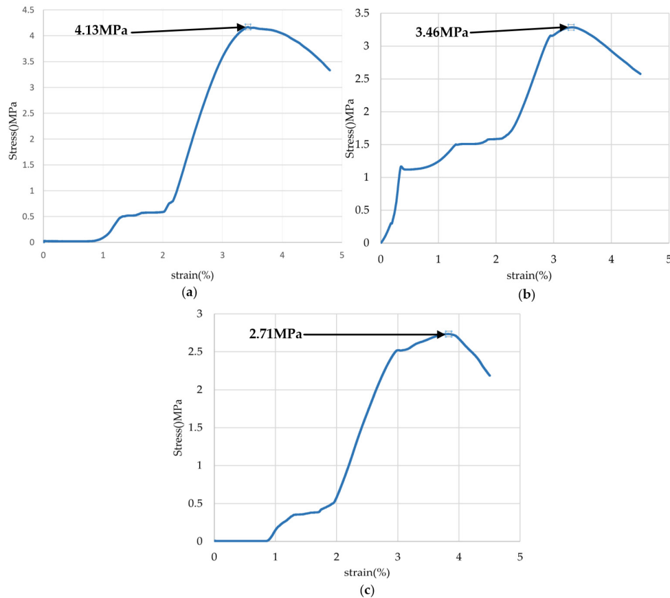
Figure 26. Stress-strain curve of simulated coal sample (a) 4.13MPa; (b) 3.46MPa; (c) 2.71MPa.
