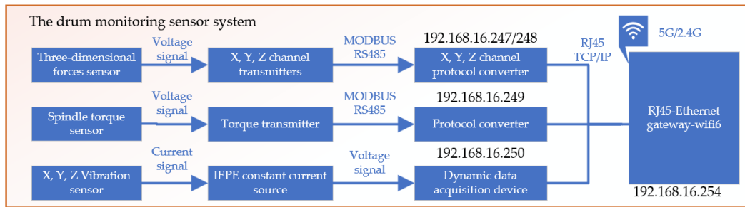
Figure 8. The Drum Signal Acquisition System Block Diagram.
