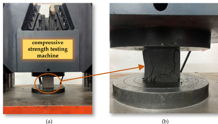
Figure 25. (a) Concrete Compressive Strength Testing Machine; (b) Tensile Strength Test.
