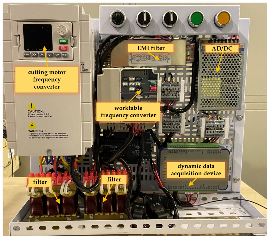
Figure 13. Electrical Control Device for the Cutting Experimental Platform.
