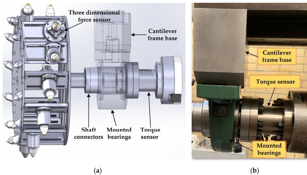
Figure 5. (a) The model of the platform spindle; (b) The physical platform spindle.
