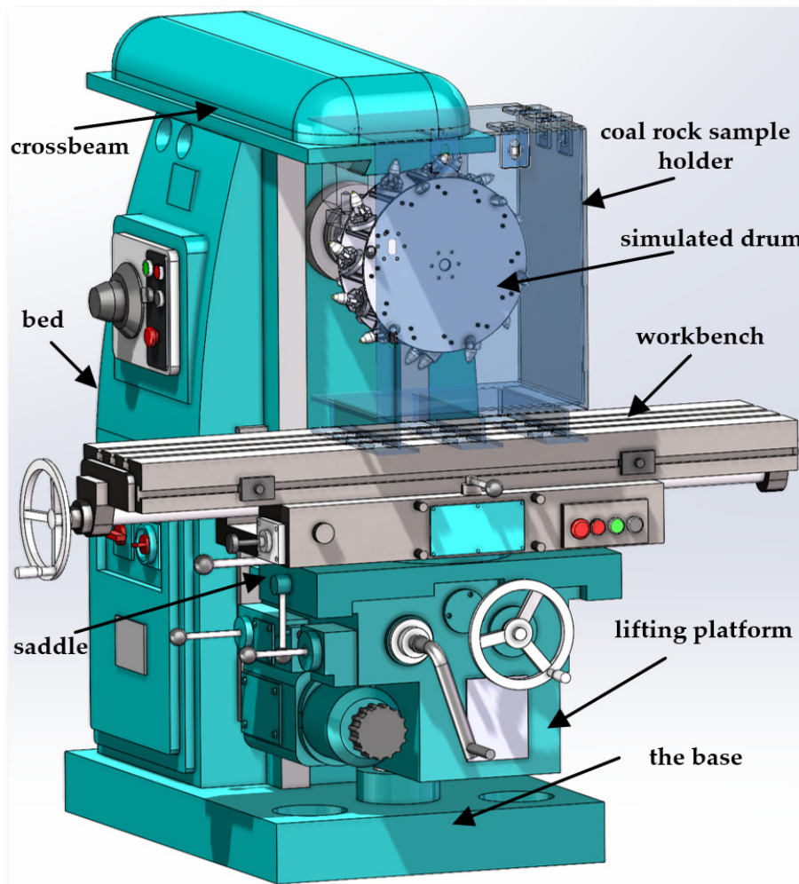
Figure 17. The geometric models of the cutting experiment platform.
