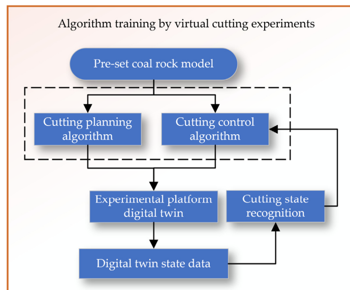
Figure 15. Algorithm training by virtual cutting experiments.
