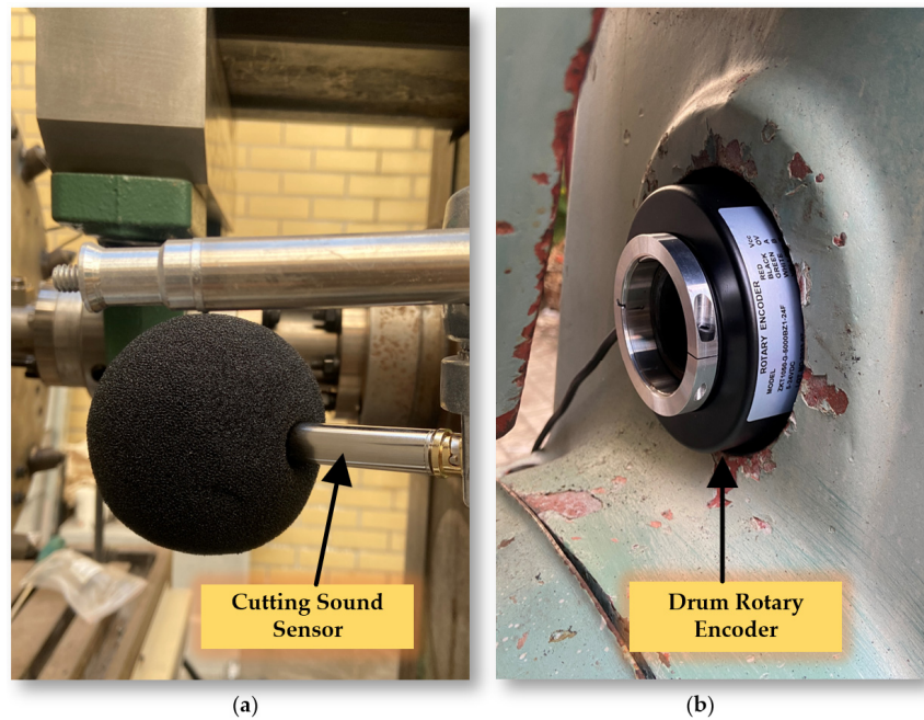
Figure 10. (a) Cutting Sound Sensor; (b) Drum Rotary Encoder.
