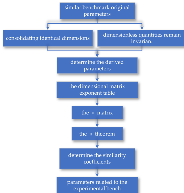
Figure 3. The simulation cutting drum builds processes based on similarity theory.
