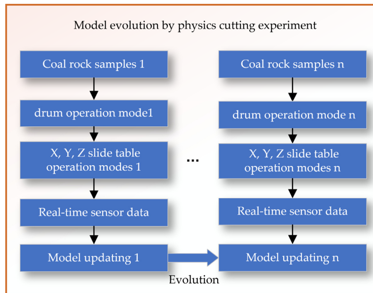
Figure 14. Model evolution by physics cutting experiment.
