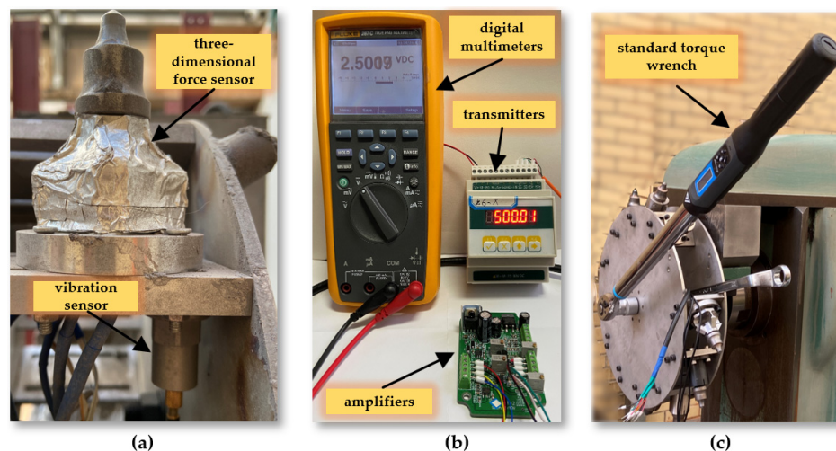
Figure 7. (a) arrangement of sensors; (b) force sensor calibration; (c) torque sensor calibration.
