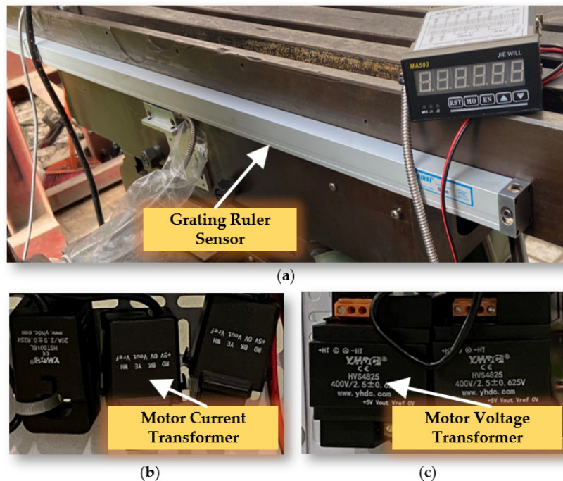
Figure 9. (a) Grating Ruler Sensor; (b) Motor Current Transformer; (c) Motor Voltage Transformer.
