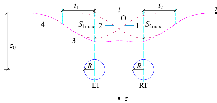
Figure 2. Peck Prediction Curve for Surface Settlement in Two-Lane Tunnel Excavation.
