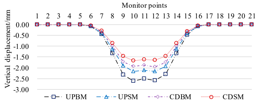
Figure 10. Calculation curves of Peck's settlement at monitoring points of existing tunnel base plate under different calculation conditions.
