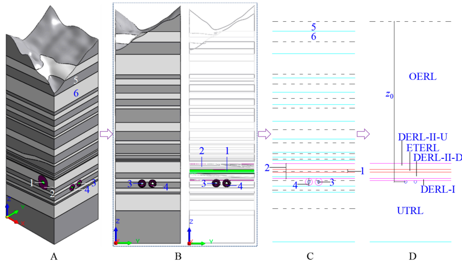
Figure 6. Spatial relationship and rock layer diagram of the underpassing two-lane tunnel and the existing tunnel: A is the three-dimensional spatial relationship, B is the X-direction side view, C is the two-dimensional rock layer and spatial relationship, and D is the spatial relationship transformed by the layer method, 1 is the structure of the existing tunnel, 2 is the dynamic and static load influence area of the existing tunnel, 3 is the structure of the underpassing tunnel, 4 is the dynamic and static load influence area of the excavation of the underpassing tunnel, 5 is the mudstone, and 6 is the Malmstone.
