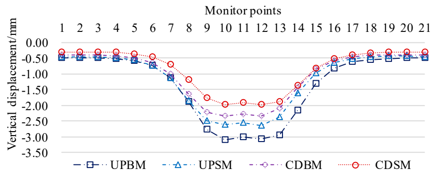
Figure 9. Displacement and settlement curves of the existing tunnel base plate under different calculation conditions.
