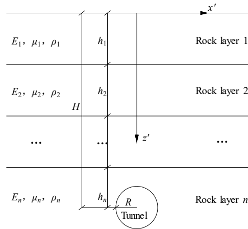
Figure 4. Schematic diagram of the location of the multi-layered soil and rock layers overlying the tunnel.
