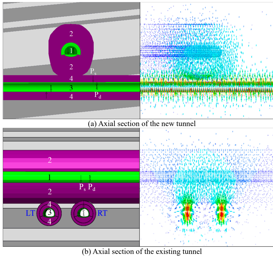
Figure 1. Schematic diagram of the location of the overlying multi-layered geotechnical layers of the tunnel: 1 is the existing tunnel structure, 2 is the area of the rock layer affected by the dynamic and static loads of the existing tunnel, 3 is the structure of the tunnel underneath, 4 is the area affected by the dynamic and static loads of the tunnel excavation underneath, P_s is the static load, and P_d is the dynamic and static load.
