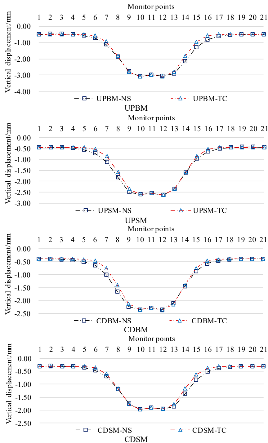
Figure 12. Comparison of numerical calculations and Peck's theoretical calculations of the settlement of the base plate of existing tunnels under different working conditions.
