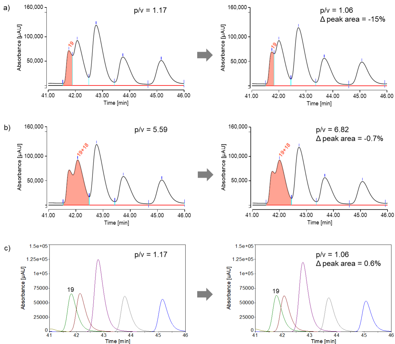
Figure 5. Variations in peak areas ( \Delta peak area) due to altered peak-to-valley ratio ( \Delta p/v ) of strongly overlapping peaks and potential solutions. a) A change in the peak-to-valley ratio of highly overlapping peptide 19 between injection #10 (left side) and #20 (right side) led to an integration error of -15% when using the perpendicular drop method. b) By grouping the peaks of peptides 19 and 18, the integration error of the vertical drop method could be reduced from -15% to only -0.7%. c) Peak fitting enabled a precise determination of the peak area even for the highly overlapping peptide 19. The peak area deviation was 0.6%. For detailed instructions on peak fitting, refer to section 2.4. Peak-to-valley ratios were calculated for injection #10. The percentage values also refer to injection #10.
