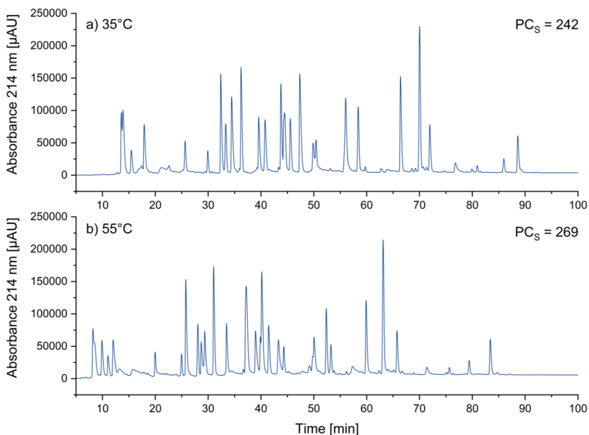
Figure 4. Influence of increasing temperature on the separation (sample peak capacity, PC_s ) of the CEF advanced peptide pool containing 32 peptides. a) 35°C; b) 55°C. A small increase of the sample peak capacity was obtained. Additionally, retention times decreased. The peptide sequences are listed in Table 2 . For UHPLC conditions, please refer to Section 2.3.
