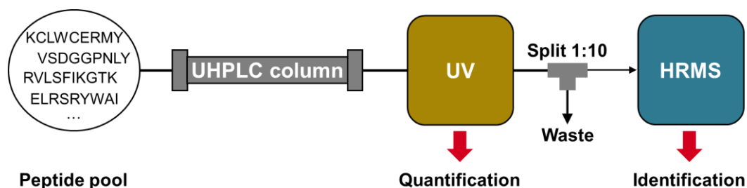
Figure 1. Simplified experimental setup for a cost- and time-efficient analysis of a peptide pool. Each of the two detectors serves a specific purpose and is used in combination. Quantification is performed using an ultraviolet (UV) detector, here at 214 nm, while identification is performed using high-resolution mass spectrometry (HRMS). Expensive internal standards labeled with stable isotopes, as well as calibration and identification runs are usually not required. However, it should be noted that the sensitivity of the UV and MS detector may need to be adjusted once during the setup, for example by using different splitting ratios, MS conditions and/or online dilution (not shown).
