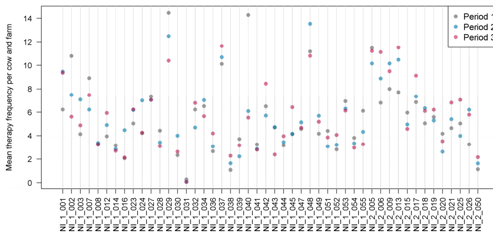
Figure 1. Mean therapy frequency per cow and farm in Q fever vaccinated and non-vaccinated dairy farms during the study periods (NI_1 = Q fever vaccinated farms, NI_2 = non-vaccinated farms). Each dot represents a farm, the different colours indicate different time periods.
