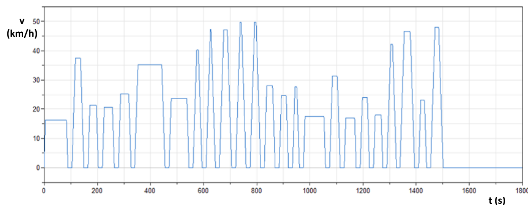
Figure 4. Model for the urban route.
