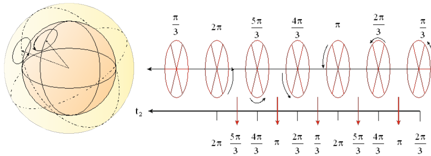
Figure 2. The wave function in the time dimension is the sum of the small packets that make up the mass field.
