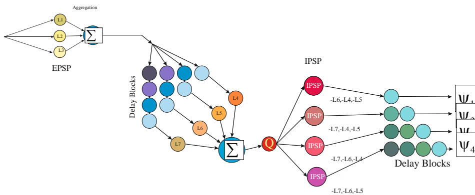
Figure 5. Different pulses are stored in memory after integration, aggregation and compression of information. Each spike current represents a unique wave function containing distinct pieces of information.
