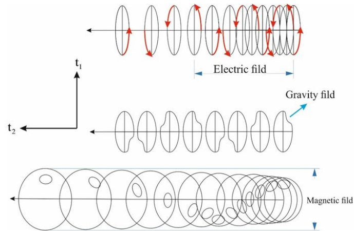
Figure 3. The relationship between the electric field and the magnetic field with the gravitational field is when the states of the wave function approach each other. Accordingly, there are three fields of information. which can be introduced in an information unit.
