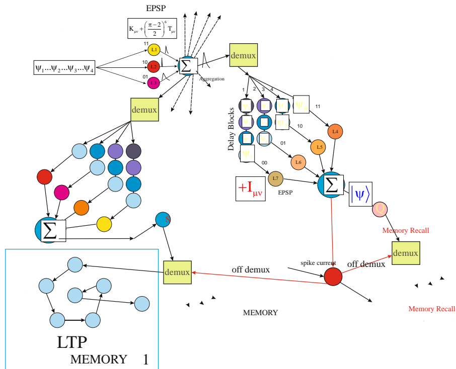
Figure 5. Different pulses are stored in memory after integration, aggregation and compression of information. Each spike current represents a unique wave function containing distinct pieces of information.
