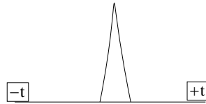
Figure 4. Each pulse contains compressed information.
