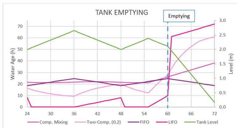
Figure 20. Evolution of water age when the tank empties.
