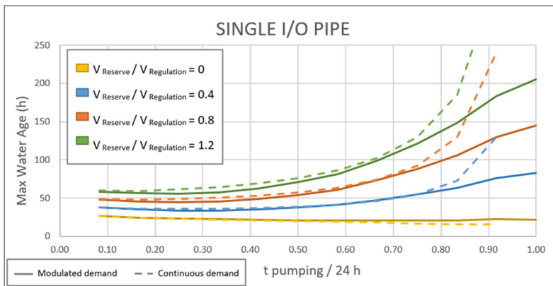
Figure 7. Evolution of water age in a tank with single pipe connection to the network.
