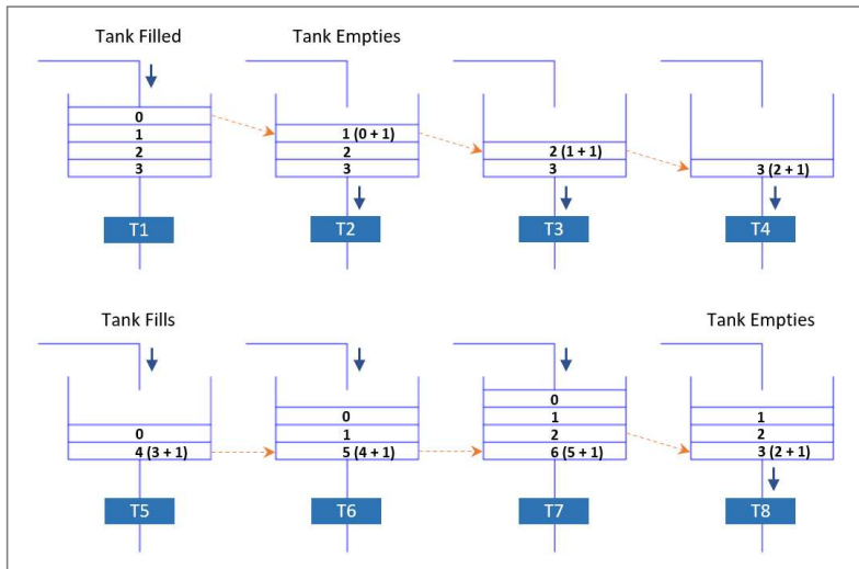
Figure 14. Evolution of water age in the parcels of the tank. FIFO Plug Flow. Numbers on parcels stand for the water age, in h. Each figure represents the evolution of parcels for a time step of 1 h.
