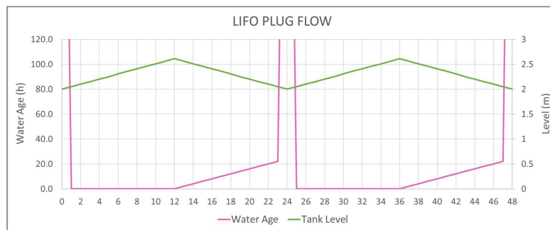
Figure 17. Evolution of water age and tank level. LIFO Plug Flow.
