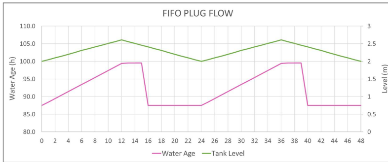
Figure 15. Evolution of water age and tank level. FIFO Plug Flow.
