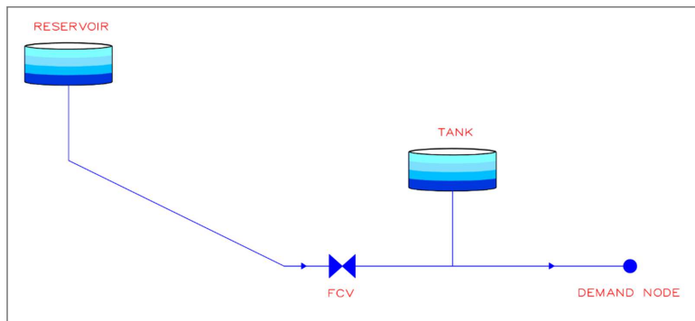
Figure 9. Case Study 1 network diagram.
