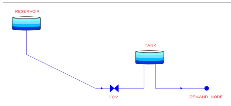
Figure 18. Case Study 2 network diagram.
