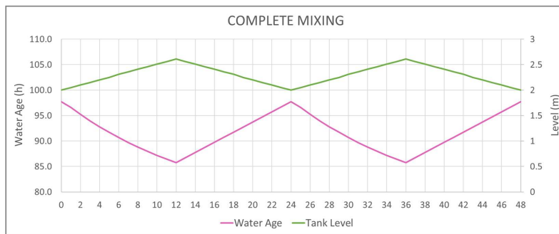
Figure 11. Evolution of water age and tank level. Complete mixing.
