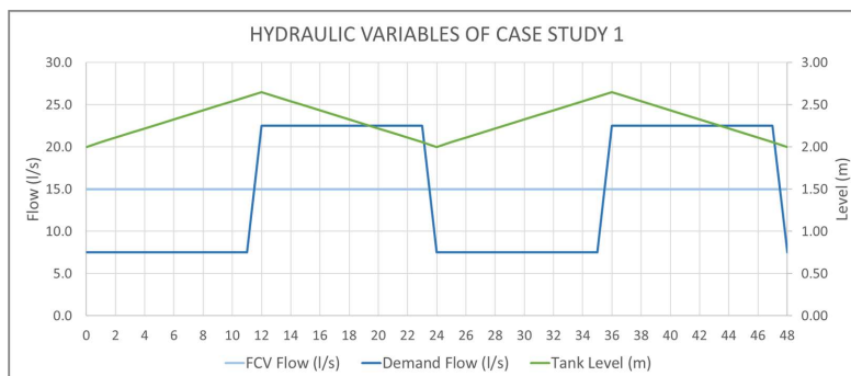
Figure 10. Evolution of the main hydraulic variables of Case Study 1.
