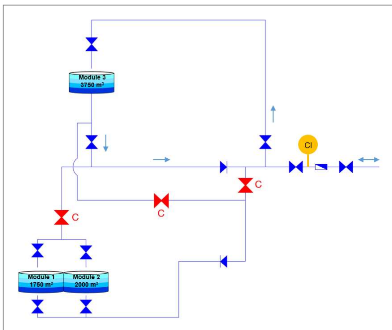
Figure 23. Tank configuration when performing the field tests. Modules 1 and 2 are isolated.
