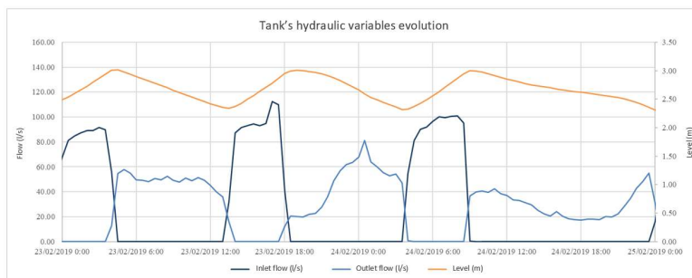
Figure 22. Evolution of the tank level, inlet and outlet flows.
