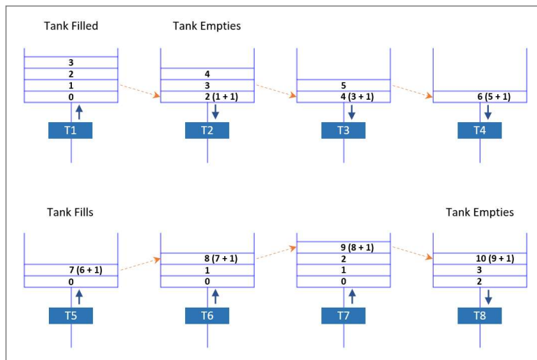
Figure 16. Evolution of water age in the parcels of the tank. LIFO Plug Flow. Numbers on parcels stand for the water age, in h. Each figure represents the evolution of parcels for a time step of 1 h.
