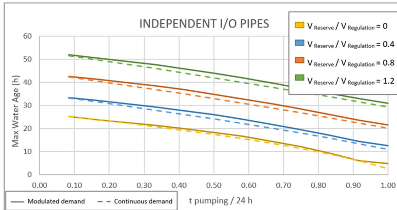
Figure 8. Evolution of water age in a tank with independent inlet/outlet pipe connection to the network.
