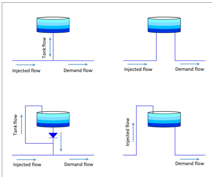
Figure 3. Single (left) and independent (right) pipe connections to the system, with bottom inlet pipes (up) and upper inlet pipes (down).
