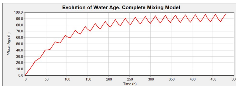
Figure 5. Evolution of water age on a tank. Complete mixing model.
