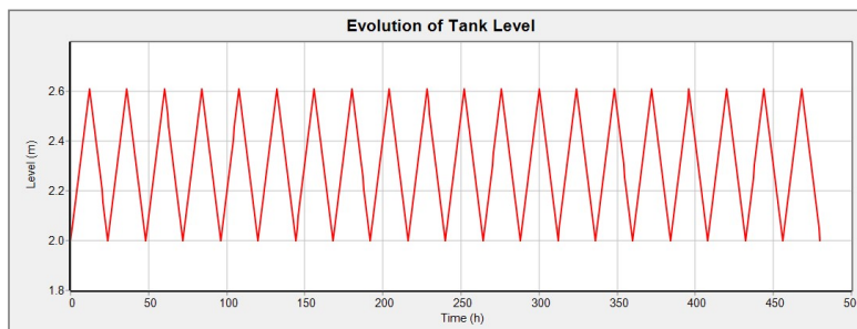
Figure 4. Evolution of a tank level. Cyclic behaviour.
