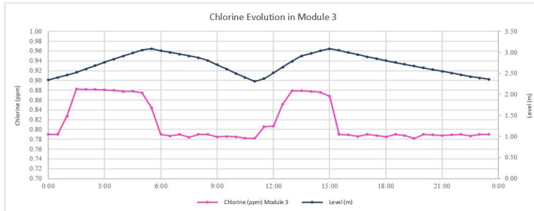
Figure 24. Tank level and chlorine evolution in Module 3.
