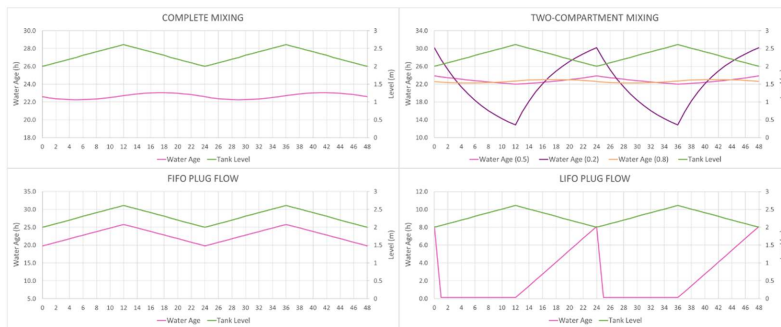
Figure 19. Evolution of water age and tank level for all four Epanet tank mixing models. Independent I/O pipes.
