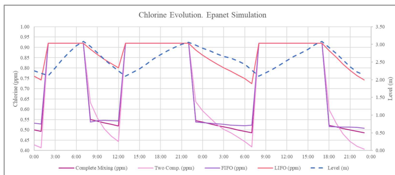
Figure 26. Simulated chlorine evolution for all mixing models available in Epanet.
