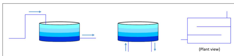
Figure 2. Inlet/Outlet pipe configuration and baffles in tanks (from left to right).
