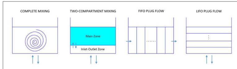
Figure 1. Tank mixing models in Epanet [7].
