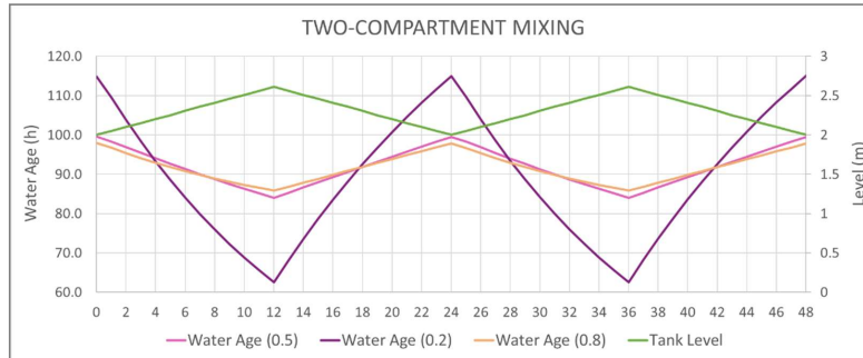
Figure 12. Evolution of water age and tank level. Two-Compartment mixing.
