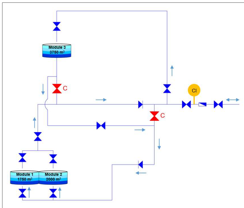
Figure 21. Tank configuration (plant view).
