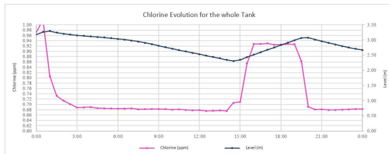
Figure 25. Tank level and chlorine evolution with all three modules operating.
