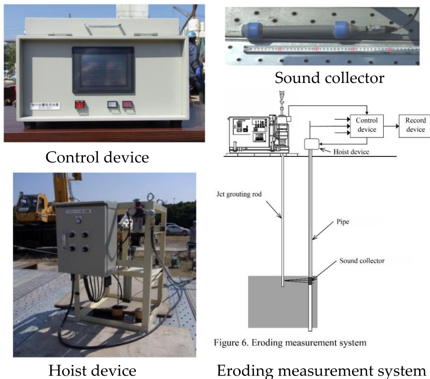
Figure 8. Acoustic monitoring system [11].
