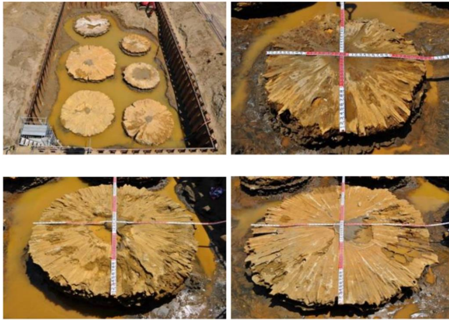
Figure 1. Excavated V-Jet columns [11].
