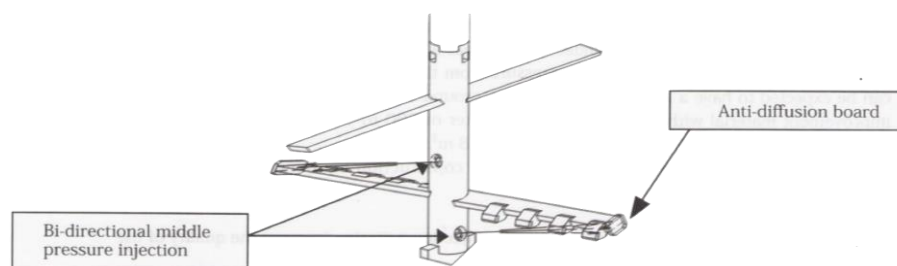
Figure 3. Schematic diagram of MITS monitor.
