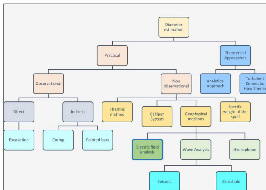
Figure 6. Categorization of the soil-cement diameter estimation methods [29].
