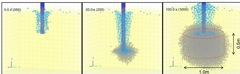
Figure 12. Simulation-based evaluation and visualization of traditional jet grouting process at 18 MPa [14].
