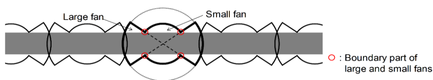
(b) MultiFan-shaped jet grouting layout
