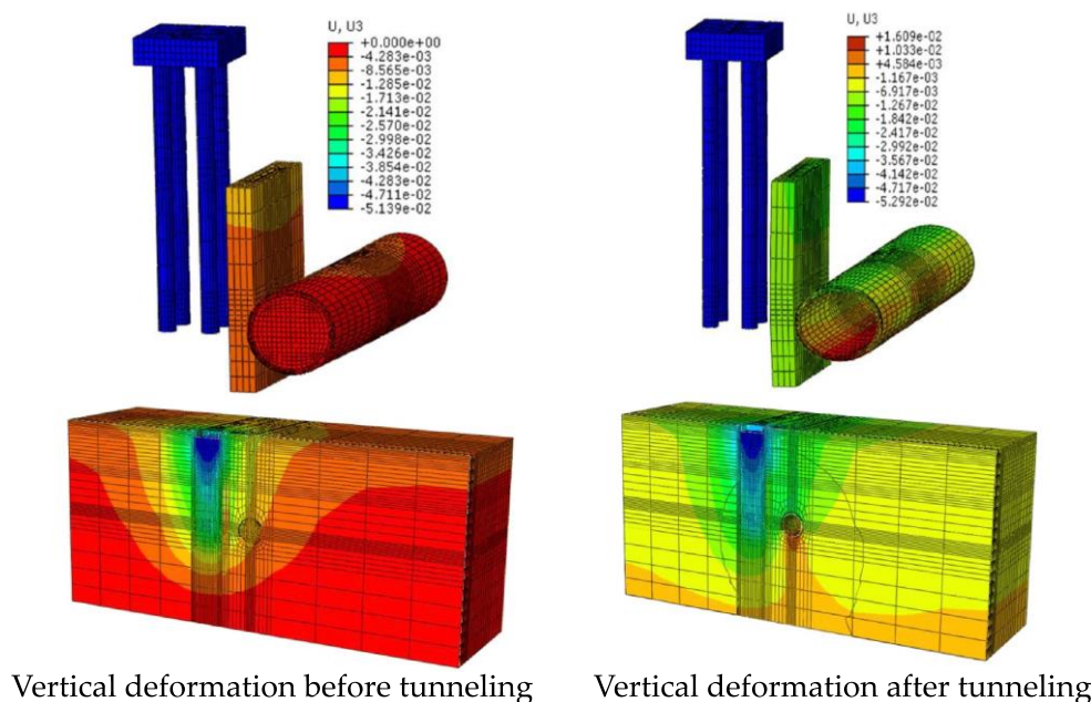
Figure 10. Vertical deformation before and after tunneling [67].
