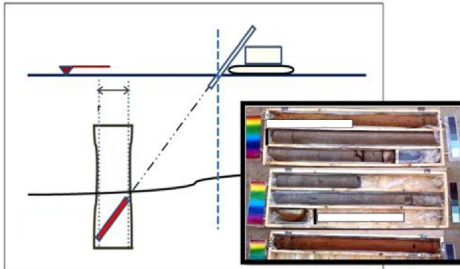
Figure 7. Inclined core sampling for unconfined compression test [29].
