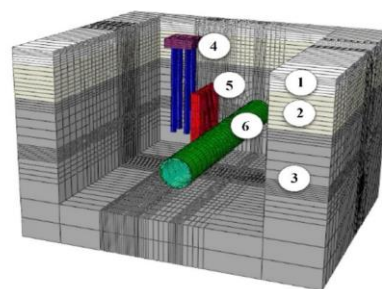
Model details: 1-plain filler layer; 2-silty clay layer; 3-clayey sandy gravel layer; 4-piles and piles cap; 5-jet grouted wall; 6-tunnel component
