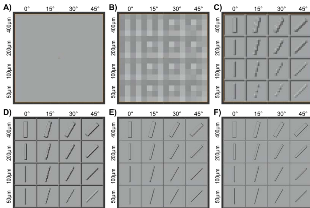
Figure 3. Effect of the mesh width on the appearance of the test part surface with the projected test image. A) No subdivisions, B) subdivided four times, and C) subdivided six times. In addition to the six subdivisions, a subdivision surface modifier was added and set to a viewport level of D) 1 level, E) 3 levels, and F) 5 levels. Surface shown in solid view.
