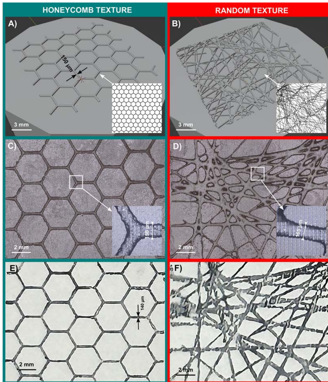
Figure 7. 3D mesh model of a stamp with A) a regular (honeycomb) texture and B) a random texture, with the imported image shown in the respective inset image. Confocal panoramic image (5x) of the 3D printed stamp surface for C) the honeycomb texture and D) the random texture, with a magnified view (x20) of a selected detail in each inset image. Optical microscopy image of the obtained image on paper when using the stamp with E) the honeycomb texture and F) the random texture. Stamping was performed under a load of 450 g for 10 seconds.
