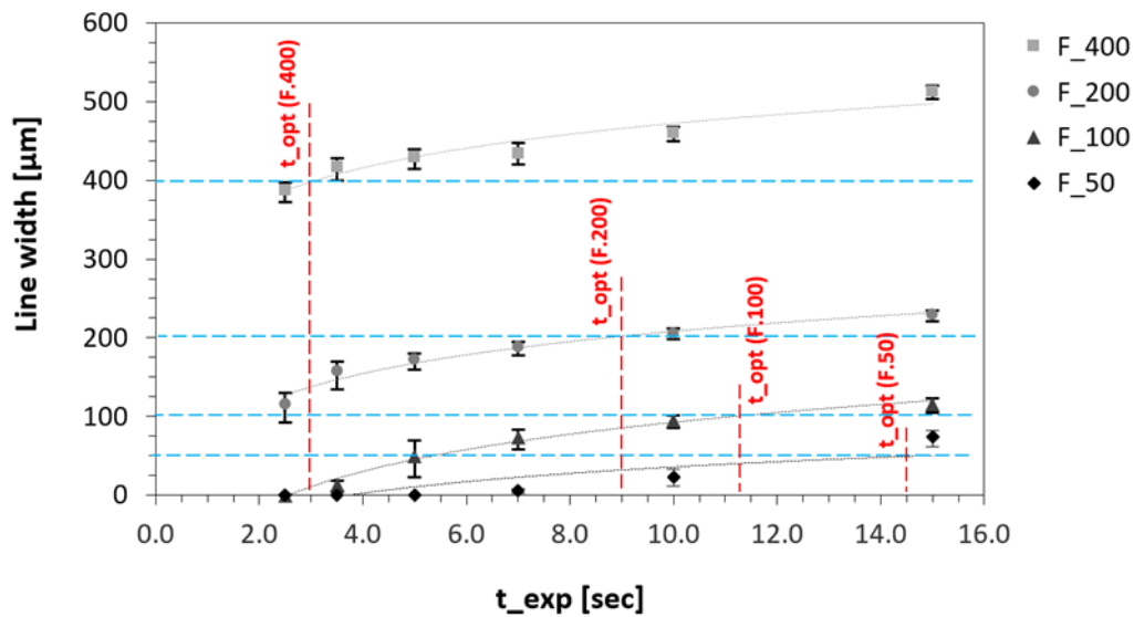
Figure 6. Effect of textured-layer exposure ( t_{\text{exp}} ) on actual width of the vertical line features.
