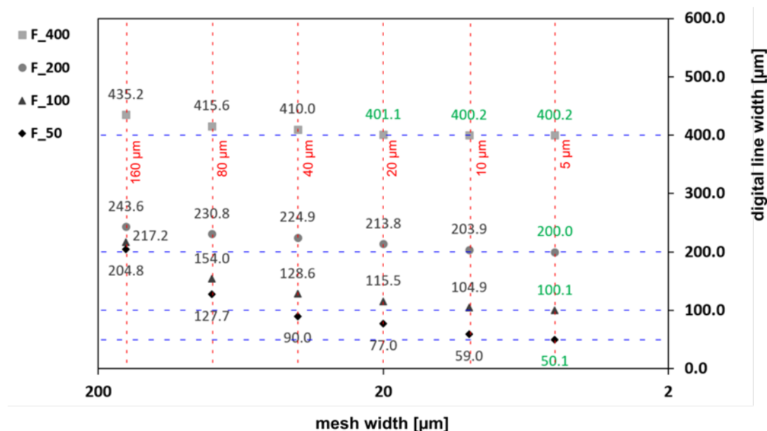
Figure 4. Effect of mesh width on digital line width in the 3D model. Line feature orientation of 0 degrees; nominal line width of 400, 200, 100, and 50 \mu\text{m} .
