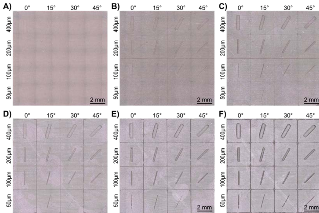
Figure 5. Confocal microscopy images of the textured surface exposed at A) 2.5 seconds, B) 3.5 seconds, C) 5.0 seconds, D) 7.0 seconds, E) 10.0 seconds, and F) 15.0 seconds per surface layer.
