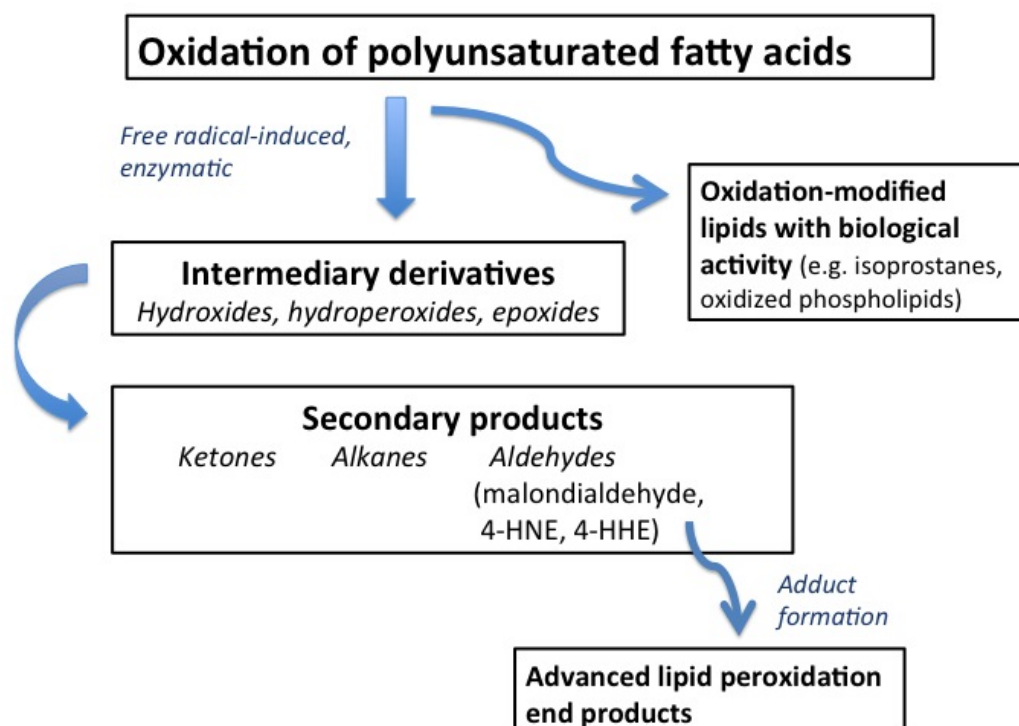
Figure 1. Formation of LOP during peroxidation of polyunsaturated fatty acids.
