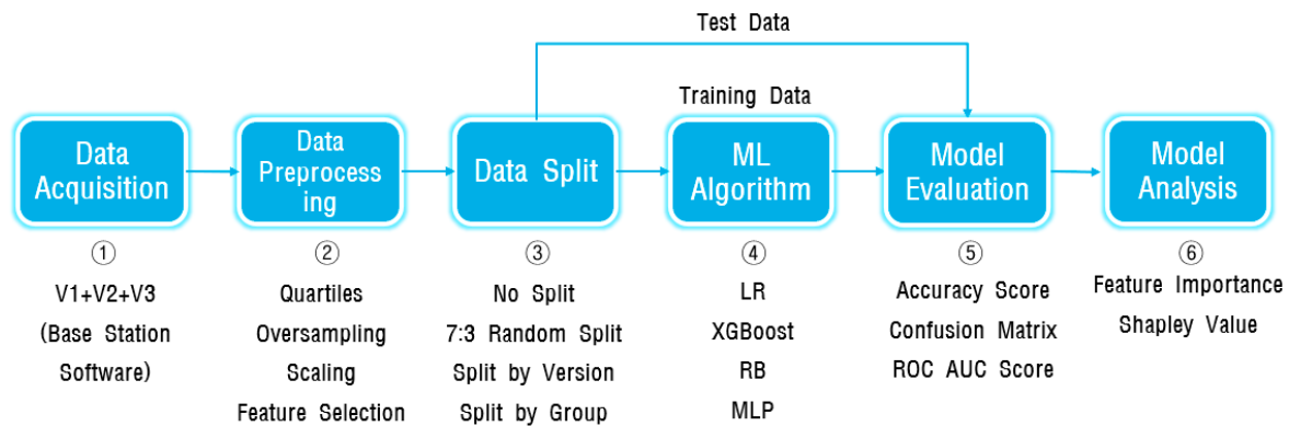
Figure 4. The experiments for developing the SDP model.
