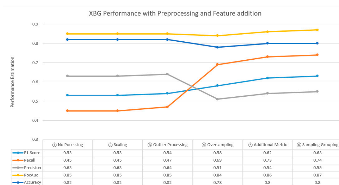
Figure 8. The changes in predictive performance due to data preprocessing and feature addition.
