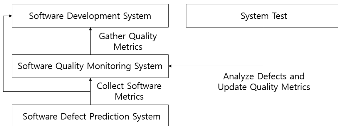
Figure 6. Update quality metrics based on defects from system test.
