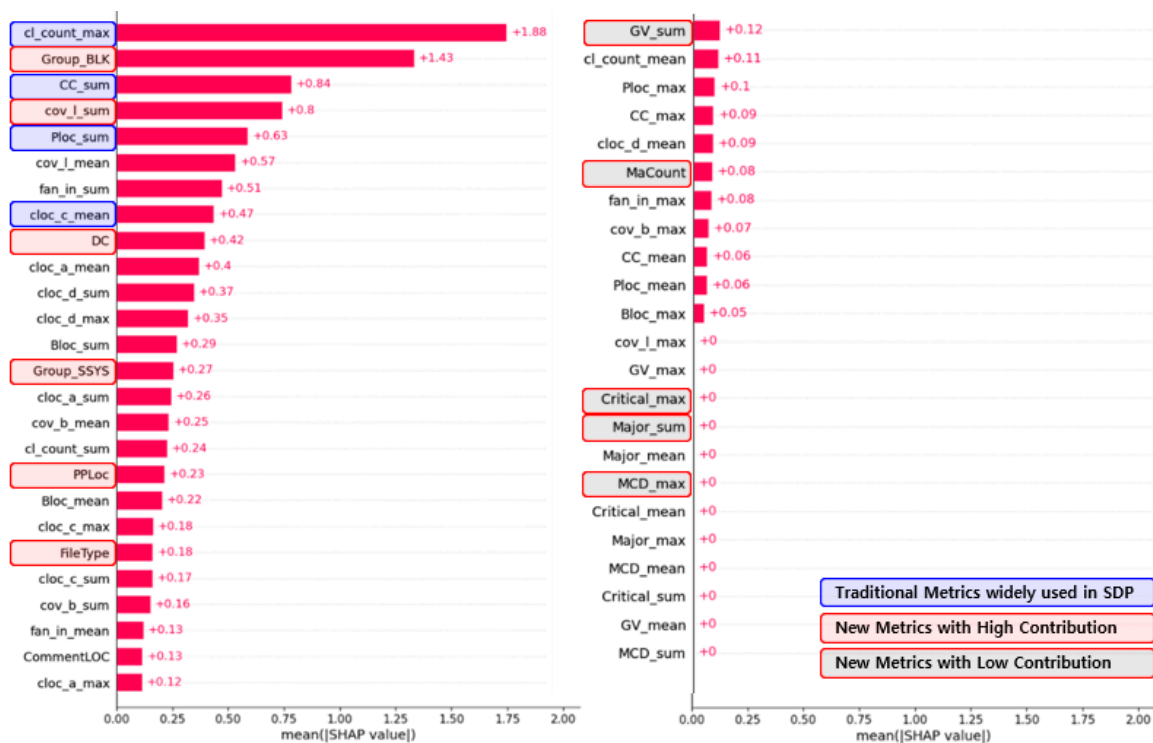
Figure 9. Shapley Value of XGB Model.
