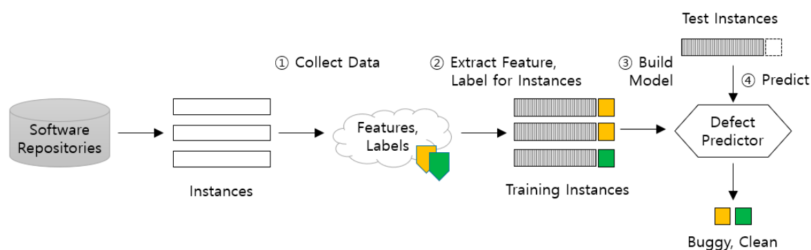
Figure 1. Machine Learning Based Software Defect Prediction (Revised).
