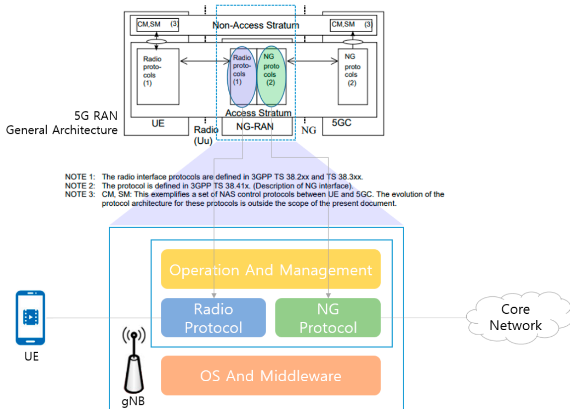
Figure 2. Software components of the base station software (Revised).
