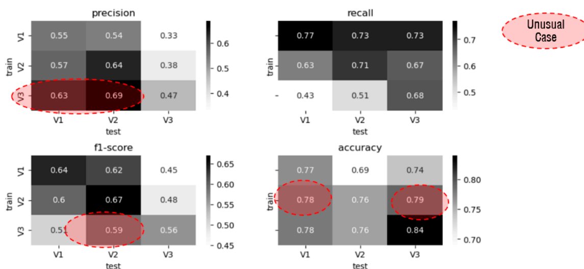
Figure 10. Prediction Performance under Cross-Version.
