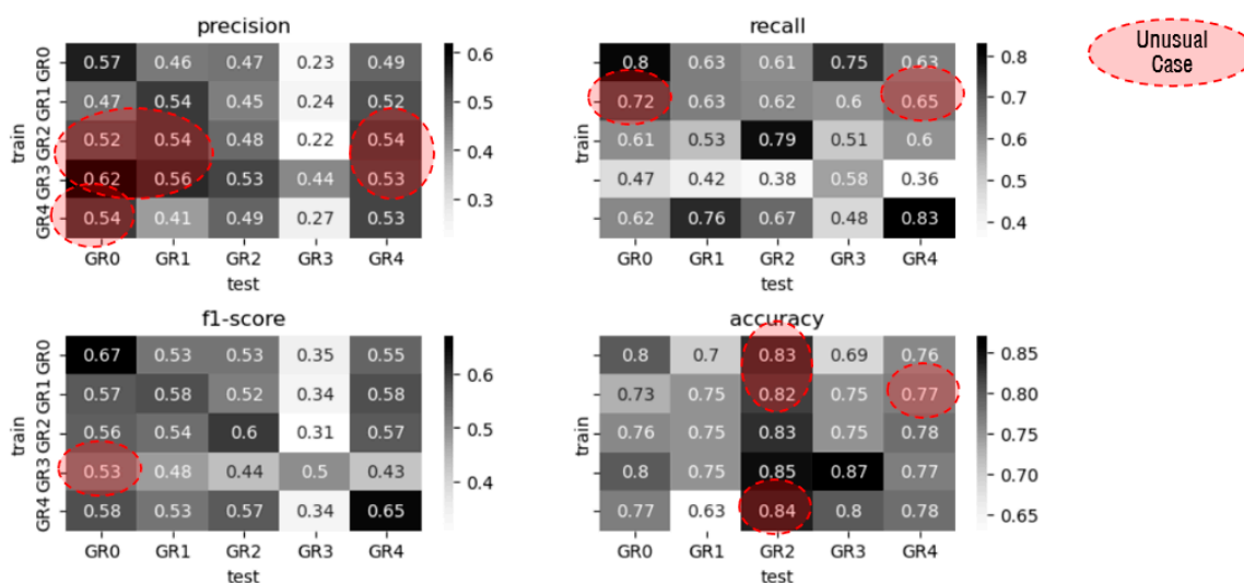
Figure 11. Prediction Performance under Cross-Group.
