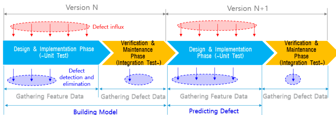
Figure 5. Data collection and defect prediction across versions.
