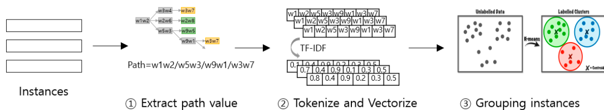
Figure 7. Grouping instances using TF-IDF and K-means (Revised).
