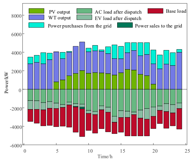
Figure 6. Power supply and demand equilibrium in Scenario 1.
