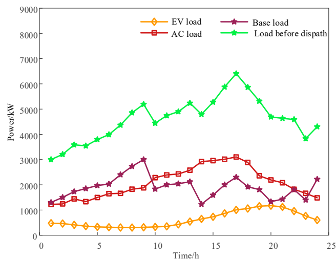
Figure 4. Load profile before the demand response.
