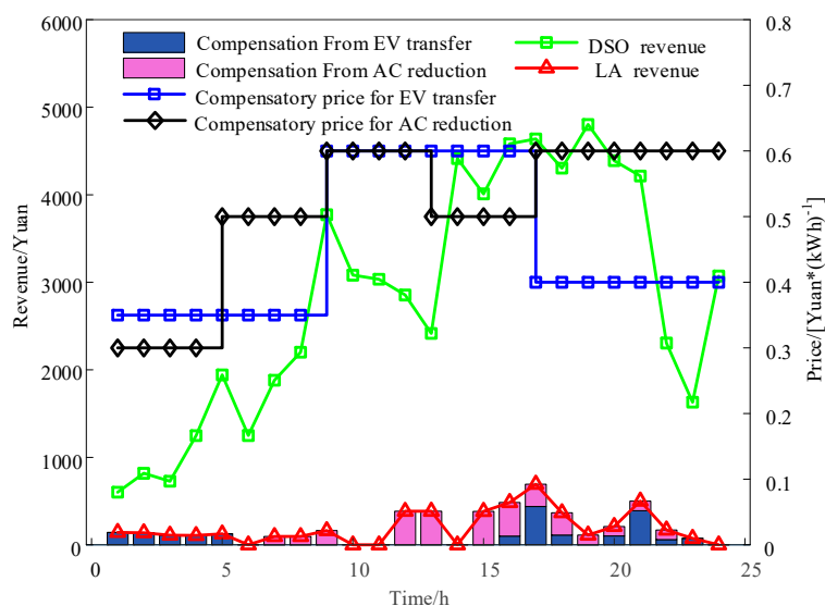
Figure 7. Postresponse DSO and LA gains at each time point.
