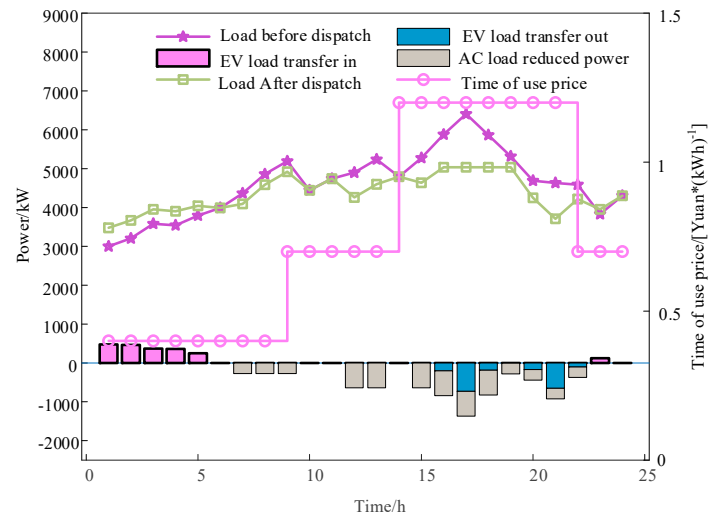
Figure 5. Comparison of the load before and after the response in Scenario 1.
