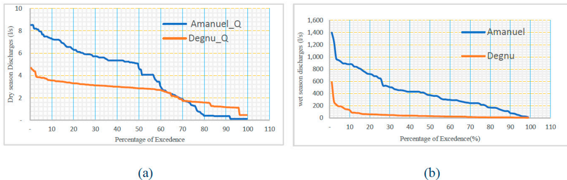
Figure 9. Flow duration curve of dry season (a) and wet season (b) of first year.
