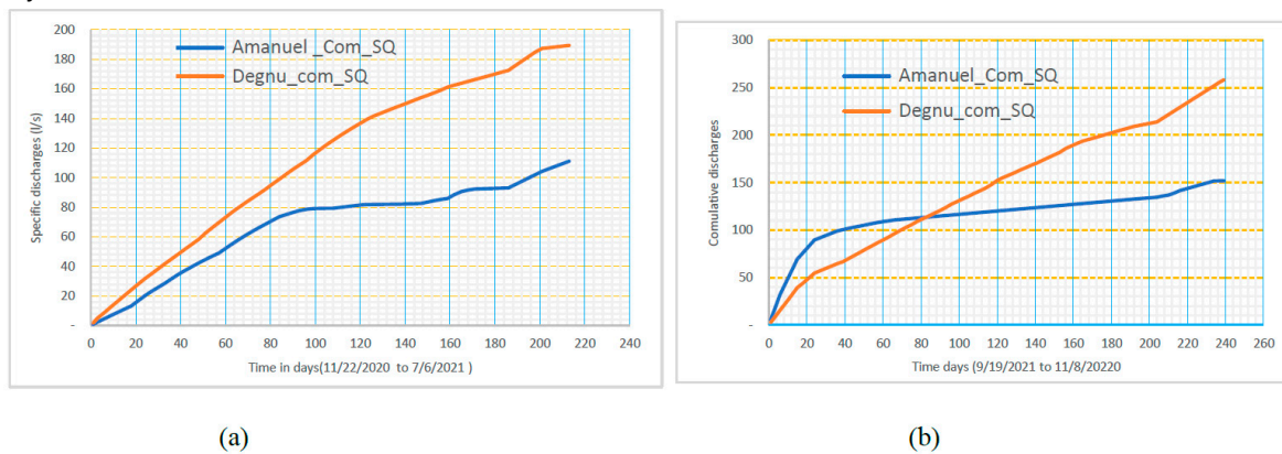
Figure 6. Cumulative Specific discharge of the dry season (a) first year and (b) second year.
