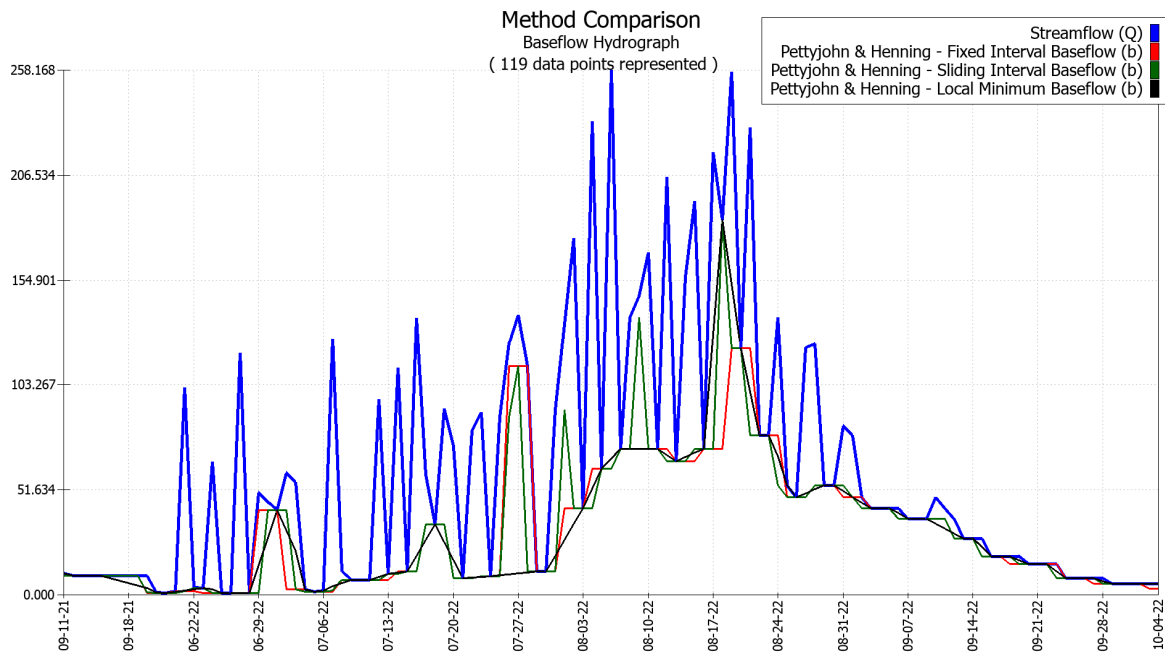
Figure 4. Base flow separation method comparison.
