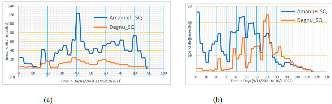
Figure 7. Specific Base flow pattern of the Wet season (a)first year (b)second year.
