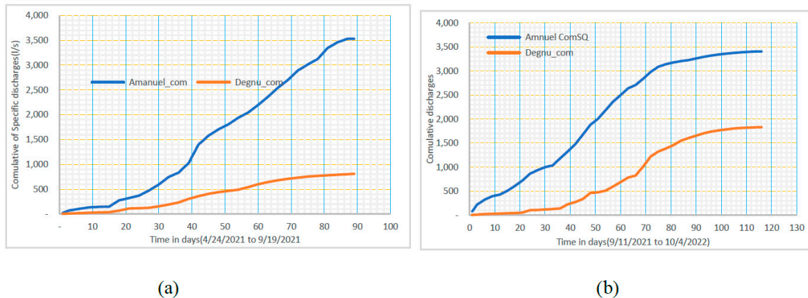
Figure 8. Specific Base flow pattern of the Wet season (a)first year (b)second year.
