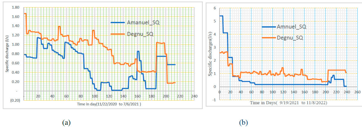
Figure 5. Specific Base flow patterns in the dry season (a) first year and (b) second year.
