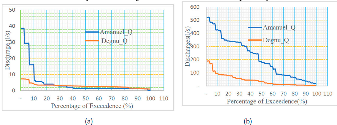
Figure 10. Flow duration curve of dry season (a) and wet season (b) of the second year.
