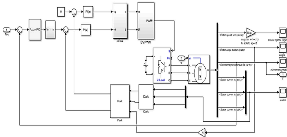
Figure 6. F-PID double closed-loop vector control system for PMSM.
