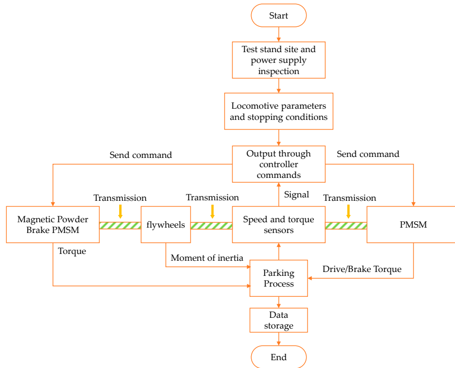
Figure 12. Experimental flow chart of test bench.
