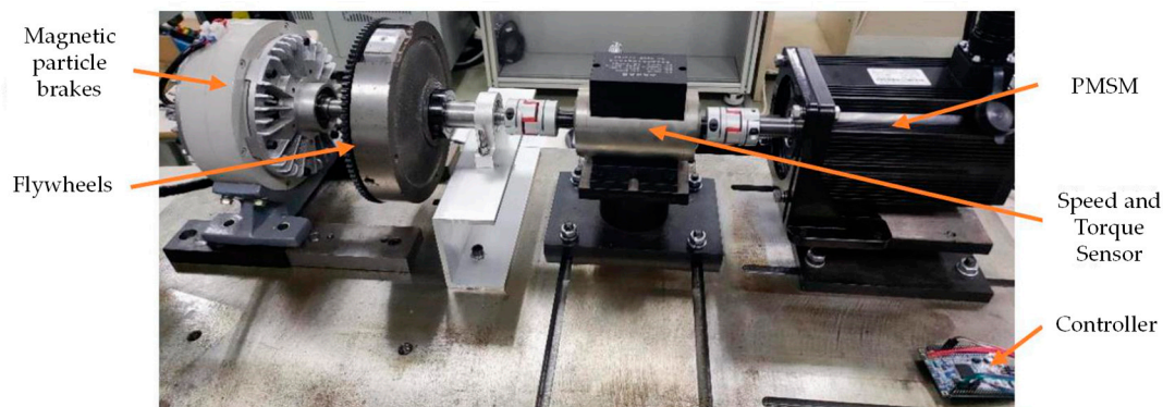
Figure 11. Experimental test bench.
