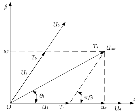
Figure 2. Linear combination of voltage space vector figure.
