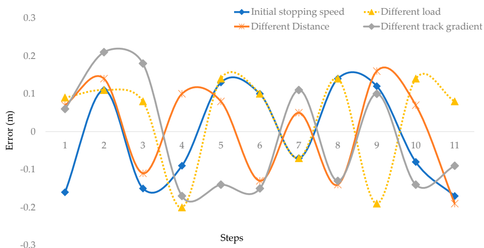
Figure 14. Exploring error variations in simulated working conditions.
