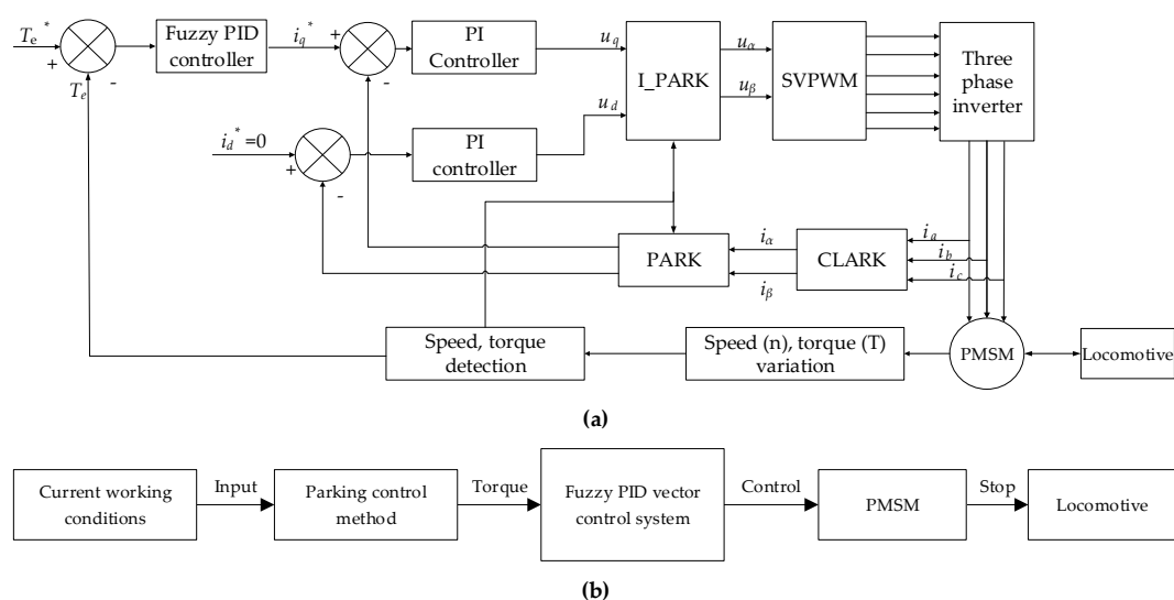
Figure 5. (a) F-PID control system, (b) Fuzzy PID vector control system in stopping control.
