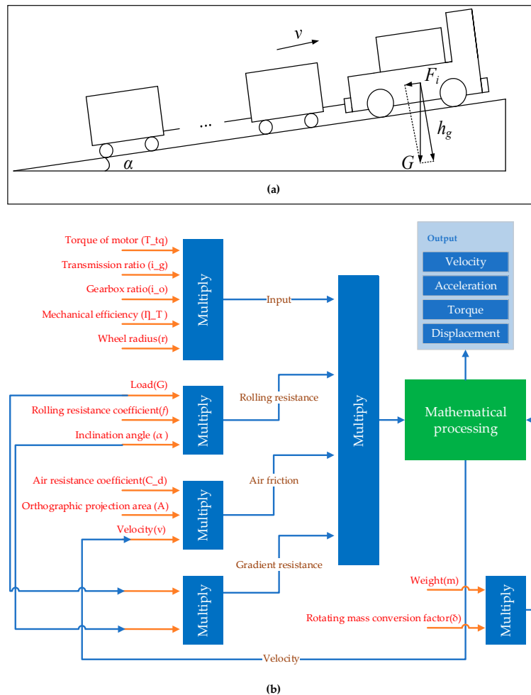
Figure 7. (a) Schematic diagram of gradient resistance of electric locomotive; (b) Schematic diagram of simulation flow in Simulink.
