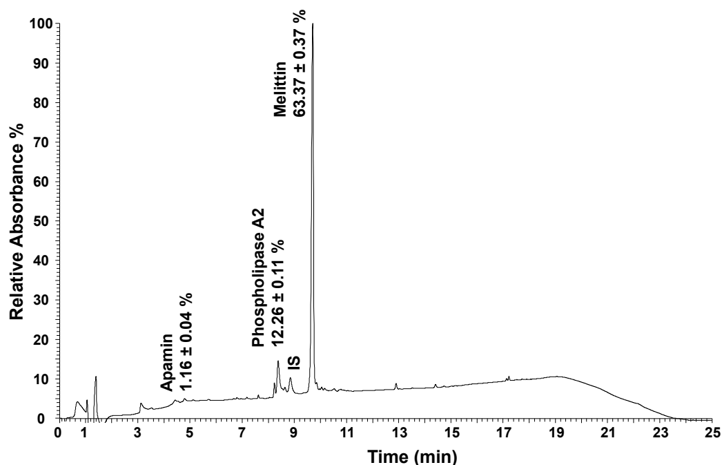
Figure 3. Example chromatogram after UHPLC analysis of the bee venom sample, at 220 nm. IS – internal standard (cytochrome C, 25 \mu\text{g/mL} ); UHPLC - ultra-high-performance liquid chromatography.
