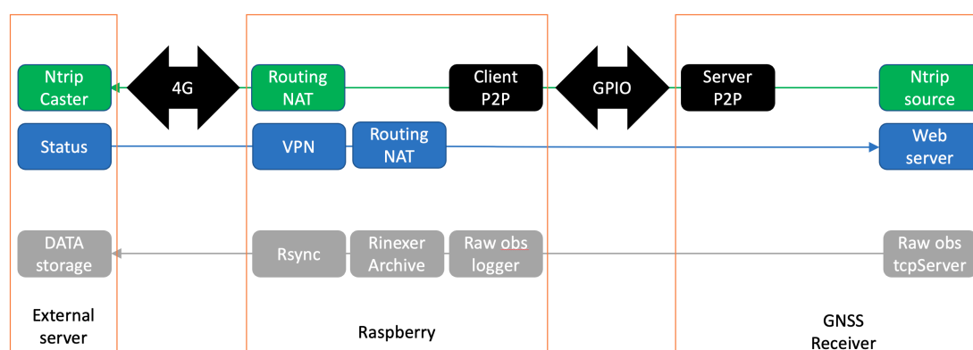
Figure 2. Flowchart implemented in Septentrio mosaic-X5 station prototype. 4G: Cellular modem. GPIO: General Purpose Port. Ntrip: Networked Transport of RTCM via Internet Protocol. VPN: Virtual Private Network. P2P: Point-two-Point. NAT: Network Address Translation.
