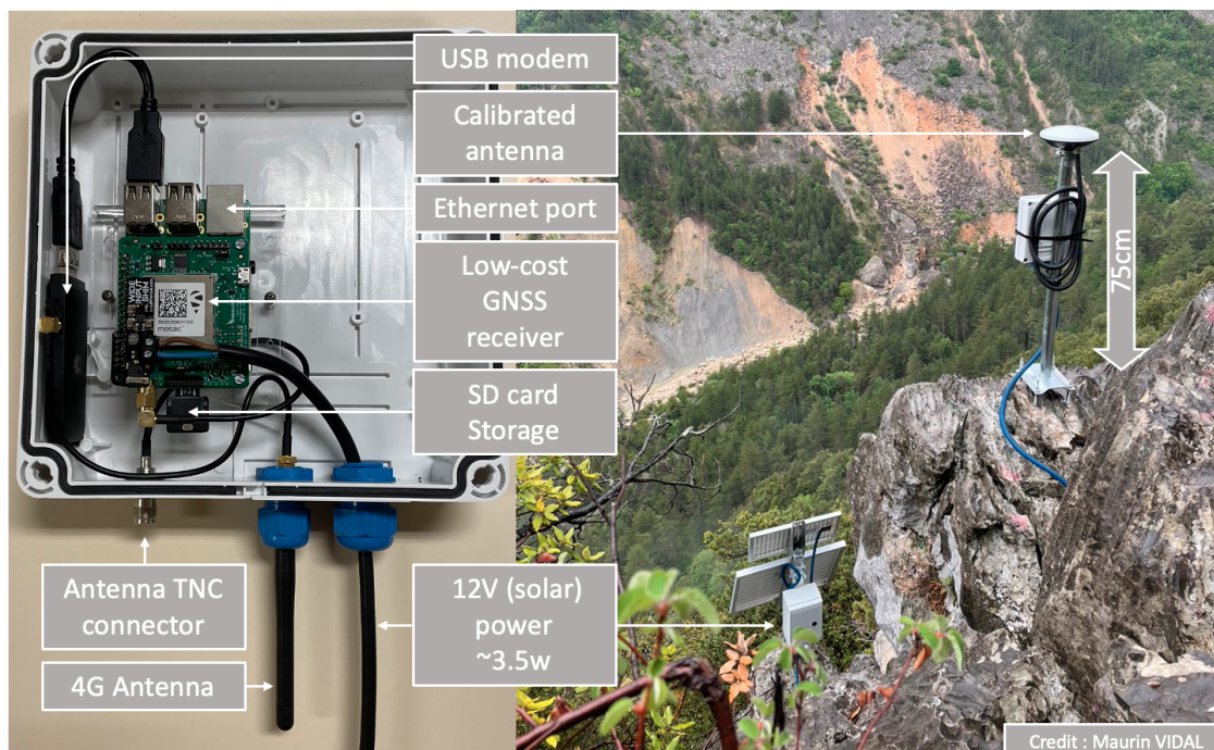
Figure 1. Ground-based GNSS field set-up using the Septentrio MOSAIC X5 receiver board in Briançonnet city in southern France, located \sim 35 km from the SOPH station. The left panel shows the in-house all-in-one dual-frequency low-cost receiver, while the right panel shows the antenna monument, anchored into bedrock, and the solar panel photovoltaic system.
