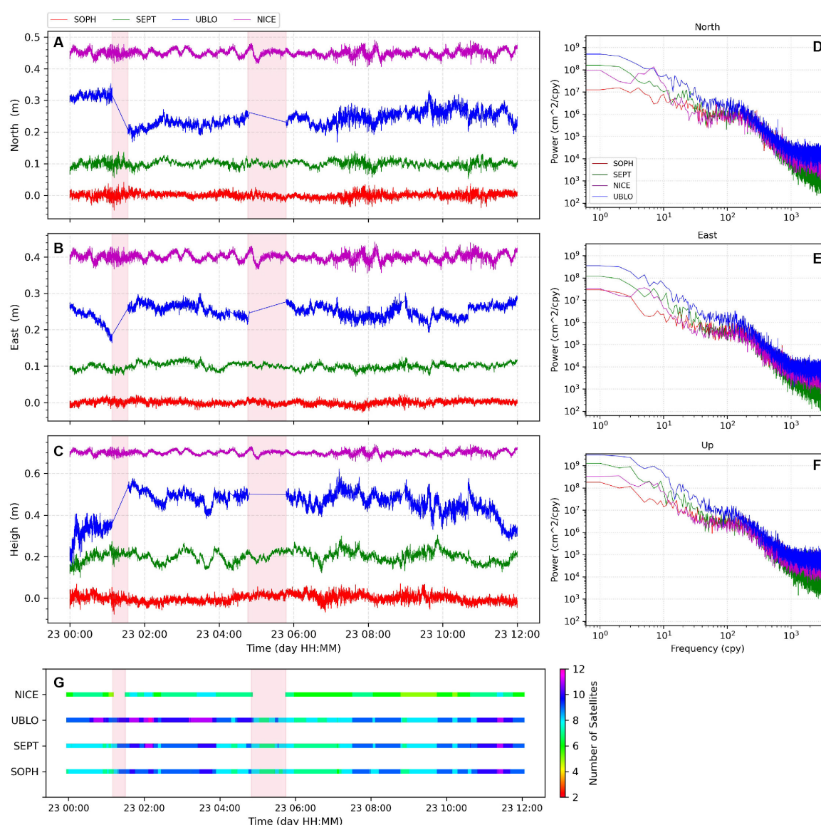
Figure 9. Kinematic displacement for the 1-second sampling rate at the NICE, SEPT, SOPH, and UBLO sites on July 23, 2023. A, B, and C panels depict the kinematic displacements for the GPS constellation. Detrended traces have been shifted to avoid overlap. Light pink vertical stripes within the left panels indicate the displacement gaps at the UBLO site. D, E, and F are the power spectral densities (PSD) estimated from the detrended kinematic displacements at NICE, SEPT, SOPH, and UBLO. G) Number of available satellites tracked by geodetic receivers from GPS observations at a 1-second sampling rate.
