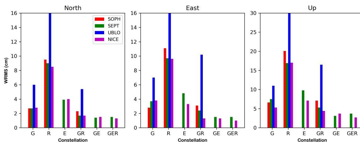
Figure 10. Repeatability (WRMS) computed from residual positions randomly selected (1 day par month) for the GNSS kinematic processing. The x-axis depicts the GNSS solution according to the selected constellation. G: GPS, R: GLONASS, E: Galileo, GR: GPS-GLONASS, GE:GPS-Galileo, GRE: GPS-GLONASS-Galileo
