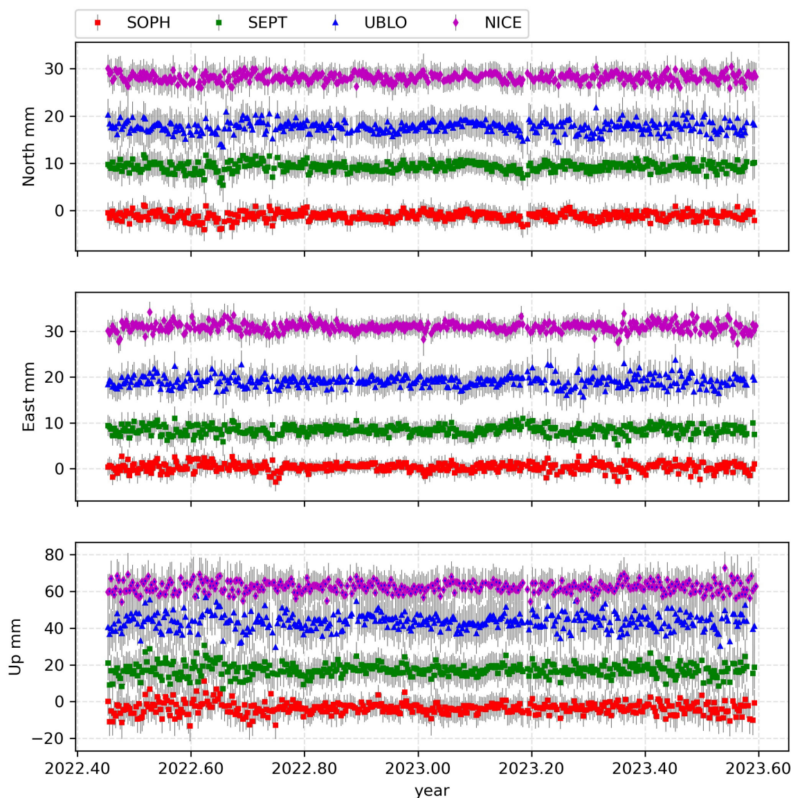
Figure 6. Detrended daily position time-series with associated uncertainties (gray bars) for the SEPT, UBLO, SOPH, and NICE GNSS sites using Gamit-Globk software. Time series are therefore solutions for the GPS constellation.
