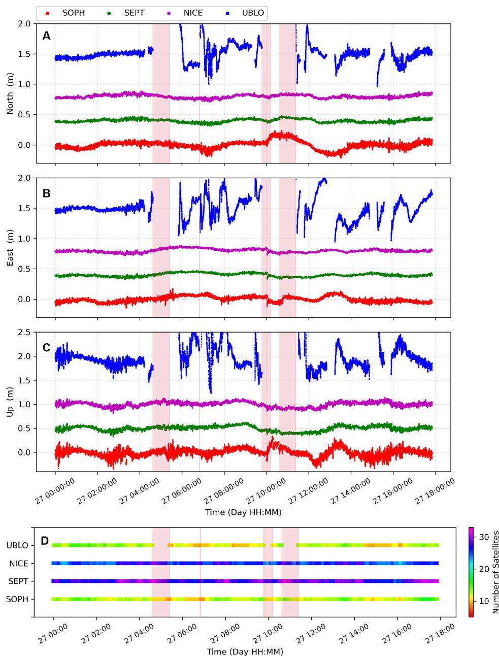
Figure 11. Kinematic displacements from the real-time analysis at the SOPH, SEPT, NICE, and UBLO stations for the North (A), East (B), and Vertical (C) components on September 27, 2023. D) Number of available satellites tracked by geodetic receivers from GNSS observations at a 1-second sampling rate. For visualization purposes, displacements greater than 0.8 m in the UBLO solution are not shown in the comparison. Light pink vertical stripes depict gaps in the kinematic solution and the loss of satellite tracking capacities of the UBLO receiver.
