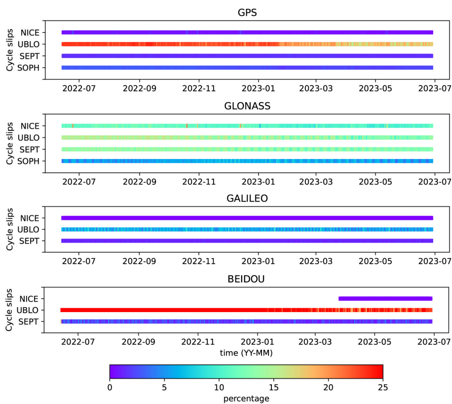
Figure 4. Daily cycle slip values estimated at the SEPT, UBLO, and SOPH sites for the GPS and GLONASS constellations (SEPT and UBLO shared antenna is 5 m apart from SOPH antenna, table 1). In order to assess the quality of the low-cost stations for the Galileo and BeiDou constellations, we have also included the NICE station, located 20 km away, in the comparison. BeiDou GNSS observations on the NICE site started after the last receiver replacement on March, 2023.
