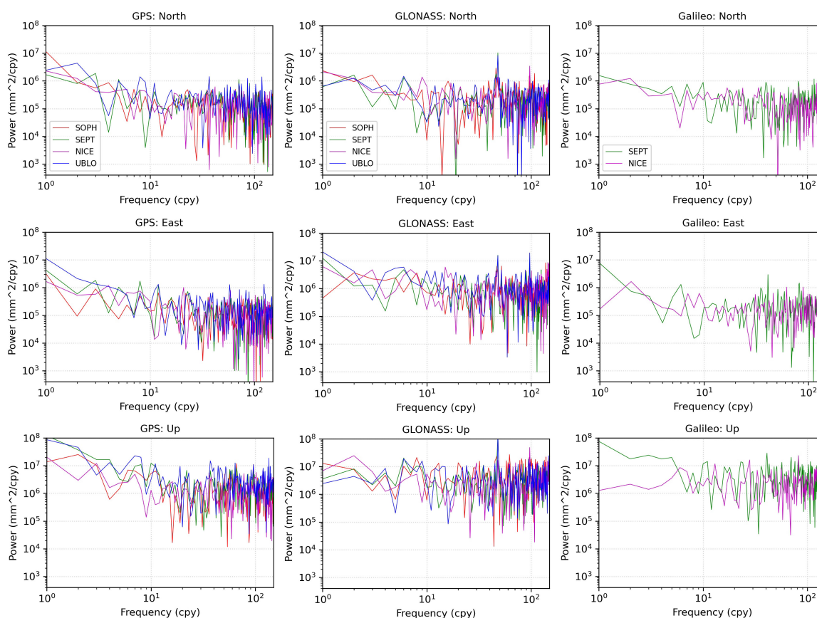
Figure 8. Power Spectral Densities (PSD) for the NICE, SOPH, SEPT and UBLO GNSS sites. PSD are computed for the GPS, GLONASS, and Galileo constellations using the CATS software [25]. cpy: cycles per year.
