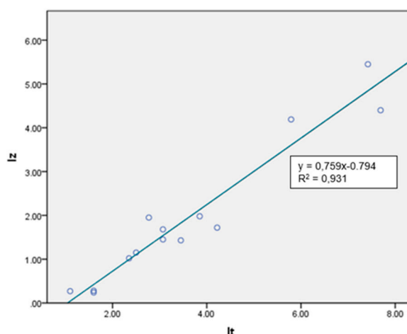
Figure 10. Pearson's correlation coefficient between slope of siltation ( I_z ) and natural bed slope ( I_t ).
