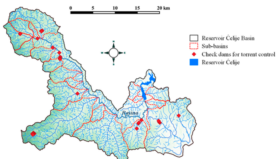
Figure 6. Hydrographic map with existing check dams.
