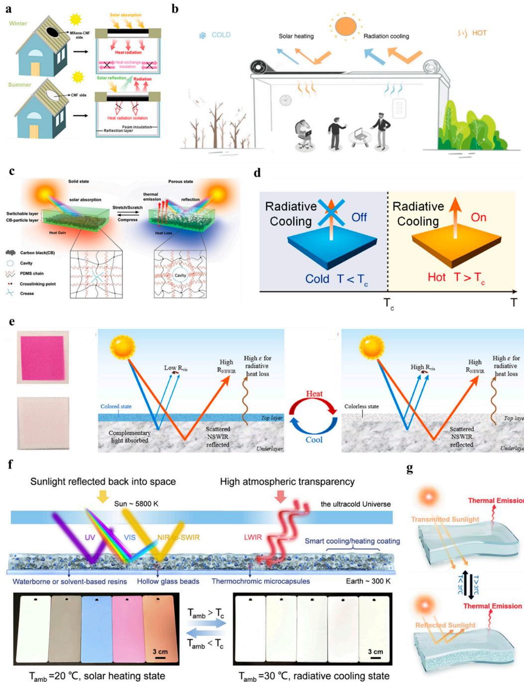
Figure 4. Adaptive radiative cooling design. a) Schematic of an engineering structural Janus MXene/CNF aerogels. Figure by [55] is licensed under CC BY-NC 4.0, with the permission of John Wiley and Sons. b) Schematic of the dual-mode device at heating (left) mode and cooling (proper) mode. [56] is licensed under CC BY-NC 4.0. c) Schematic of the bilayer structure consisting of a switchable silicone top layer and carbon black particle-embedded bottom layer. Figure by [19] is licensed under CC BY-NC 4.0, with the permission of John Wiley and Sons. d) Concept of a temperature-dependent adaptive radiative cooler containing \text{VO}_2 . [57] is licensed under CC BY-NC 4.0. e) Schematic of a low-cost and scalable temperature adaptive radiation-cooling coating Reprinted from [47,65], with permission from Elsevier [OR APPLICABLE SOCIETY COPYRIGHT OWNER]. f) Schematic of a \text{TiO}_2 -free coating with self-adaptive switching between cooling. Reprinted from [47,66], with permission from Elsevier [OR APPLICABLE SOCIETY COPYRIGHT OWNER]. g) Schematic
