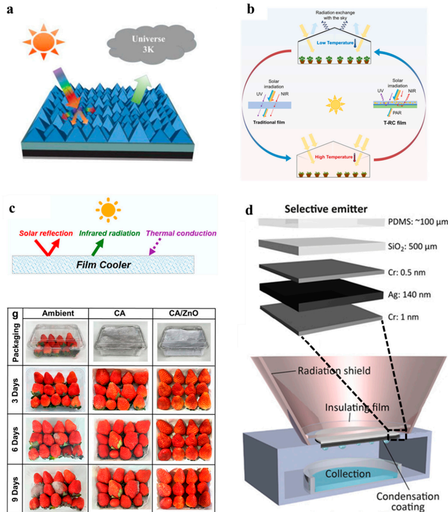
Figure 6. Other applications of radiative cooling. a) Schematic of the imprinted texture glass used in PV modules. Figure by [96] is licensed under CC BY-NC 4.0, with the permission of John Wiley and Sons. b) Schematic diagram for greenhouse temperature regulation using radiative cooling film. Reprinted from [103], with permission from Elsevier [OR APPLICABLE SOCIETY COPYRIGHT OWNER]. c) Cooling of strawberries via the hierarchically designed CA/ZnO film. Reprinted (adapted) with permission from [109]. Copyright 2024 American Chemical Society. d) Design of 24-hour atmospheric water harvesting system driven by radiative cooling. From [126]. Reprinted with permission from AAAS.
