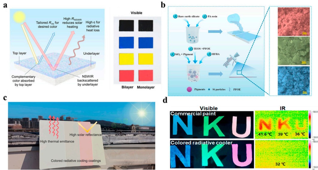
Figure 3. Colored radiative coolers. a) Bilayer colored radiative coolers for enhanced NSWIR reflectance. From [46]. Reprinted with permission from AAAS. b) The schematic of colorful radiative cooling emitters. Reprinted from [47], with permission from Elsevier [OR APPLICABLE SOCIETY COPYRIGHT OWNER]. c) Colored radiative cooling coatings using phosphor dyes. Reprinted from [47,48], with permission from Elsevier [OR APPLICABLE SOCIETY COPYRIGHT OWNER]. d) Photonic-Structure Colored Radiative Coolers. Reprinted (adapted) with permission from [53]. Copyright 2024 American Chemical Society.
