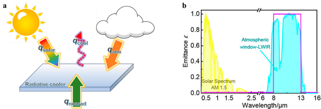
Figure 1. Fundamentals of passive radiative cooler. a) Schematic diagram of the heat transfer processes of a typical passive radiative cooler. b) The ideal solar reflectivity and MIR emissivity of daytime passive radiative cooling.
