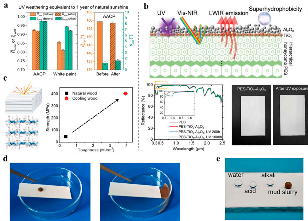
Figure 2. High durability radiative cooler design. a) The almost unchanged optical and wetting properties of AACP coating after 1000 h of UV exposure. [41] is licensed under CC BY-NC 4.0. b) Cross-sectional schematic of the trilayer PES-TiO 2 -Al 2 O 3 cooler and its UV resistance capability. Figures by [42] is licensed under CC BY-NC 4.0, with the permission of John Wiley and Sons. c) Schematic diagram of the cooling wood structure and its strength comparison with ordinary wood. [43] is licensed under CC BY-NC 4.0. d) Photograph of a mud slurry droplet on a PS/PDMS/PECA coating. Reprinted (adapted) with permission from [44]. Copyright 2024 American Chemical Society. e) Photograph of the spherical droplets of water, acid, alkali, and mud slurry on the coating. Reprinted from [45], with permission from Elsevier [OR APPLICABLE SOCIETY COPYRIGHT OWNER].
