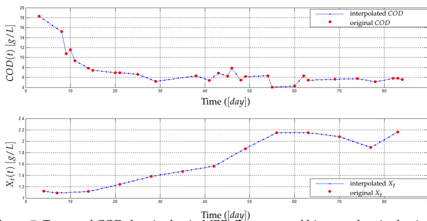
Figure 7. Top: total COD data in the AnMBR. Bottom: total biomass data in the AnMBR.
