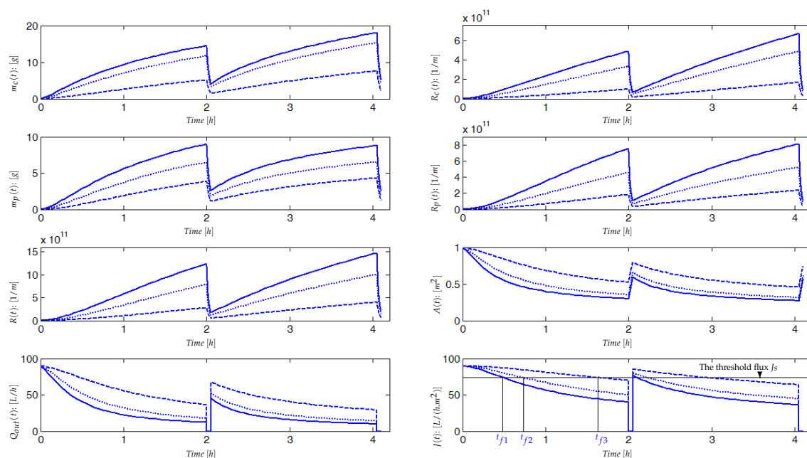
Figure 5. Simulation results of the membrane fouling model for both phases (filtration and backwash), with values of C_s , C_x , C_{smp} equal to : 0.1 (—) ; 0.4 (- - -) ; 0.7 (⋯⋯).
