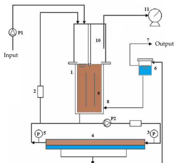
Figure 6. Schematic diagram of the AnMBR installed at CBS for the municipal and abattoirs wastewater treatment. 1: Anaerobic reactor, 2: Flow-meter, 3 Manometer, 4: Ultra-filtration membrane, 5: Manometer, 6: Permeate tank, 7: Permeate output, 8: Permeate recycling, 9: Column, 10: Tube, 11: Gas-meter. [33]
