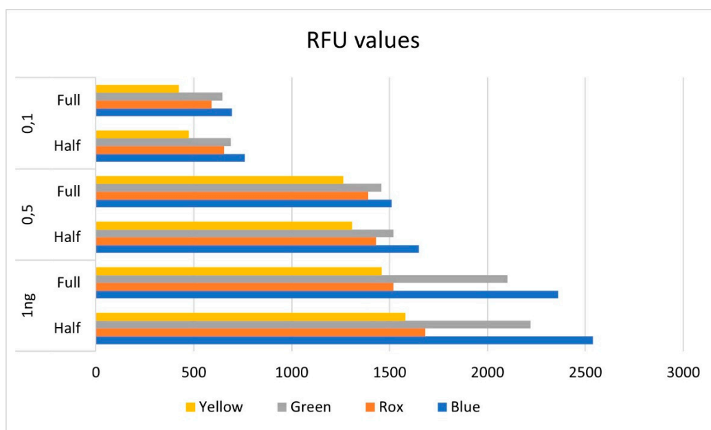
Graf. 1: Average RFU values for each dye channel for different DNA quantity.
