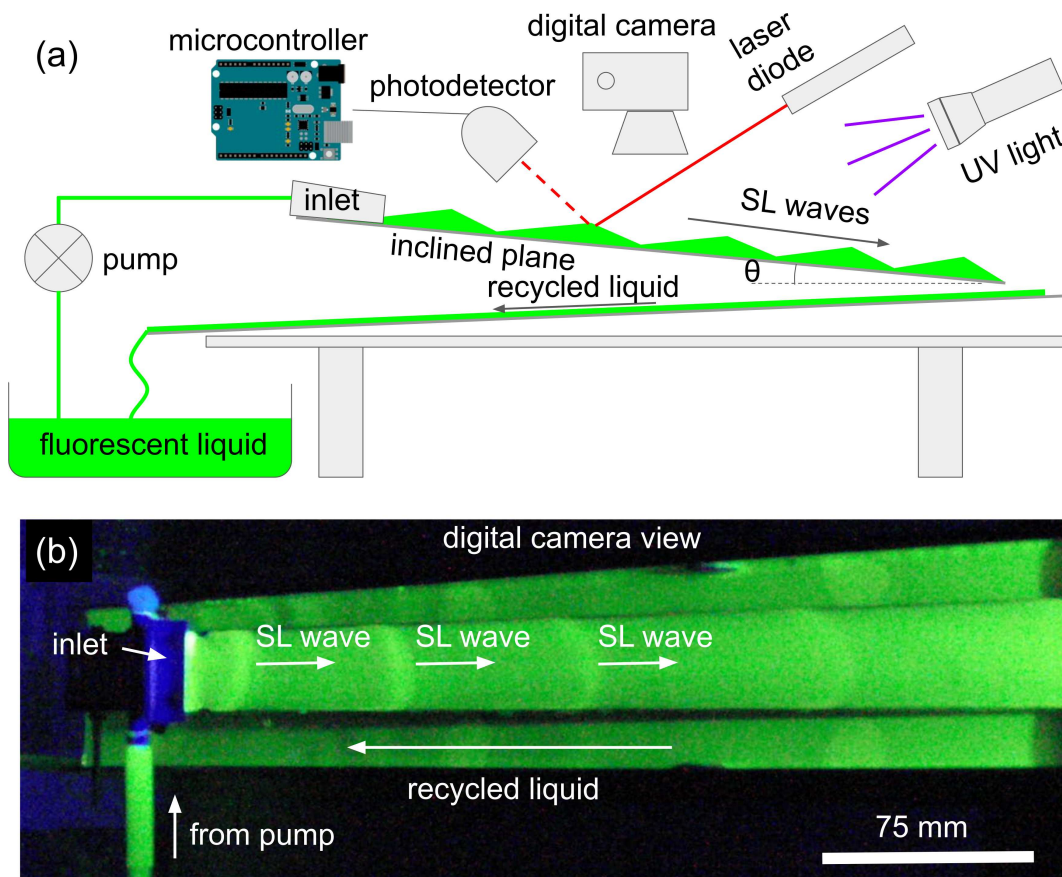
Figure 2. (a) Sketch and (b) top view fluorescence photograph of the experimental setup used to validate the proposed architecture of the physical RC system. The fluorescent dye, UV light and digital camera play an auxiliary role and can be removed from the setup without compromising its operation. The remaining components of the setup are controlled by an Arduino microcontroller that is also used to process the raw data traces.
