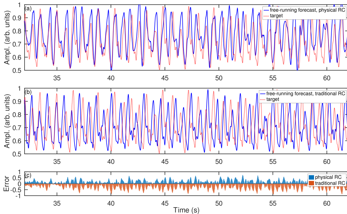
Figure 5. Generative mode operation (free-running forecast) of (a) physical RC system based on SL waves and (b) traditional algorithmic RC system (the solid curve) compared with the target MGTS (the dotted curve). (c) Modulus of absolute error of the forecasts produced by the physical and traditional RC algorithmic systems. Note that for the sake of comparison the error of the traditional RC system is plotted with the negative sign.
