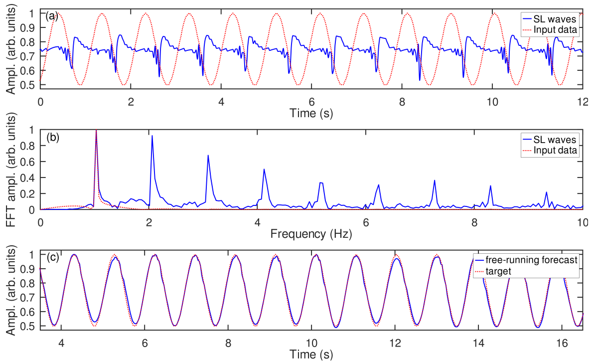
Figure 3. (a) Input sinusoidal signal (the dotted curve) and the SL waves excited by it (the solid curve). (b) Fourier spectra of the signals in Panel (a). (c) Free-running forecast of the future evolution of the sinusoidal waves made by the RC system based on the SL waves. Note that the timescale in Panel (c) is unrelated to that in Panel (a).
