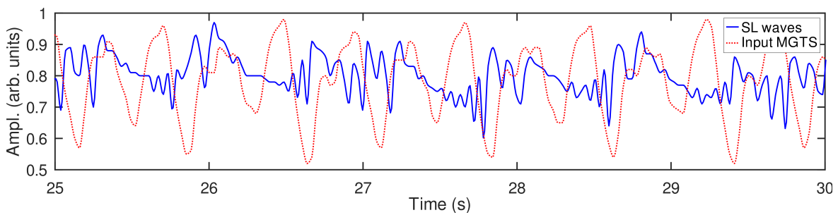
Figure 4. Input MGTS signal (the dotted curve) and the SL waves excited by it (the solid curve). Unlike in Figure 3a, since each variation of MGTS results in the generation of SL waves with different amplitude and propagation speed, the SL waves collide and form more complex wave profiles.
