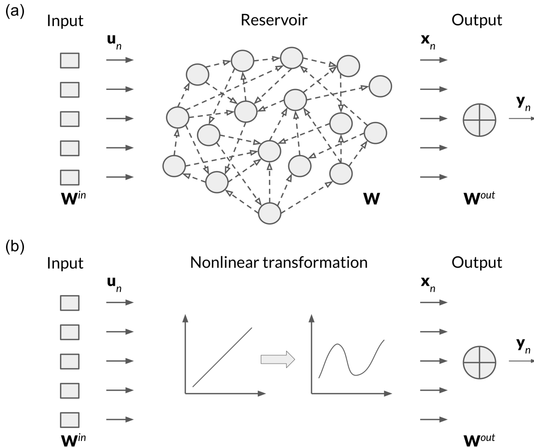
Figure 1. Schematic representation of (a) a traditional algorithmic RC system and (b) an RC system with a reservoir of random connection substituted by a nonlinear functional of the input data.
