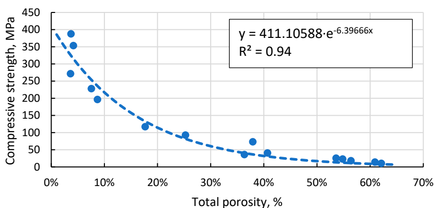
Figure 13. Dependence of compressive strength on total porosity of sintered samples.
