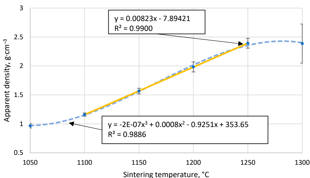
Figure 4. The apparent density of CS 63-150 \mu\text{m} samples sintered in a 20 mm mould as a function of sintering temperature.
