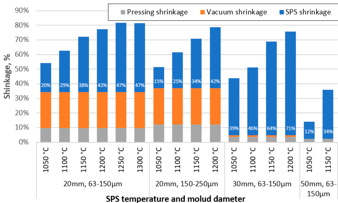
Figure 3. Shrinkage of specimens after squeezing, vacuum and SPS process steps, depending on sintering temperature, material used and die diameter.
