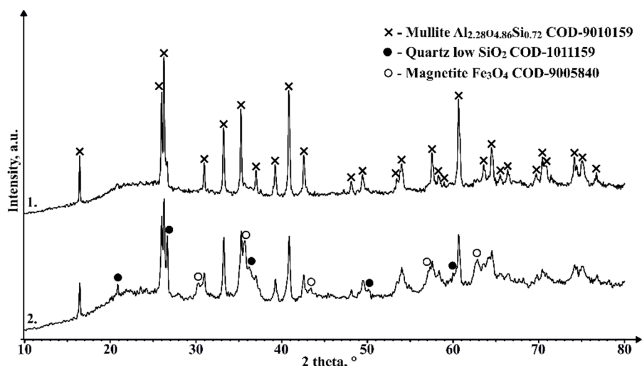
Figure 14. XRD results of magnetic CS 150-250 \mu\text{m} fraction (1), and magnetic particle concentrate from that same fraction (2).
