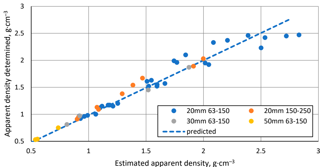
Figure 5. Relationship between predicted and observed apparent density of samples.
