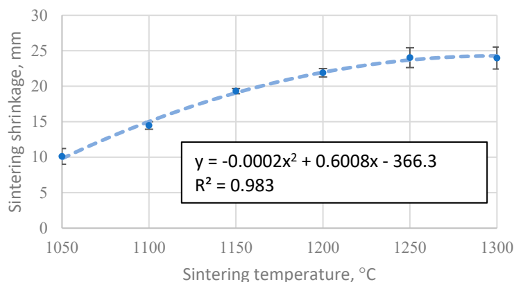
Figure 1. Shrinkage of CS 63-150 \mu\text{m} samples sintered in a 20 mm mould during the SPS process as a function of sintering temperature.
