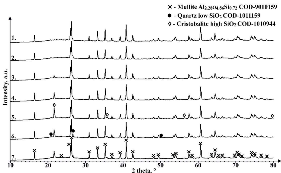
Figure 15. XRD results of unsintered CS2 63-150 \mu\text{m} (1), and samples sintered in 20mm mould for 2 minutes at 1050 ^{\circ}\text{C} (2), 1100 ^{\circ}\text{C} (3), 1150 ^{\circ}\text{C} (4), 1200 ^{\circ}\text{C} (5), 1250 ^{\circ}\text{C} (6) and 1300 ^{\circ}\text{C} (7).
