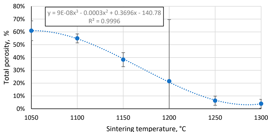
Figure 8. Total porosity of CS 63-150 \mu\text{m} samples sintered in a 20 mm die as a function of sintering temperature.
