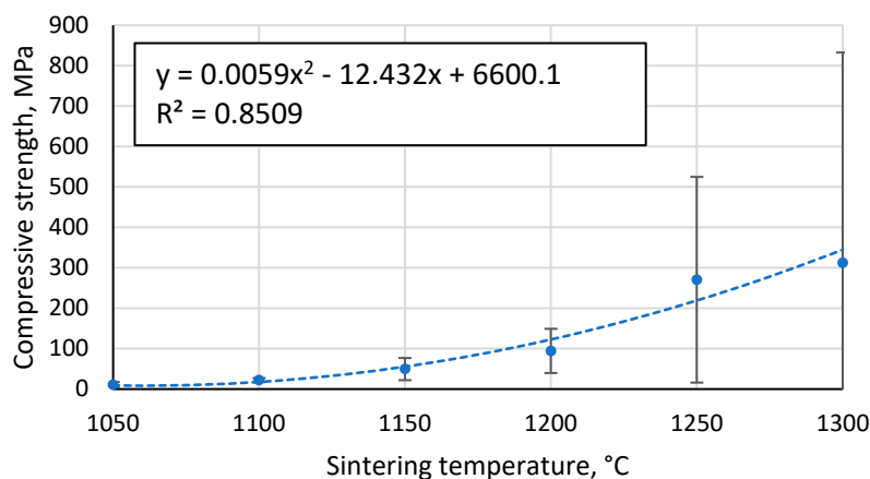
Figure 11. Compressive strength of sintered cenospheric specimens as a function of sintering temperature.
