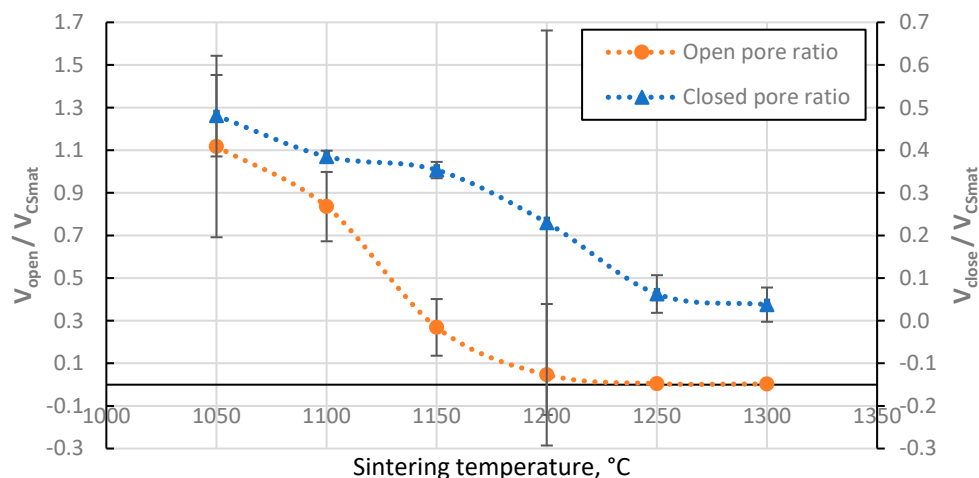
Figure 7. The ratio of closed and open pore volumes of sintered CS 63-150 \mu\text{m} samples to the volume of CS material volume (aluminosilicate only, excluding voids) as a function of sintering temperature.
