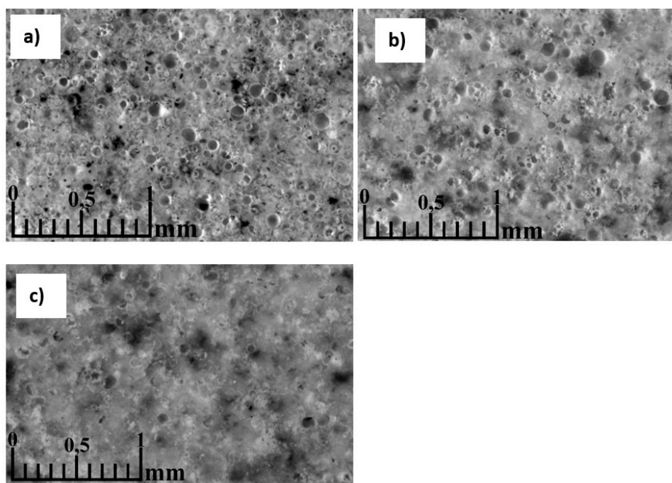
Figure 9. Optical microscopy image of CS 63-150 \mu\text{m} samples sintered in a 20 mm mould at 1050 °C (a), 1200 °C (b), 1250 °C (c), perpendicular to the die axis.
