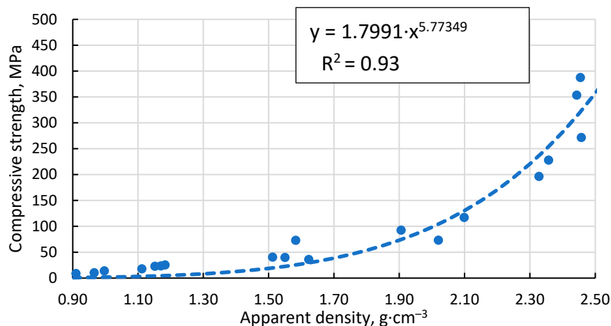
Figure 12. Dependence of compressive strength on apparent density of sintered specimens.
