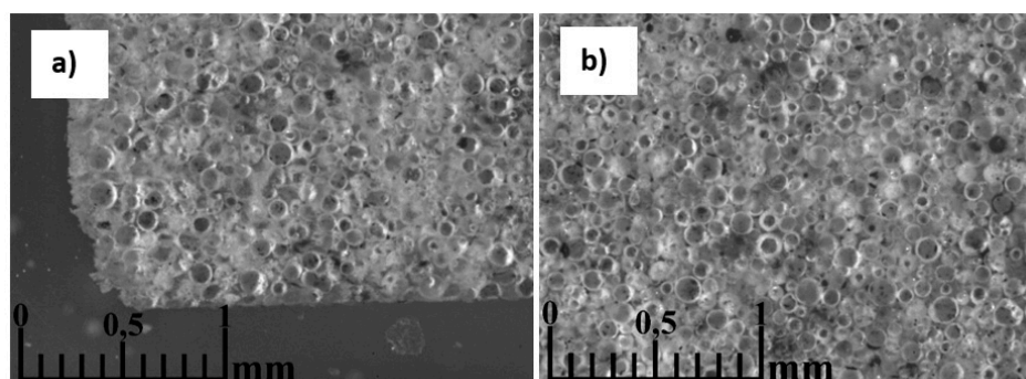
Figure 10. Optical microscopy images of a CS 63-150 \mu\text{m} sample sintered at 1050 ^{\circ}\text{C} in a 50 mm mould, parallel to the die axis, close to the material-mould boundary (a), and near the centre of the specimen (b).
