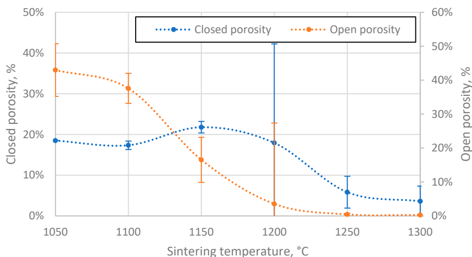
Figure 6. Open and closed porosity of CS 63-150 \mu\text{m} samples sintered in 20 mm mould as a function of sintering temperature.
