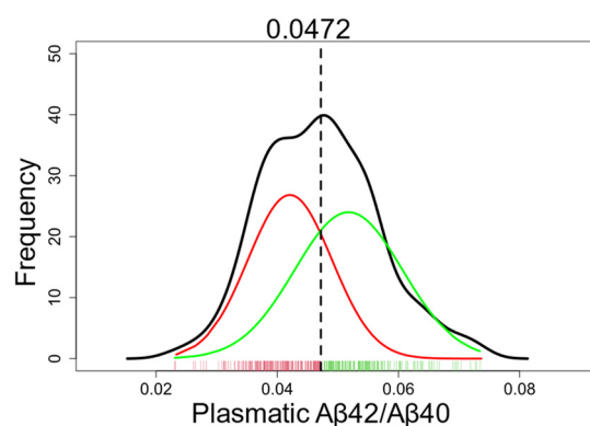
Figure 1. The full distribution of the plasma A \beta 42/A \beta 40 ratio is shown in black. This distribution was then approximated as two gaussians, represented in red (plasmatic A \beta +) and green (plasmatic A \beta -). Each tick on the x-axis represents one individual. The threshold at the intersection of the two gaussians is 0.0472.
