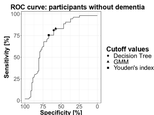
Figure 3. ROC curve representing the sensitivity and specificity of the plasma A \beta 42/A \beta 40 ratio for different cutoff values, calculated on participants without dementia. The cutoff values obtained by GMM (0.0472) and decision tree (0.0465) are indicated on the curve, as well as the Youden's index (0.0450).
