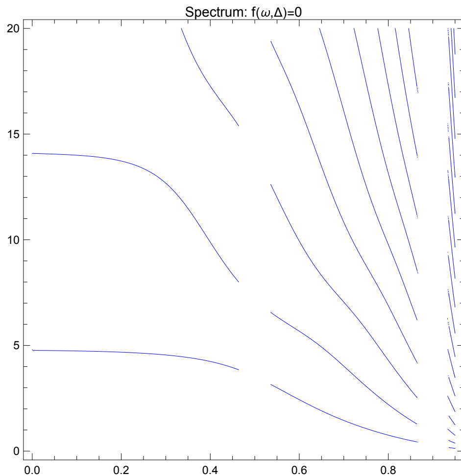
Figure 7. The first levels of the spectrum satisfying equation f(\omega, \Delta) = 0 . The broken lines correspond to the end of zones of real solutions.
