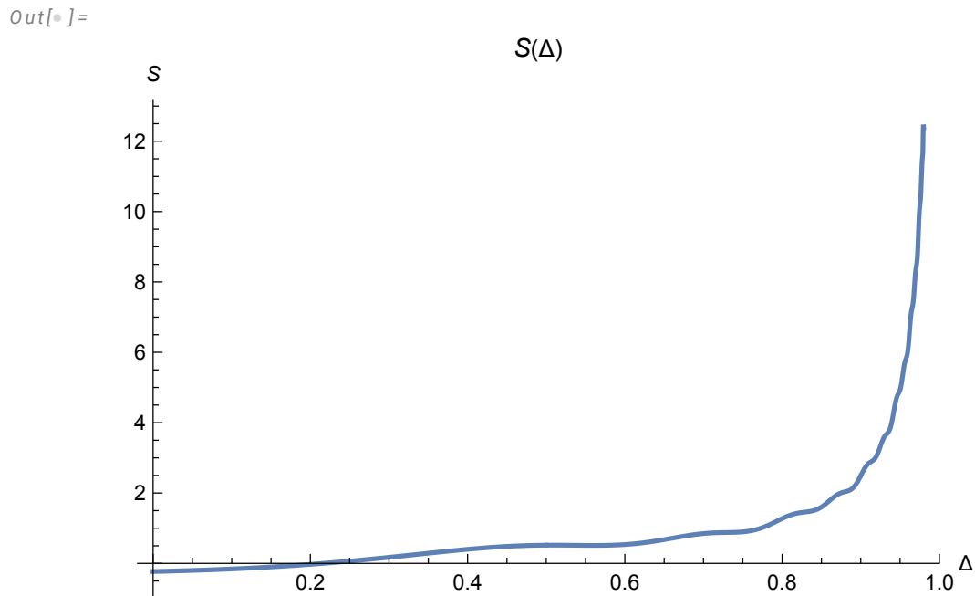
Figure 5. Plot of S(\Delta) .
