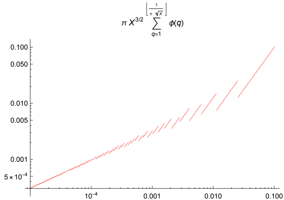
Figure 2. The log-log-plot of the distribution f_X(X) . It is equals \pi\Phi(k)X\sqrt{X} at each internal \frac{1}{\pi^2(k+1)^2} < X < \frac{1}{\pi^2k^2} with positive integer k . Asymptotically f_X(X) \rightarrow \frac{3\sqrt{X}}{\pi^3} at X \rightarrow 0 .
