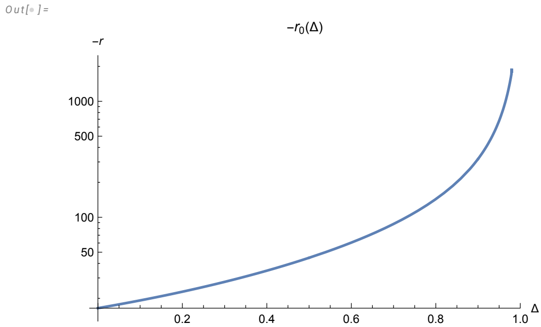
Figure 3. Log plot of -r_0(\Delta) .
