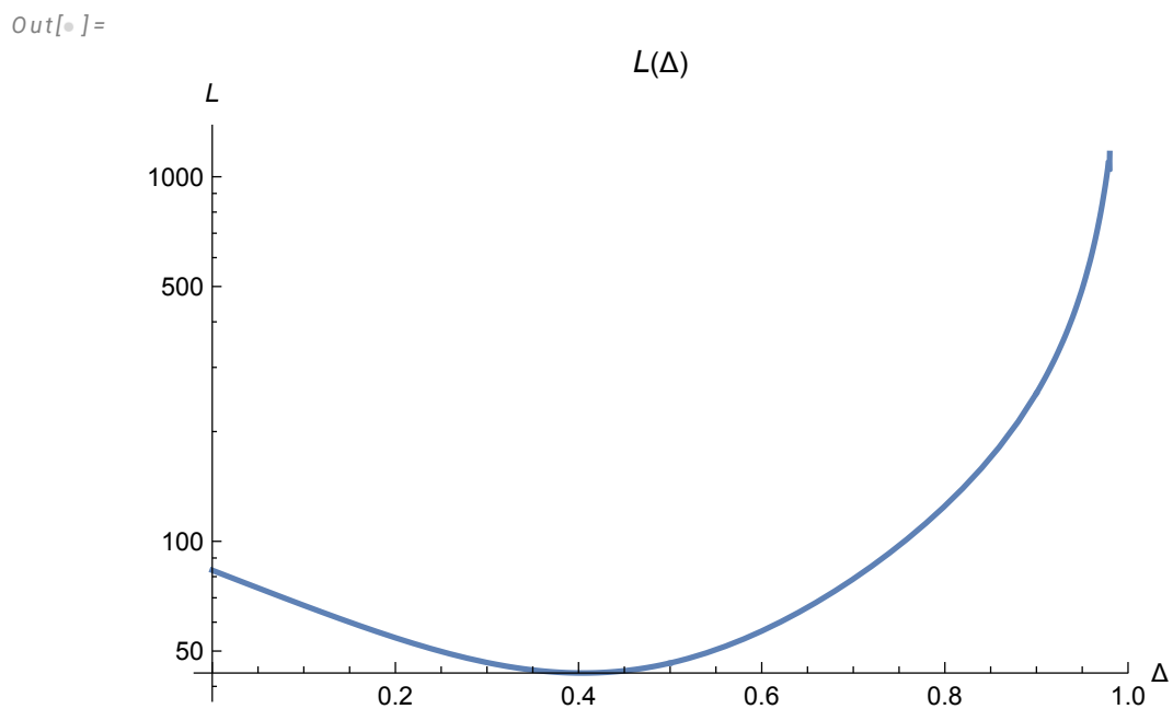
Figure 4. Log plot of L(\Delta) = A_c(r_0(\Delta), \Delta) .
