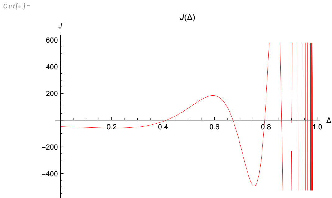
Figure 6. Plot of universal function J(\Delta) . There are no singularities inside the physical region 0 < \Delta < 1 , but there are zeros, condensing at \Delta = 1 .
