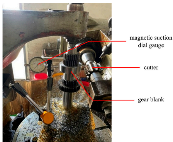
Figure 15. The diagram of the gear blank after clamping.
