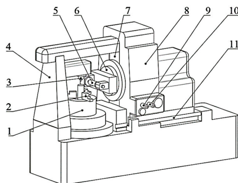
Figure 9. The structure schematic diagram of the Y-38 gear hobbing machine. 1-rotary workbench 2-loading fixture of the gear blank 3-live center 4-hobbing machine body; 5-cutter 6-cutter holder and its turntable; 7-radial rail 8-axial workbench; 9-axial feed handwheel shaft 10-radial feed handwheel shaft 11-axial rail.
