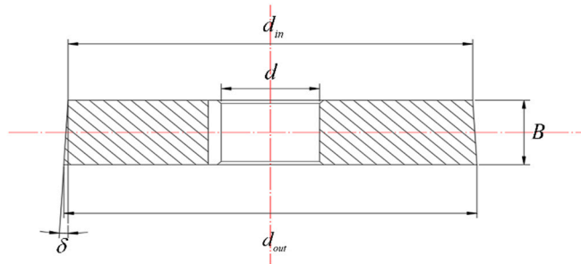
Figure 5. The structure of the gear blank.
