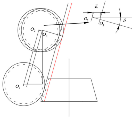
Figure 6. The schematic diagram of the cutter setting. E - the moving distance of the cutter after the cutter aligning. It can be calculated by Eq.16.
