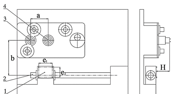
Figure 10. The schematic diagram of the installation position of the hanging wheel mechanism. 1-cover plate 2-axial lead screw rail 3-axial feed handwheel shaft 4-radial feed handwheel shaft; a-the distance between the two handwheel shafts; b-the height difference between the center of the cover plate and the axial feed handwheel shaft axis; e_1 and e_2 -the distance between the fixed bolt of the cover plate; H-the height difference between the cover plate transverse plane and the handwheel install plane.
