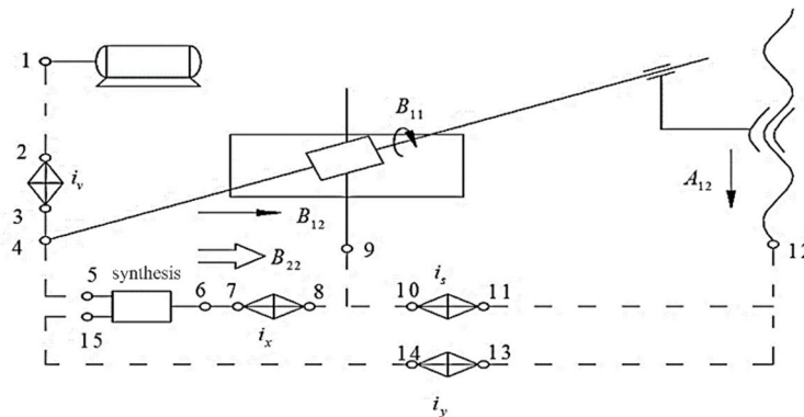
Figure 7. The transmission principle of helical cylindrical gears hobbing process.
