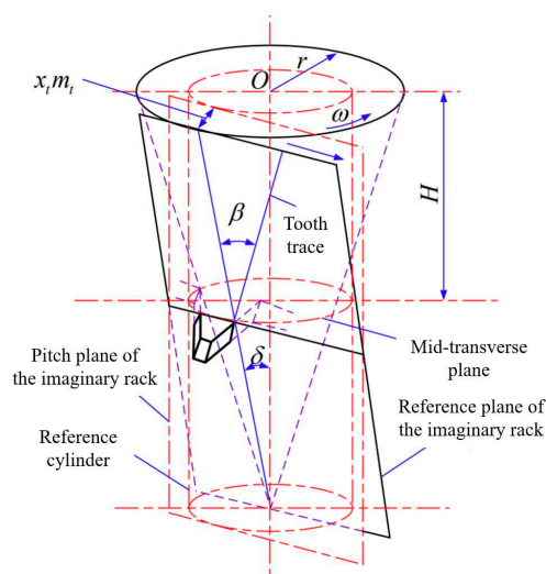
Figure 1. The schematic diagram of the helical beveloid gear's structure. H - the distance between the outer-transverse-plane and the mid-transverse-plane; \beta - the spiral angle, \delta - the taper angle; x_t m_t - addendum modification of the transverse plane; x_t - transvers modification coefficient; m_t -transverse module.
