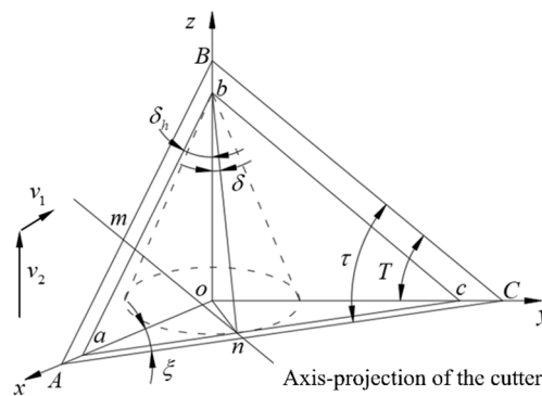
Figure 3. The relative position between the axis of the cutter and the gear blank. \tau - the inclination angle of the cutter axis in the plane ABC; \delta_h - the motion taper angle of the cutter
