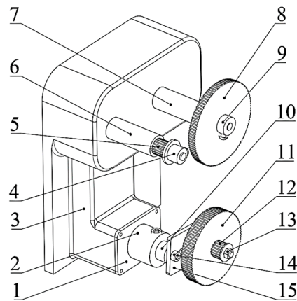
Figure 12. The three-dimensional assembly drawing of the hanging wheel mechanism. 1-cover plate 2-shaft seat 3-hobbing machine body 4-fix bolt of axial synchronous belt wheel; 5-axial synchronous belt wheel 6-axial rotary shaft 7-radial rotary shaft; 8-axial synchronous belt wheel 9-fix bolt of radial synchronous belt wheel 10-center rotary shaft 11-large center synchronous belt wheel 12-small center synchronous belt wheel; 13-fix bolt of the hanging wheel 14-connecting plate screws 15-connecting plate.
