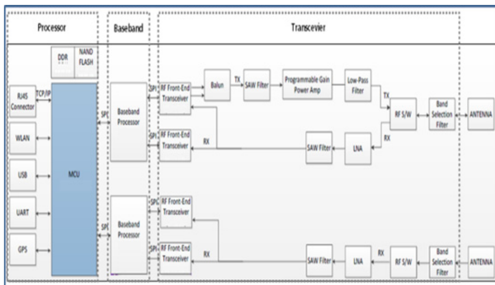
Figure 4. The hardware block diagram of gateway.
