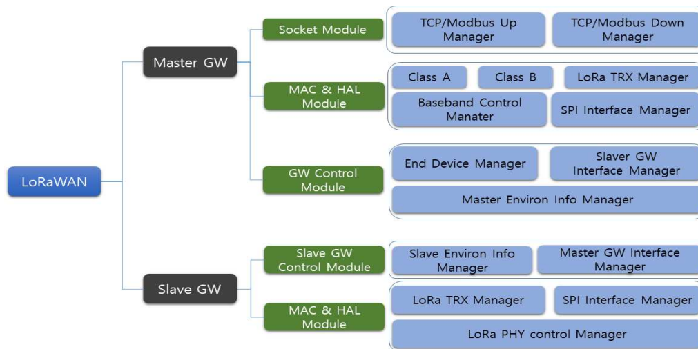
Figure 5. The function configuration diagram of gateway.
