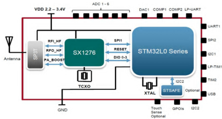
Figure 3. The hardware block diagram of sensor node.
