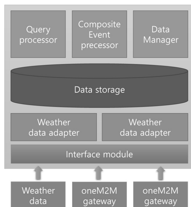
Figure 6. The structure diagram of bigdata analysis system.
