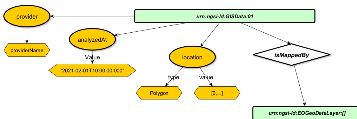
Figure 4. Visualisation of the GIS Data Model schema.
