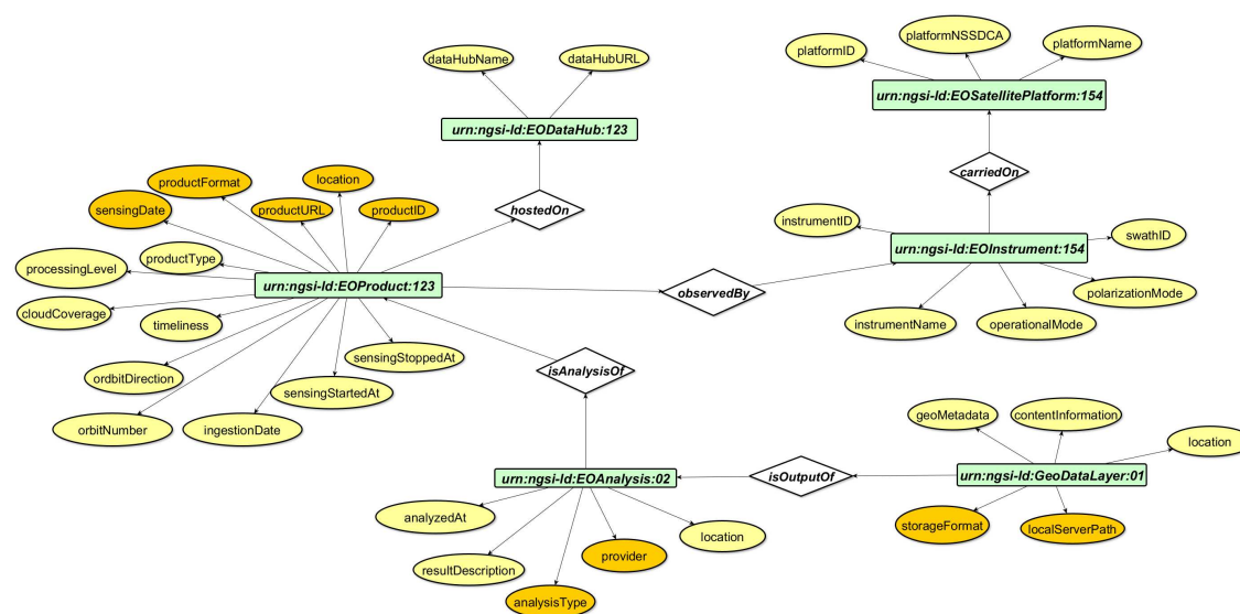
Figure 3. Visualisation of the Satellite Imagery Data Model schema.
