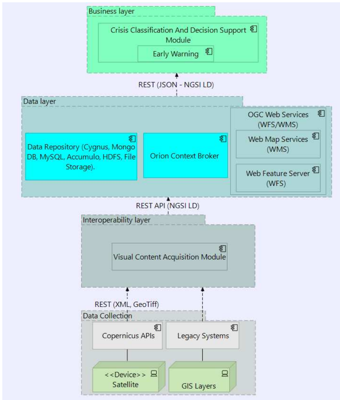
Figure 1. The logical architecture of the proposed framework.
