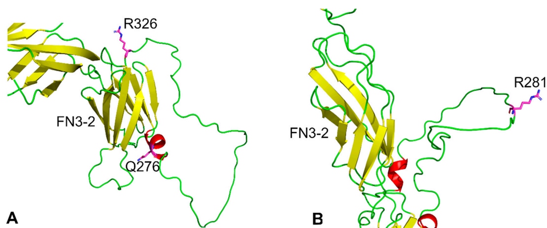
Figure 5. Location of missense SNPs in AlphaFold2 structures of CD148 and PTPRQ. (A) Structure of a section of the AlphaFold2 CD148 extracellular domain showing the position of the SNPs (Q276P and R326Q). Ribbons for other domains have been removed for clarity. (B) Structure of a section of the AlphaFold2 PTPRQ extracellular domain showing the position of the SNP (R281G).
