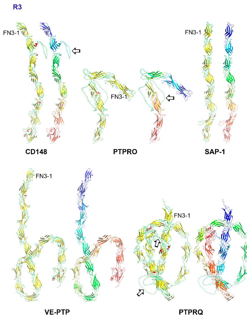
Figure 3. AlphaFold predicted structures for the extracellular domain of R3 subgroup PTPs. Colouring is by secondary structure (helix, red; sheet, yellow; loop, green) and by spectrum (N-terminus, blue; C-terminus, yellow/red). For clarity, sequence preceding FN3-1 and from the predicted transmembrane domain onwards is not shown. Unstructured loops are indicated by an arrow.
