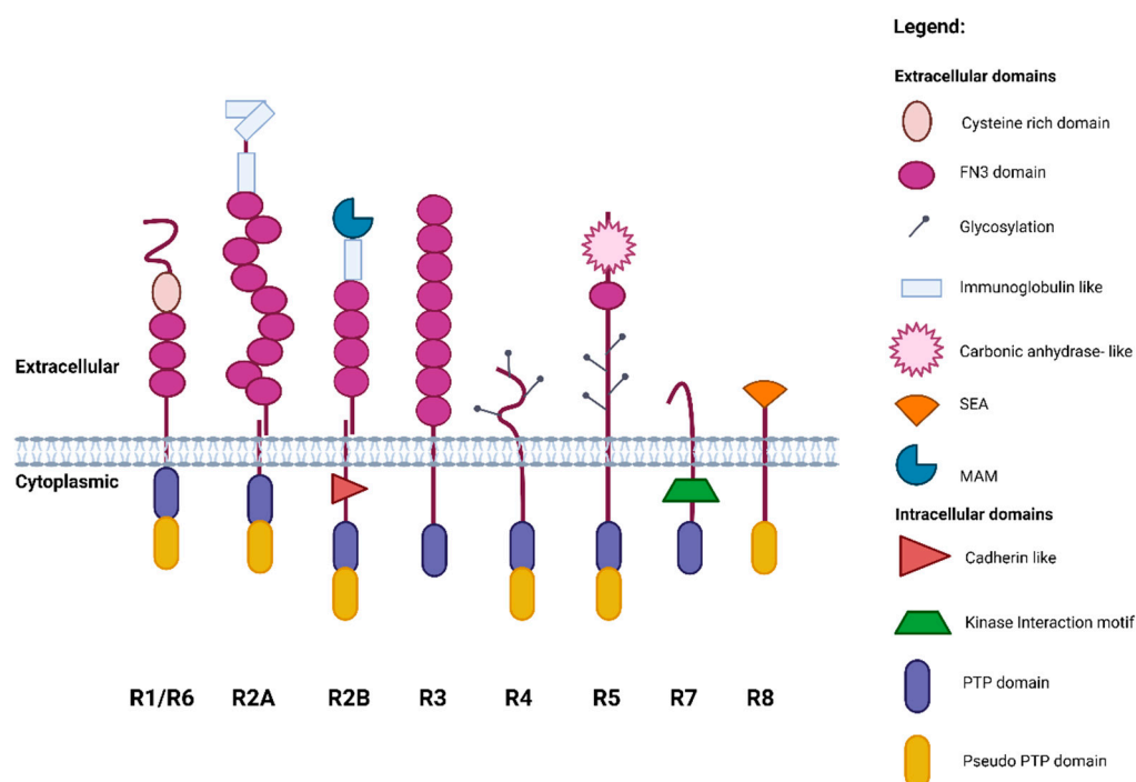
Figure 1. Schematic representation of the RPTP family. Created with BioRender.com.
