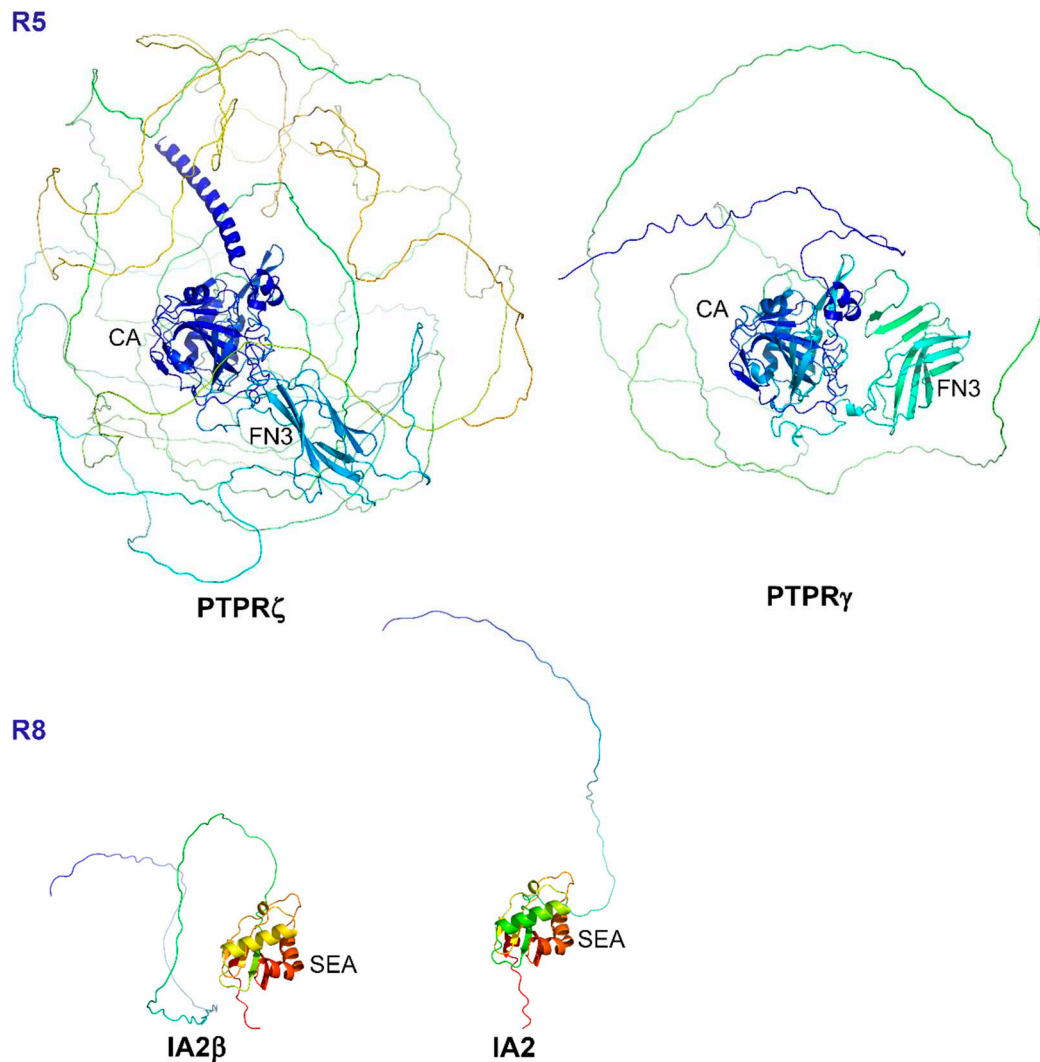
Figure 6. AlphaFold2 structures of the extracellular region of R5 and R8 subgroup PTPs. Structures are coloured by spectrum (N-terminus, blue; C-terminus, yellow/red). The structured carbonic anhydrase-like (CA) domain and single FN3-like (FN3) domain and long disordered spacer region are shown for the R5 group. SEA (sea urchin sperm protein, enterokinase, agrin) module.
