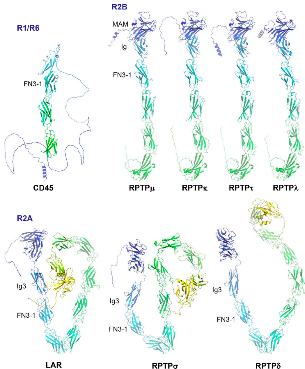
Figure 2. AlphaFold2 structural predictions of the extracellular domain for R1, R2A and R2B subgroup RPTPs. Structures are coloured by spectrum (N-terminus, blue; C-terminus, yellow).
