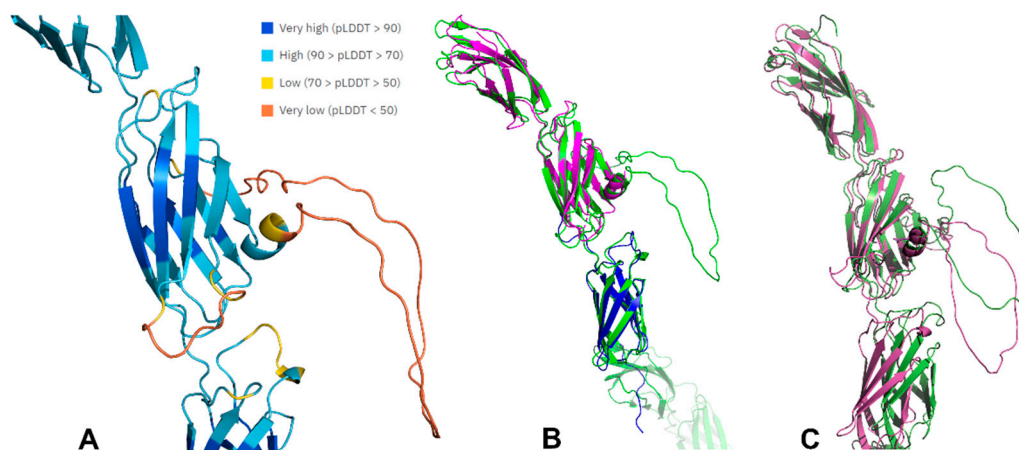
Figure 4. The unstructured loop of CD148 extracellular domain. (A) Part of the AF2 predicted extracellular domain CD148 structure coloured by pLDDT colours. (B) Superimposition of the AlphaFold predicted CD148 structure FN3-1 to FN3-3 (AF-Q12913-F1, green) with X-ray crystal structure of CD148 FN3 domains 1 & 2 (PDB: 7U08, magenta) and the NMR solution structure of FN3-4 of CD148 (PDB: 2DLE, blue). (C) Superimposition of a section of the CD148 AF2 structure and Colabfold structure generated without templates.
