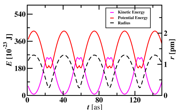
Figure 2. Energies of the electron and its radius variation with time in a Hydrogen atom. The radius of a Hydrogen atom is presented on the y-axis on the right.
