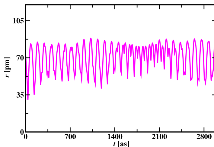
Figure 6. Change in Radius of the Carbon atom with time.
