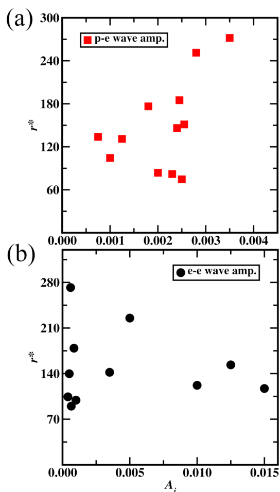
Figure 11. Radius of carbon atom variation with aether medium wave amplitude ( A_i ). (a) Proton and neutron aether medium wave amplitude, (b) electron aether medium wave amplitude.
