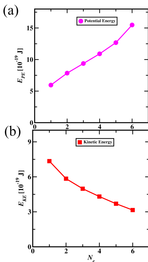
Figure 7. Potential (a) and Kinetic (b) energies of electrons in particle nature of Carbon atom. (On the x-axis, variable ( N_e ), the core electron numbered 1 and the valence electron numbered 6)
