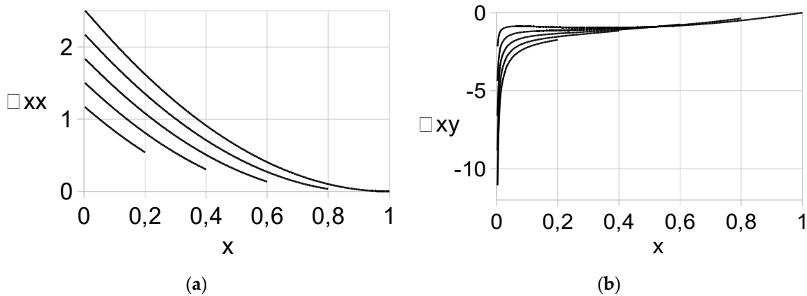
Figure 7. The components of the deformation rate matrix \mathfrak{R}_{xx} (graph a) and \mathfrak{R}_{xy} (graph b) at the entrance of a spherical heated spot vs the dimensionless coordinate x/a . The shock and gas conditions are the same as in the previous figure. In both graphs, the time sequence is from lower to upper curve and each curve corresponds to a dimensionless time starting at n\tau = 0.2 through equal intervals of \Delta n\tau = 0.2 .
