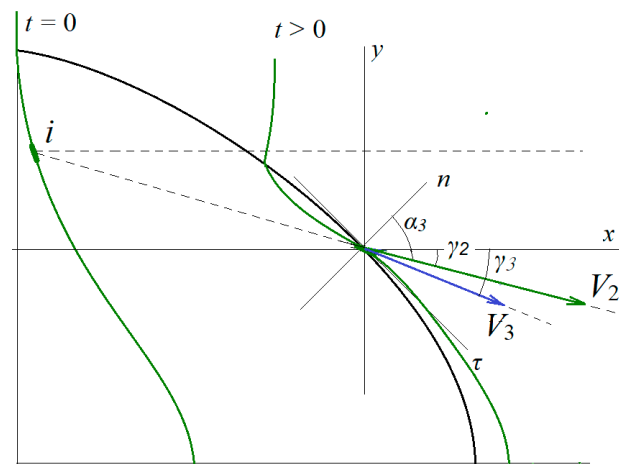
Figure 2. A shock front interacting with the back interface (black solid curve) during its partial exiting into the cooler surrounding. It starts from the initial position (left green) followed with further front distortion (right green).
