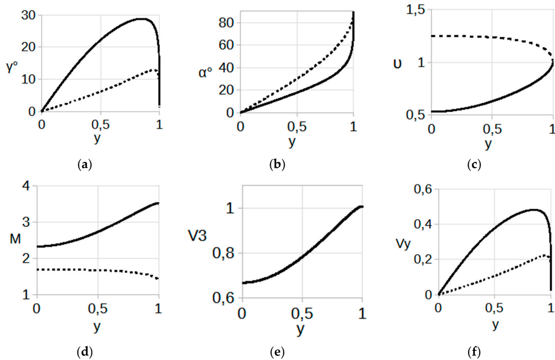
Figure 6. Shock parameter distribution along the interface (its dimensionless coordinate y ). (a) Refraction angles \gamma_2^\circ (dashed curve) and \gamma_3^\circ (solid). (b) Incidence angles \alpha_2^\circ (dashed) and \alpha_3^\circ (solid). (c) Shock velocity ratios, u_{21} (dashed) and u_{32} (solid). (d) Mach numbers M_2 (dashed) and M_3 (solid). (e) Shock velocity V_3 normalized to V_1 . (f) V_{2y} (dashed) and V_{3y} (solid) components of the shock velocities. Diatomic nitrogen gas at T_1 = 300\text{ K} , T_2 = 2000\text{ K} , M_1 = 3.5 .
