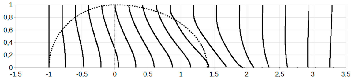
Figure 10. Front distortion as the shock crosses a drop-like shaped heated spot. The profiles correspond to several instances of dimensionless time through the equal intervals of \Delta n\tau = 0.2 (first 6 curves at the entrance), \Delta n_b = 0.15 (next 4 fronts at the exit), and \Delta n_b = 0.25 for those moving free behind the spot. The profile coordinates are normalized to b , and b/a_3 = 5/7 . Diatomic nitrogen at T_1 = 300 K, T_2 = 2000 K, M_1 = 3.5 .
