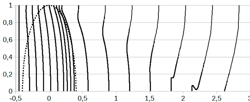
Figure 9. Shock front distortion as it crosses a hot spot of an elliptical cross section oriented transversely, followed by its recovery after emergence from the spot. The fronts entering the spot correspond to times starting at n_\tau = 0.2 through the equal intervals of \Delta n_\tau = 0.2 , for those exiting the spot \Delta n_b = 0.1 , and for the rest outside of the spot \Delta n_b = 1.0 . The profile coordinates are normalized to b , and b/a = 5/2 . Diatomic nitrogen at T_1 = 300\text{ K} , T_2 = 2000\text{ K} , M_1 = 3.5 .
