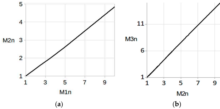
Figure 4. (a) The normal component of the Mach number M_{2n} vs M_{1n} , at the entrance part of the interface. (b) The component M_{3n} vs M_{2n} at the back interface. Diatomic nitrogen at T_1 = 300 K, T_2 = 2000 K, M_1 = 3.5 , p = p_{\text{atm}} .
