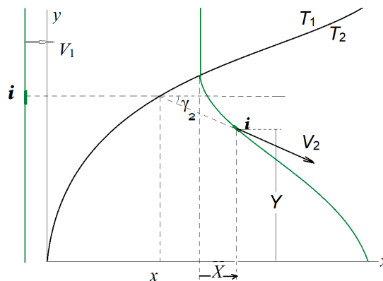
Figure 1. The initially planar shock wave (green vertical line) incident on the interface (black curve) with velocity V_1 , from left to right, undergoes a distortion (green curve) at a moment of time t_0 . Due to symmetry, only the upper half of the interaction picture is shown.
