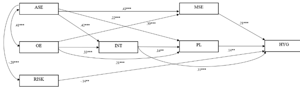
Figure 2. Structural equation modeling of the trimmed Health Action Process Approach. Note. HAPA variables: ASE=Action Self-Efficacy; OE=Outcome Expectancies, RISK=Risk Perception; INT=Intentions; MSE=Maintenance Self-Efficacy; PL=Planning; HYG=Hand Hygiene Behavior; N=279 ; Intention R^2=39.3\% ; Planning R^2=23.5\% ; Hand Hygiene R^2=33.2\% . The values reported represent the standardized estimates of each path in the model. Age, gender, depressive symptoms, and symptoms of generalized anxiety were included as covariates. Significant path at *** p<.001 , ** p<.01 , * p<.05 .
