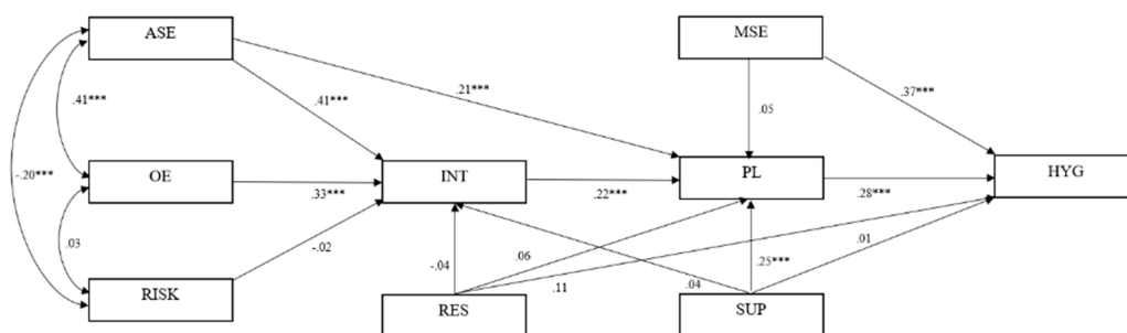
Figure 1. Structural equation modeling of the full Health Action Process Approach. Note. HAPA variables: ASE=Action Self-Efficacy; OE=Outcome Expectancies, RISK=Risk Perception; INT=Intentions; MSE=Maintenance Self-Efficacy; PL=Planning, RES=Resources, SUP=Social Support, HYG=Hand Hygiene Decisions; N=279 ; Intention R^2=39.5\% ; Planning R^2=19.8\% ; Hand Hygiene R^2=21.6\% . The values reported represent the standardized estimates of each path in the model. Significant path at *** p<.001 , ** p<.01 , * p<.05 .
