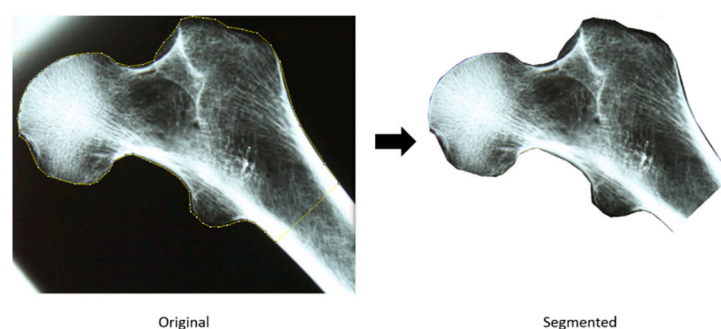
Figure 1. Feature extraction with Principal Components Analysis – a femora space and eigenfemora approach.
