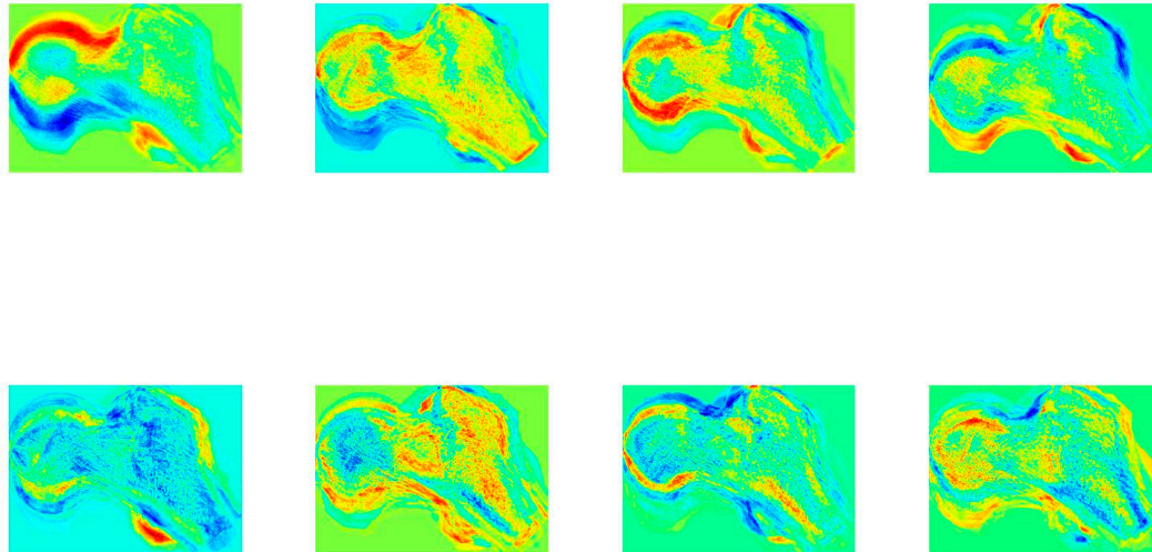
Figure 3. Jet color map representation of the first eight eigenfemora of the males' sample (ordered from top left to bottom right).
