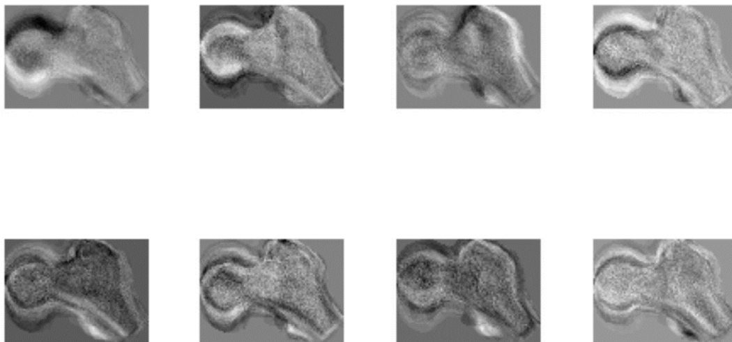
Figure 2. First eight eigenfemora of the females' sample (ordered from top left to bottom right).
